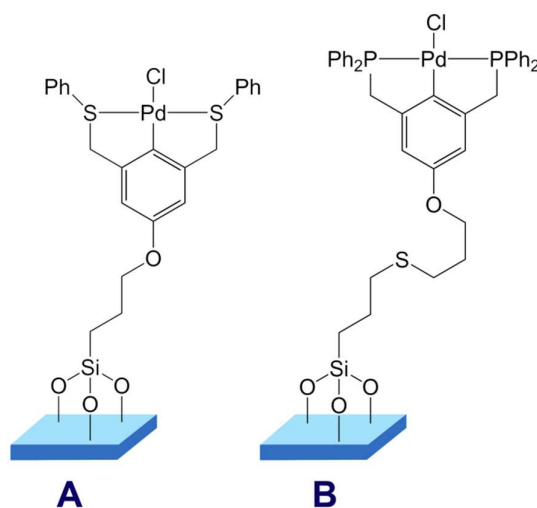
Figure 4. Examples of pincer complexes used for Pd anchoring.
