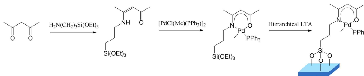
Scheme 6. Synthesis of zeolite-supported \beta -oxoiminatophosphinopalladium complex.
