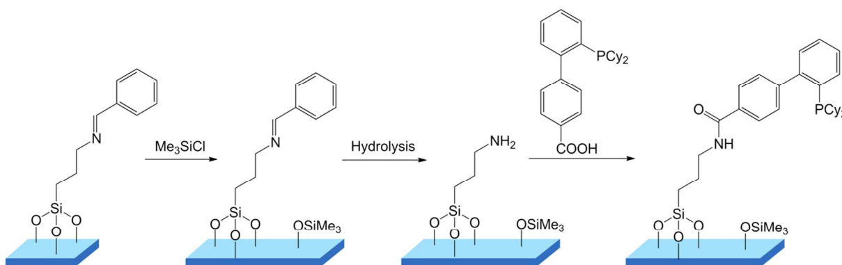
Scheme 5. Immobilization of a (dicyclohexyl)biphenyl moiety (Cy = cyclohexyl).
