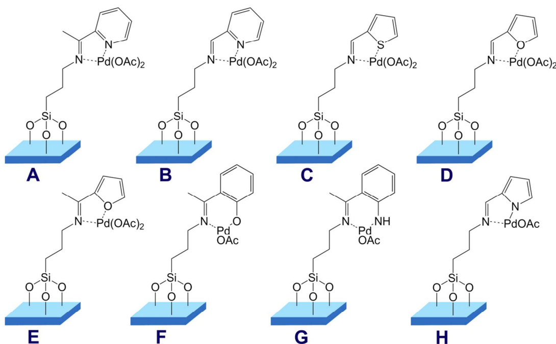
Figure 6. The set of silica supported palladium catalysts bearing N–N, N–S and N–O chelating ligands used in Suzuki-Miyaura coupling.
