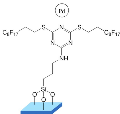
Figure 3. Supported Pd-catalyst containing perfluoroalkyl ligand used in Heck coupling reaction.
