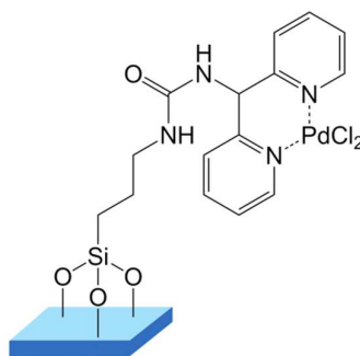
Figure 10. Bis(2-pyridyl)methane-Pd complex immobilised via an urea spacer.
