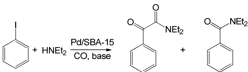
Scheme 13. Carbonylation of aryl iodide with secondary amine.
