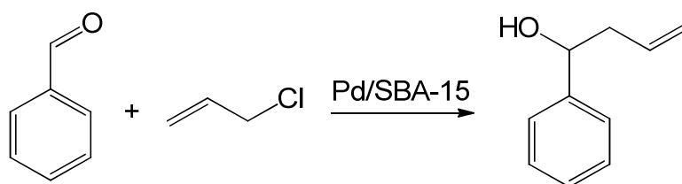
Scheme 31. Representative addition of allyl chloride to benzaldehyd.
