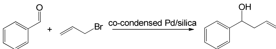
Scheme 36. Allylation of benzaldehyde with allyl bromide.
