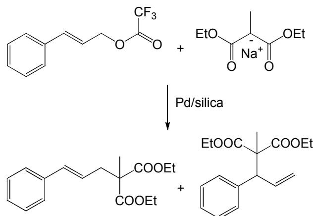
Scheme 42. Allylic substitution with diethyl 2-methylmalonate.
