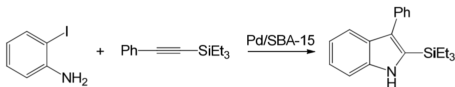
Scheme 41. Larock indole synthesis via heteroannulation.
