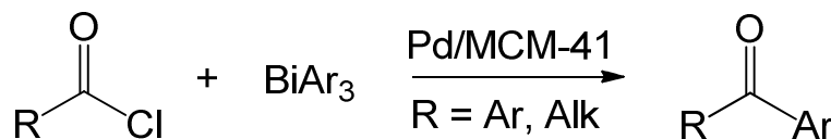
Scheme 34. Arylation of acyl chlorides with triarylbismuth derivatives.
