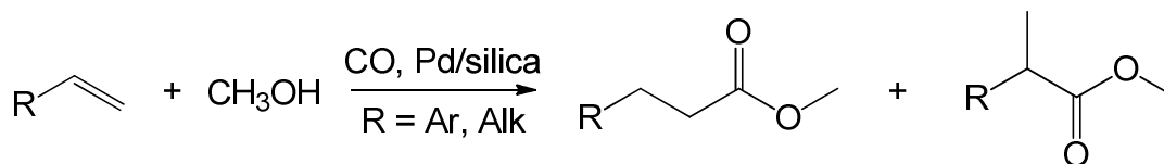
Scheme 35. Hydroesterification of alkenes with methanol affording methyl esters.
