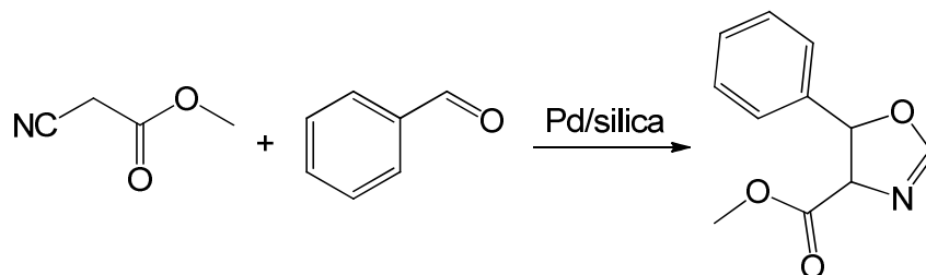
Scheme 44. Aldol reaction of methyl isocyanoacetate and benzaldehyde.
