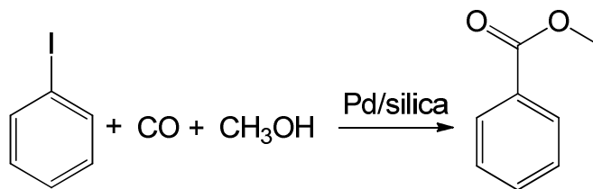
Scheme 12. Methoxycarbonylation of iodobenzene to methyl benzoate
