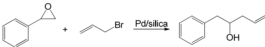
Scheme 37. Allylation of styrene oxide.
