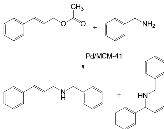
Scheme 43. Allylic amination of cinnamoyl acetate with benzylamine.
