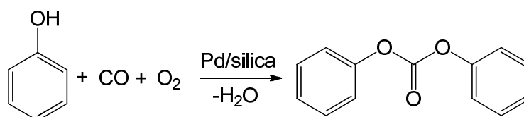
Scheme 9. Oxidative carbonylation of phenol.
