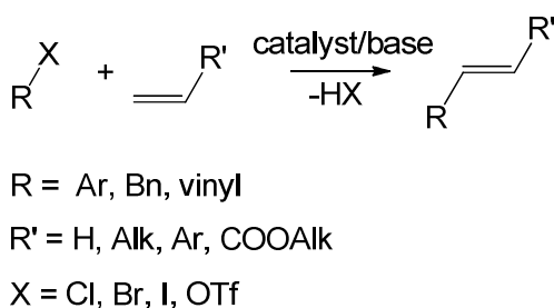
Scheme 2. The Heck coupling reaction.
