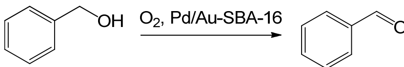
Scheme 17. Catalytic oxidation of benzyl alcohol to benzaldehyde
