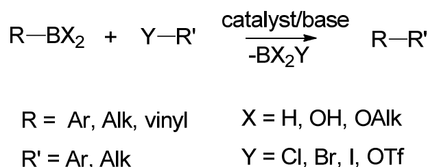
Scheme 3. Suzuki-Miyaura reaction.
