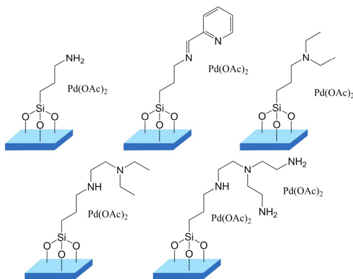
Figure 2. Supported Pd-catalysts comparatively evaluated in Heck coupling.
