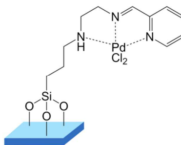
Figure 7. MCM-41-supported complex of a terdentate nitrogen ligand and Pd(II).
