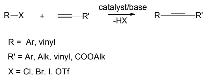
Scheme 7. Sonogashira coupling.
