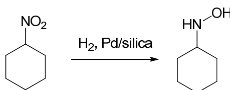
Scheme 23. Selective hydrogenation of 1-nitrohexane to N-hexyl hydroxylamine.
