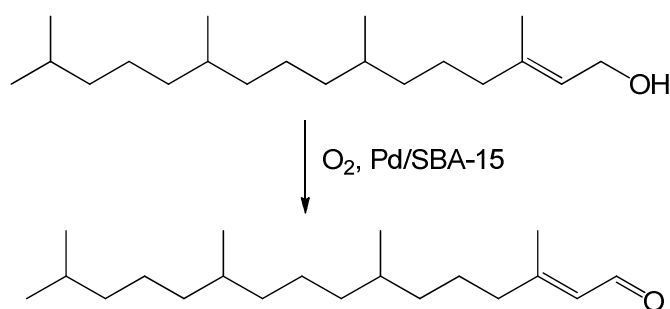
Scheme 19. Selective oxidation of phytol.
