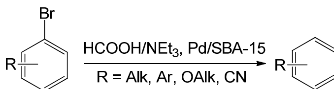
Scheme 30. Reductive dehalogenation of aryl bromide.
