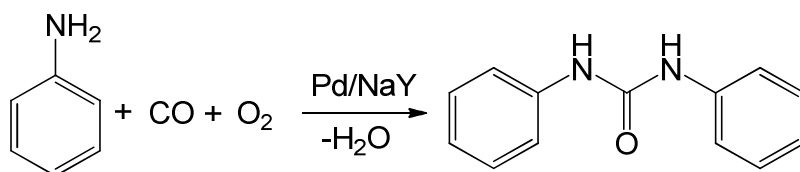
Scheme 10. Oxidative carbonylation of aniline to the corresponding N,N-disubstituted urea
