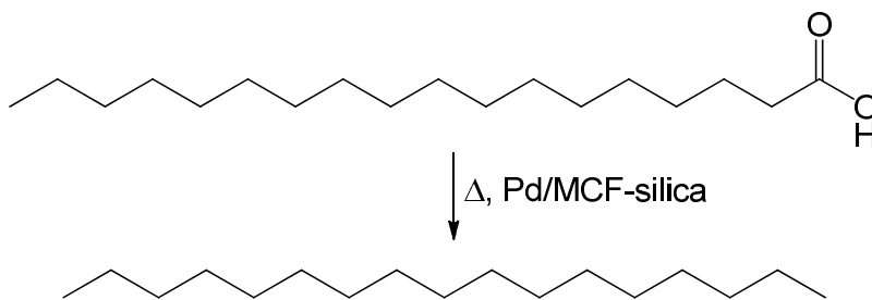
Scheme 40. Decarboxylation of stearic acid to n -heptadecane.
