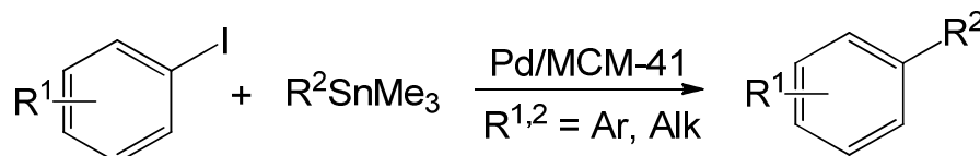
Scheme 39. Stille reaction of organostannanes with aryl halides.
