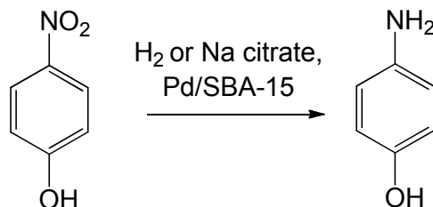
Scheme 21. Reduction of 4-nitrophenol into 4-aminophenol.
