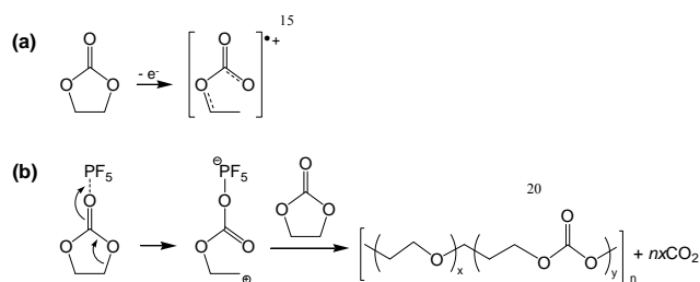
Fig. 11. Possible mechanism for the EC decomposition via strong Lewis acid, \text{PF}_5 . Reproduced with permission. 68
