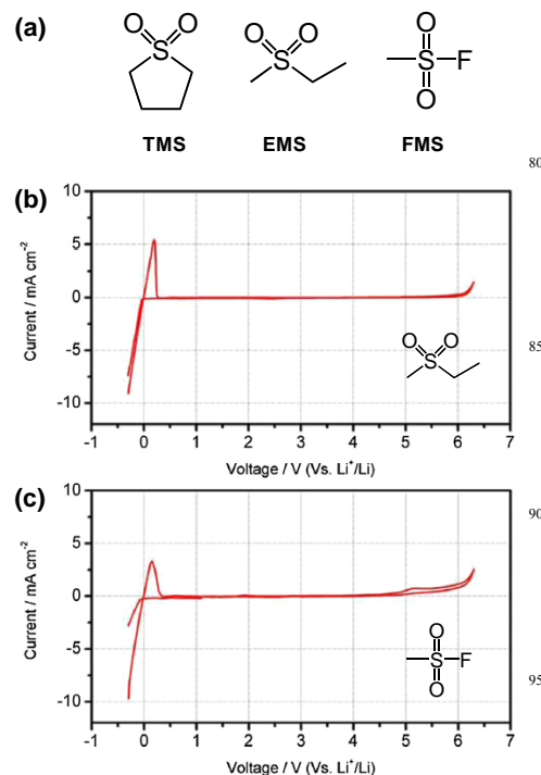
Fig. 14. (a) Structures of typical sulfone solvents. Cyclic voltammograms of 1 M \text{LiPF}_6 in (b) EMS/DMC (1:1 by wt.) and (c) EMS/FMS (1:1 by wt.). Scan rate: 5 mV s -1 . Pt as the working and counter electrodes and Li as the reference electrode. Reproduced with permission. 78
