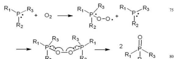
Fig. 27. Schematic representation for oxygen-absorbing reaction by phosphorus compound. Reproduced with permission. 117
