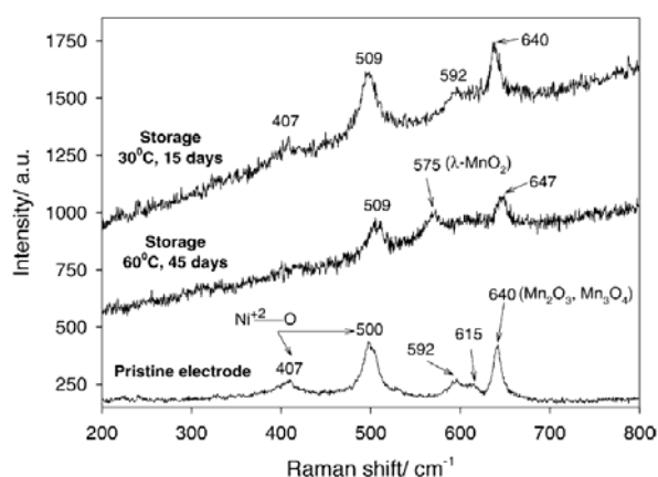
Fig. 10. ex-situ Raman spectra obtained from the pristine \text{LiNi}_{0.5}\text{Mn}_{1.5}\text{O}_4 , the electrode stored at 30 °C for 15 days, and the electrode stored at 60 °C for 45 days in EC/DMC (1/2)/1.5M \text{LiPF}_6 . Reproduced with permission. 69
