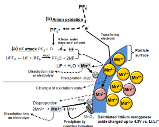
Fig. 3. Schematic presentation for the manganese dissolution out of a delithiated LMO cathode (a) by the HF attack, (b) by the PF 6 - anion oxidation. Reproduced with permission. 36
