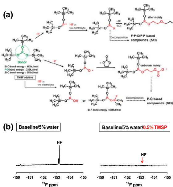
Fig. 19. (a) Proposed mechanisms for electrochemical oxidative decomposition of TMSP and for the unique function of TMSP scavenging HF from the electrolyte. (b) 19 F NMR spectra of the electrolyte with and without TMSP. Reproduced with permission. 92
