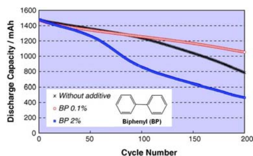
Fig. 6. Cycle life of LiCoO 2 /graphite cylindrical cells with and without BP additive cycled between 2.7 V and 4.3 V at 45 °C. Reproduced with permission. 26
