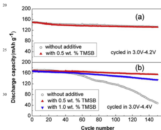
Fig. 8. Cycling performance of LiNi_{0.5}Co_{0.2}Mn_{0.3}O_2 /graphite cells cycled at a rate of 1 C in the voltage ranges of (a) 3.0-4.2 V and (b) 3.0-4.4 V. Reproduced with permission. 57
