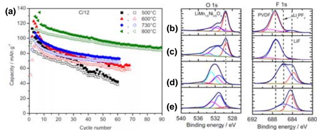
Fig. 12. (a) charge (filled symbols) and discharge (blank symbols) capacities of LNMO sintered at various temperatures. O 1s, F 1s, and P 2p XPS spectra of LNMO cathode sintered at 800 °C (b) before cycling, (c) after 1 cycle, (d) after 100 cycles, (e) LNMO cathode sintered at 500°C after 100 cycles. Reproduced with permission. 13
