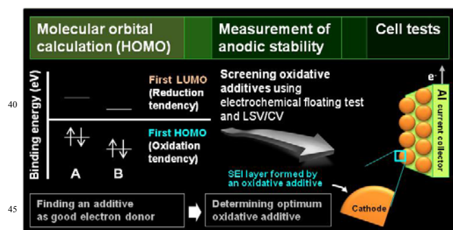
Fig. 2. Useful processes for discovering suitable oxidative additives for stabilizing the cathode-electrolyte interface. The optimum additive is identified via comparative studies of anodic stability of the electrolytes with various oxidative additives; such studies, involve measuring the
