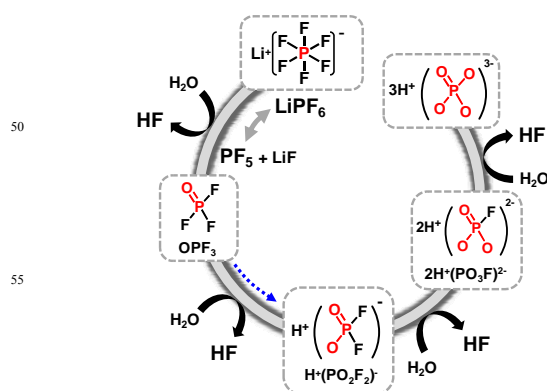
Fig. 18. Hydrolysis reactions of LiPF 6 salt in the presence of trace water in the cell.
