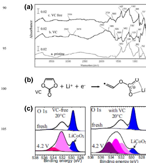
Fig. 4. (a) FTIR spectra obtained from the LMO cathodes before and after being cycled in the VC-free and VC-added electrolytes. (b) Possible mechanism of the VC decomposition. The polymerization of VC may occur by the radical species. (c) O 1s XPS spectra of the LCO cathodes before and after being cycled in the VC-free and VC-added electrolytes. Reproduced with permission. 4,53
