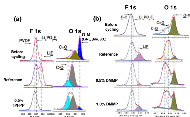
Fig. 21. F 1s and O 1s XPS spectra of (a) LiNi 0.5 Mn 1.5 O 4 electrode before and after cycled in reference and TPFPP-added electrolyte. (The cycled cathodes were obtained from the Li/LNMO half cells after 55 cycles.) and (b) LiNi 0.5 Mn 1.5 O 4 electrode before and after cycled with reference and DMMP-added electrolyte. (The cycled cathodes were obtained from the Li/LNMO half cells after 50 cycles.) Reproduced with permission. 98,99
