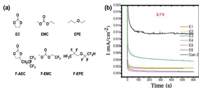
Fig. 13. (a) Chemical structure of the baseline carbonate (EC and EMC), ethyl propylether (EPE), fluorinated cyclic carbonate (F-AEC), fluorinated linear carbonate (F-EMC), and fluorinated ether (F-EPE), (b) Electrochemical stability of Gen 2 and fluorinated electrolytes E1 to E6 at 5.7 V using a 3-electrode electrochemical cell (Pt/Li/Li). Gen 2: 1.2 M \text{LiPF}_6 EC/EMC (3/7), E1: 1.2 M \text{LiPF}_6 in EC/EMC/F-EPE (2/6/2), E2: 1.2 M \text{LiPF}_6 in EC/EMC/F-EPE (2/5/3), E3: 1.2 M \text{LiPF}_6 in F-AEC/EMC/F-EPE (2/6/2), E4: 1.2 M \text{LiPF}_6 in F-AEC/EC/EMC/F-EPE (1/1/6/2), E5: 1.2 M \text{LiPF}_6 in F-AEC/F-EMC/F-EPE (2/6/2), E6: 1.2 M \text{LiPF}_6 in EC/F-EMC/F-EPE (2/6/2). Reproduced with permission. 18
