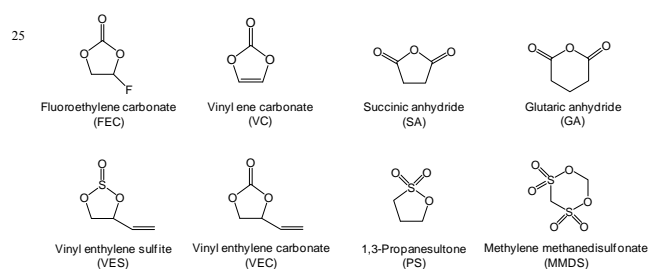
Fig. 1. Chemical structures of various organic-based additives.
