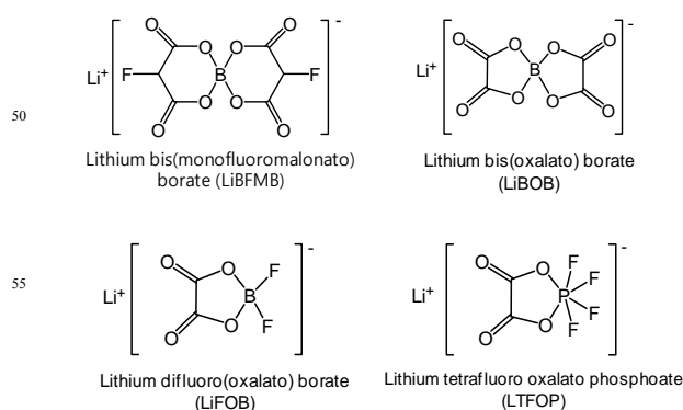
Fig. 9. Chemical structures of salt-type additives.
