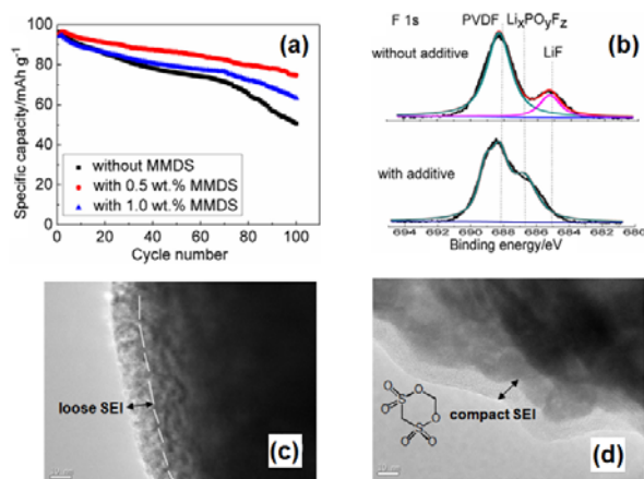
Fig. 5. (a) Discharge capacity retention of LMO/graphite full cell at 60 °C. (b) F 1s XPS spectra of LMO cathodes after 100 cycles at 60 °C. TEM images of LMO cathode surface cycled in (c) the additive-free electrolyte, (d) the MMDS-added electrolyte. Reproduced with permission. 56
