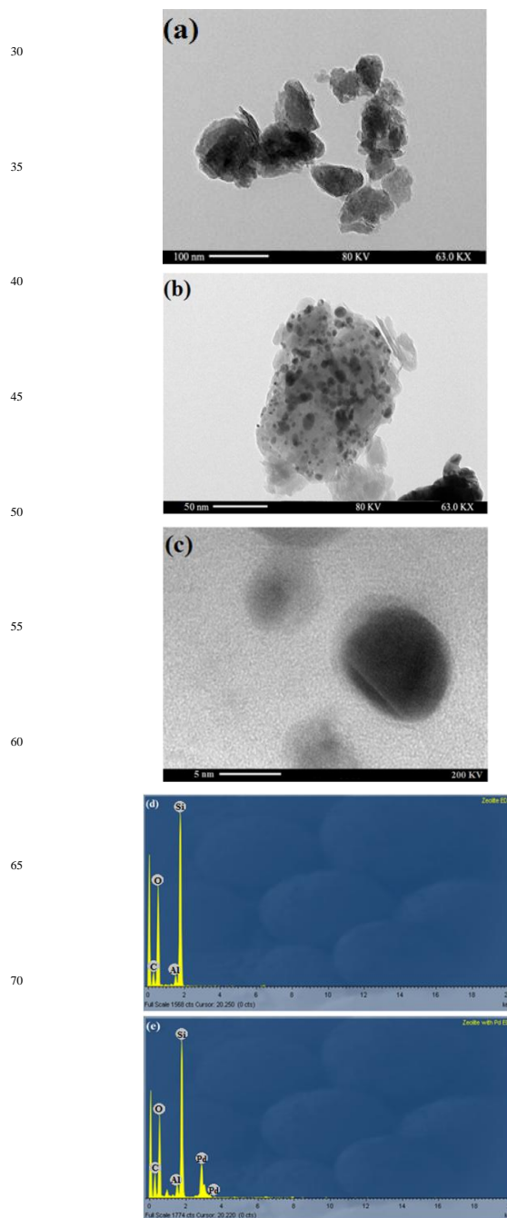
Fig 4. TEM images of (a) AT- Nano CP and (b) AT-Nano CP-Pd 0 . (c) HRTEM image of AT-Nano CP-Pd 0 . TEM-EDS data of (d) AT-Nano CP and (e) AT-Nano CP-Pd 0 .
