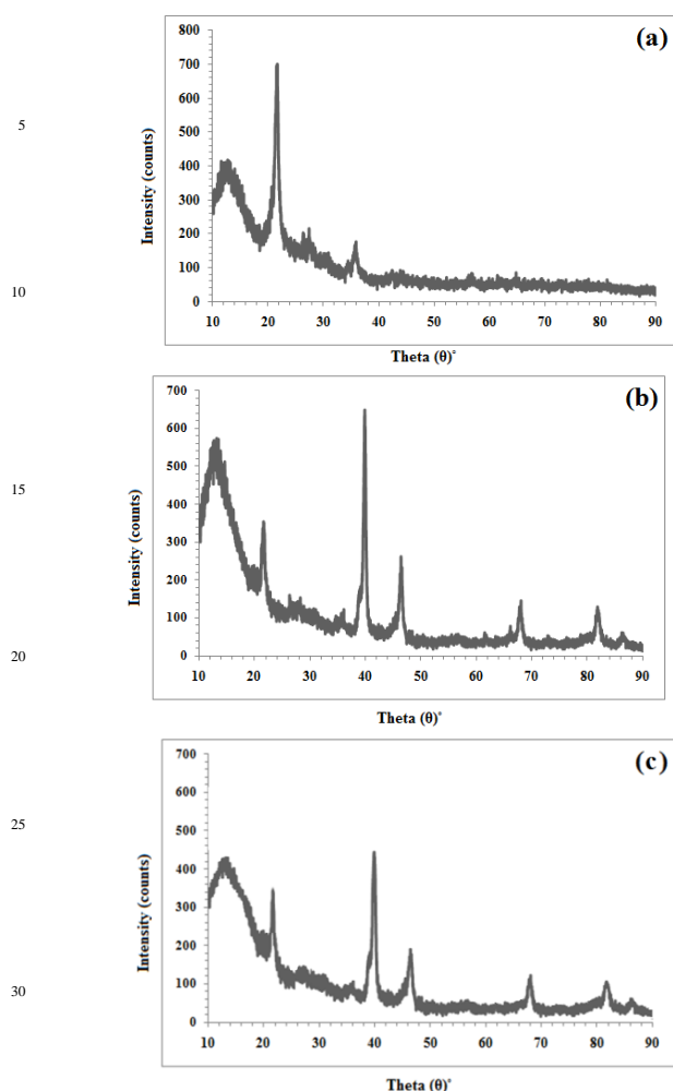
Fig 2. XRD patterns of (a) AT-Nano CP, (b) AT-Nano CP-Pd 0 and (c) AT-Nano CP-Pd 0 recovered after 8rd cycles
