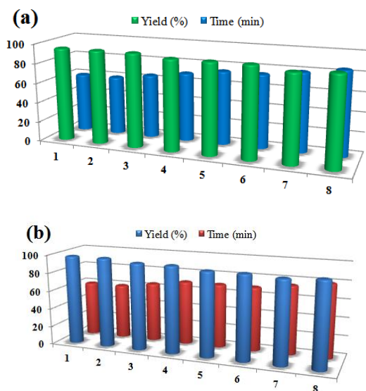
Fig. 6. Recyclability of the catalyst in (a) Sonogashira coupling reaction; Reaction conditions: Iodobenzene (1 mmol), phenylacetylene (1 mmol), water (5 ml), K_2CO_3 (1.5 mmol) and the catalyst (3 mg, containing 6 \times 10^{-4} mmol, 6.3 \times 10^{-5} g of Pd), 60 °C. (b) Ullmann coupling reaction; Reaction conditions: Iodobenzene (1 mmol), phenol (1 mmol), water (5 ml), K_2CO_3 (1.5 mmol) and the catalyst (3 mg, containing 6 \times 10^{-4} mmol, 6.3 \times 10^{-5} g of Pd), 60 °C.
