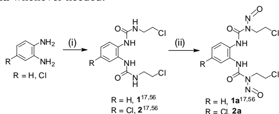
Scheme 2 Representative scheme for synthesis of nitrosoureas ( 1a , 2a ) (where 1 , 2 and 1a were synthesized according to literature procedure 17, 56 ). (i) 2-chloroethyl isocyanate (2 equiv.), DCM/THF, 0°C, 0°C to RT, 6h (ii) NaNO_2-HCO_2H , 0°C-5°C, 4h
