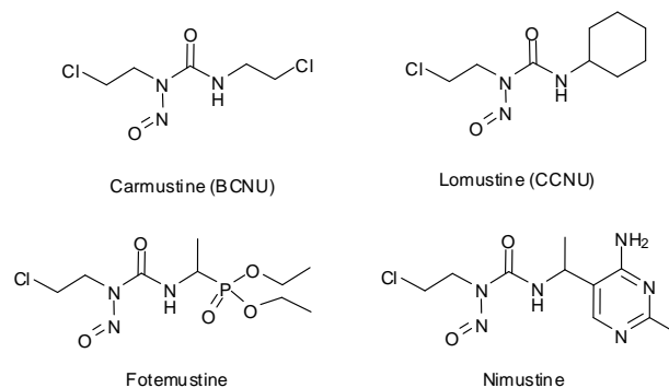
Scheme 1. Different nitrosoureas as chemotherapeutic agents.
