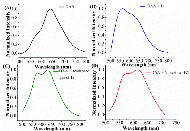
Fig. 5 (A) DAA (50 \mu M in DMSO): normalized emission spectrum, \lambda_{\text{ex}} = 490 nm. (B) DAA (50 \mu M in DMSO) + 1a (50 \mu M in DMSO): normalized emission spectrum, \lambda_{\text{ex}} = 490 nm. (C) DAA (50 \mu M in DMSO) + Headspace gas of 1a (20 mL): normalized emission spectrum, \lambda_{\text{ex}} = 490 nm. (D) DAA (50 \mu M in DMSO) + nimustine.HCl (50 \mu M in DMSO): normalized emission spectrum, \lambda_{\text{ex}} = 490 nm
