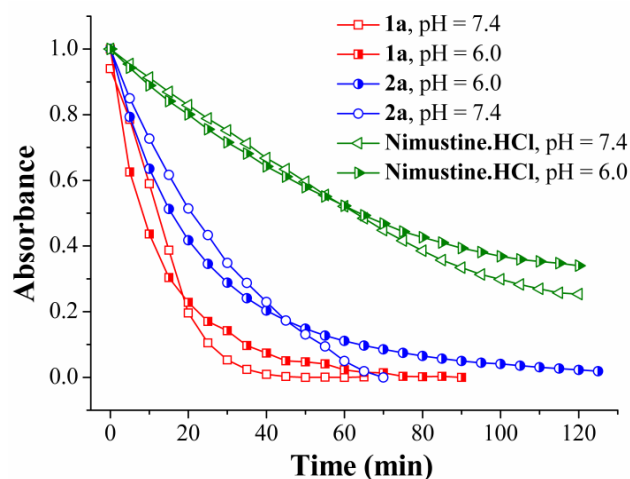
Fig. 2 Decrease in absorbance (normalised) vs. time plot for aqueous stability of compounds 1a , 2a and nimustine.HCl in phosphate buffer (10 mM) of pH 7.4 and 6.0. The decrease in absorbance at \lambda = 236 nm for 1a , 242 nm for 2a , and 232 for nimustine.HCl with time has been monitored and plotted.
