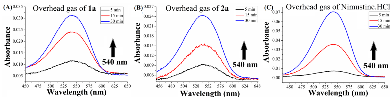
Figure 4. Change in absorbance vs. wavelength ( \lambda_{\max} = 540 nm) when headspace gas from (A) 1a and (B) 2a and (C) nimustine.HCl giving positive Griess Reagent test.
