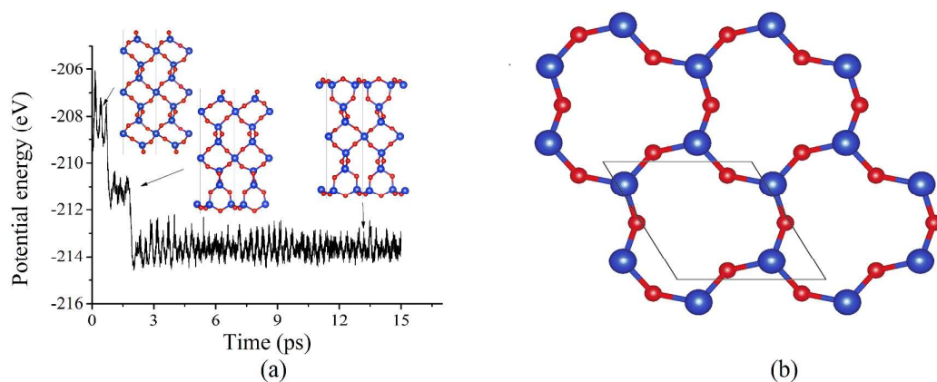
Fig. 1 (a) Evolution of potential energy of cleaved \alpha -SiO 2 (001) surface at 600 K. (b) Top view on reconstructed \alpha -SiO 2 (001) surface generated from BOMD simulation of a unit cell. Here and for all other figures, red and blue circles are oxygen and silicon atoms, respectively.
