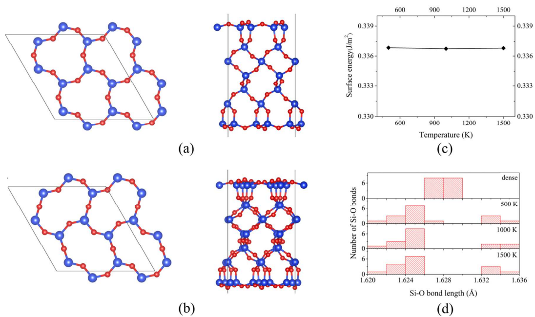
Fig. 2 Top and lateral views on (a) prereconstructed (“dense” surface) 27-layer supercell slab and (b) 2×2 reoptimized “dense” slab. (c) Surface energy of 2×2 reoptimized “dense” 27-layer supercell slab as a function of annealing temperature. (d) Bond length distributions for the central layer of 27-layer supercell slab for “dense” and 2×2 reoptimized “dense” surfaces at different temperatures (500, 1000, and 1500 K).
