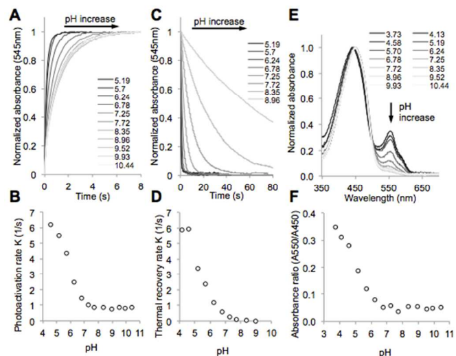
Fig. 3. pH dependence of shyRFP. A and B, photoactivation traces and rates at different pH values. C and D, thermal recovery traces and rates at different pH values. E and F, normalized absorbance spectra and absorbance ratio (550 nm/450 nm) in the yellow state under various pH values.
