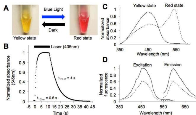
Fig. 1. Photochromic properties of shyRFP. A, visible colour appearance of purified protein in the yellow and red states. B, absorbance (545 nm) change upon violet light (405 nm) activation and dark conversion (22 °C, pH=7.5). Bar above the curve indicates the time when laser illumination is on. C, photochromic absorbance spectrum change. D, photochromic fluorescence spectrum change (yellow state, solid line; red state, dashed line). Note that the 545 nm absorbing species is not apparent in the red state excitation spectrum.
