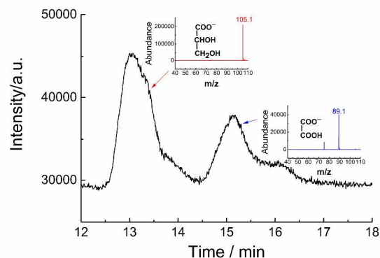
Fig. 5. Representative mass spectra of the main molecules resulting from the glycerol oxidation performed at 0.8 V vs. RHE on PdMn/C electrocatalyst.
