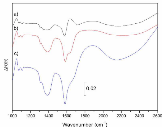
Fig. 7. FTIR spectra of the species recorded after 30 minutes of chronoamperometry measurements performed at 0.8 \text{ V vs. RHE} on Pd/C (a), PdFe (b) and PdMn (c) electrocatalysts in 0.1 \text{ M NaOH} containing 0.1 \text{ M} glycerol.
