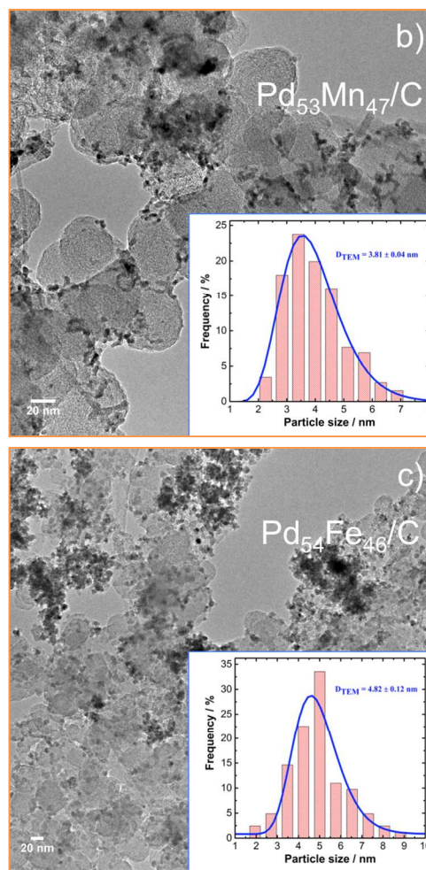
Fig. 2. TEM images of the PdM/C (M = Mn and Fe) nanomaterials prepared by the MW method. The insets represent the histograms of the particle size distribution.
