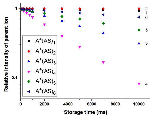
Figure 4. Relative intensity of the parent ions A^+(AS)_n (with n = 1-6 ) for different ion-trap storage times. Cluster size n is also indicated next to the data series for clarity. Note the semi-logarithmic scale.
