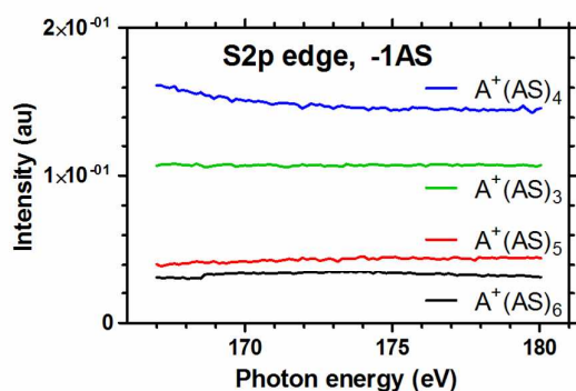
Figure 5. Relative intensity of the fragmentation peaks corresponding to loss of a single AS unit loss from the clusters A^+(AS)_6 , A^+(AS)_5 , A^+(AS)_4 and A^+(AS)_3 in the energy region of the S2p absorption edge.
