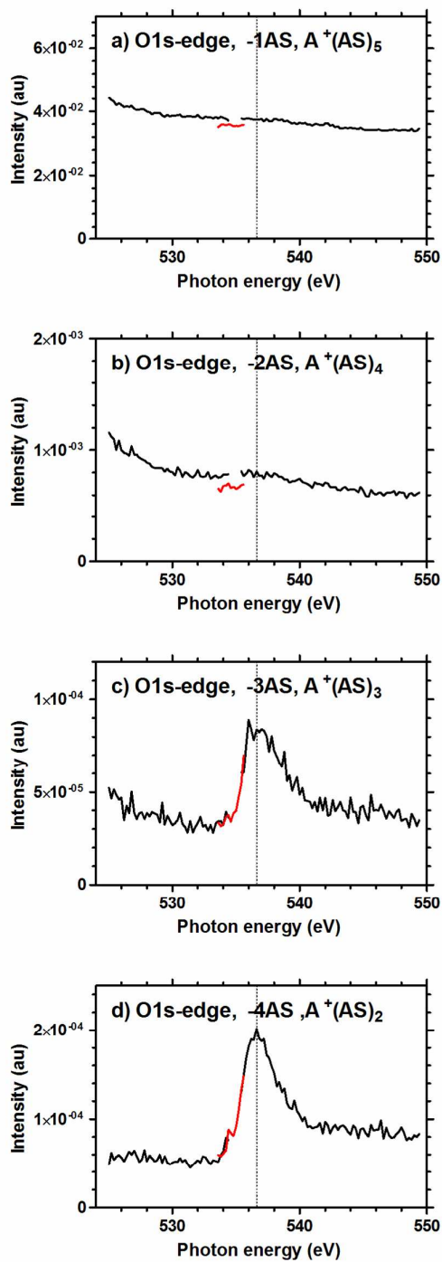
Figure 1. Relative intensity of fragmentation peaks corresponding to the loss of 1 AS unit (panel a), 2 AS units (panel b), 3 AS units (panel c) and 4 AS units (panel d) from the A + (AS) 6 cluster ion in the energy region of the oxygen-1s absorption edge. Original measurement in black (data points lost for 534.2–535.4 eV); completing measurement in red. The vertical dotted line is included to guide the eye.
