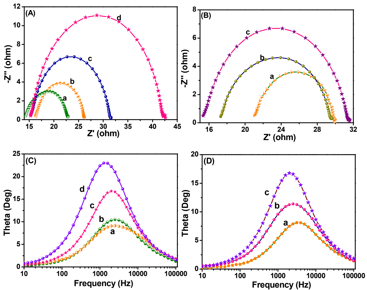
Fig. 7. (A) Nyquist plot and (C) Bode phase plots obtained for N-TiO 2 -Ag nanocomposite-modified photoanodes with (a) 2.5, (b) 5, (c) 10, and (d) 20 wt% of Ag content. (B) Nyquist plot and (D) Bode phase plots of (a) TiO 2 , (b) N-TiO 2 , and (c) N-TiO 2 -Ag (10 wt% Ag).
