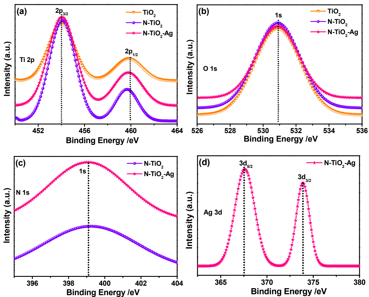
Fig. 2. XPS spectra of TiO 2 , N-TiO 2 , and N-TiO 2 -Ag (10 wt.% Ag) and their corresponding (a) Ti 2p (b) O 1s (c) N 1s, and (d) Ag 3d core-level spectra.
