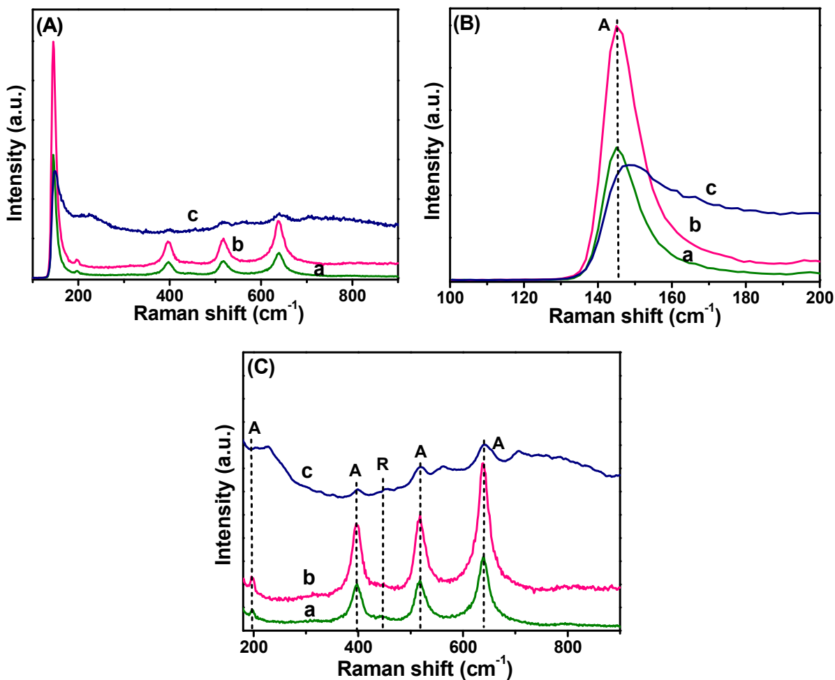
Fig. 3. Raman spectra of (a) TiO 2 , (b) N-TiO 2 , and (c) N-TiO 2 -Ag (10 wt.% Ag) in different frequency regions: (A) 100–900 cm -1 , (B) 100–200 cm -1 , and (C) 180–900 cm -1 , which are provided separately for better clarity of the anatase and rutile phase TiO 2 .
