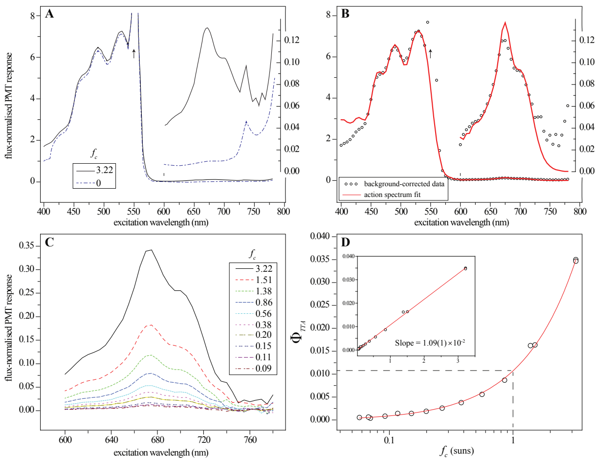
Figure 4: Action spectrum results for the PQ 4 PdNA:Rubrene system (detector monochromator set to 555 nm with a bandpass of approximately 5 nm). (A) Full action spectra for maximum and zero bias intensity, corresponding to concentration factors of 3.2 and zero, respectively. The arrow shows the location of the scatter peak, which was ignored during fitting. The inset shows the upconversion region scaled by 52 times on the same abscissa as the main plot; (B) Fit of Eq. 6 to the background-corrected full-bias spectrum, with the upconversion region similarly zoomed; (C) The upconversion region measured at higher sensitivity for a range of concentration factors; (D) \Phi_{TTA} values, extracted from the fit of Eq. 6, plotted with respect to concentration factor.
