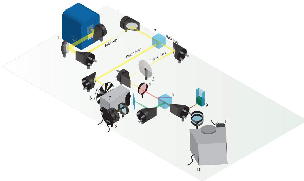
Figure 1: Action spectrum experimental setup. The output of a laser-driven xenon arc lamp (1) is collimated, the beam diameter is halved in Telescope 1, then the beam is divided in a polarising beam splitter cube (2). The transmitted beam (bias) enters Telescope 2, again halving the beam diameter, then passes through a variable neutral density filter (3) and chromatic filter (4) before re-entering a second identical beam splitter (5). Meanwhile, the reflected probe beam is modulated by a chopper wheel (6), then imaged into a monochromator (7). A reference silicon photodiode (8) monitors lamp stability. The probe beam is re-combined with the bias in (5), then focused into the UC sample (9). Photoluminescence from the sample is collimated, then imaged into a second monochromator (10), with a PMT mounted on the output (11). During calibration measurements the reference photodiode is moved to the sample position.
