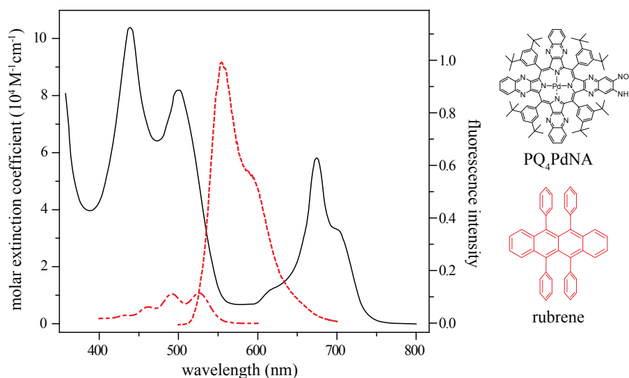
Figure 3: The structures and spectra of PQ 4 PdNA (extinction, in black solid line) and rubrene (extinction and emission, red dot-dashed and red dashed lines, respectively), the sensitizer and emitter employed in the reported TTA-UC system.
