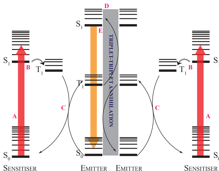
Figure 2: Energy level diagram of the TTA-UC process. Two sensitiser absorb uncorrelated low-energy photons (A) and intersystem-cross to the first triplet state (B). Triplet energy transfer via Dexter exchange produces two triplet-excited emitters (C). Subsequent collisions between such emitters leads to TTA, which can yield one singlet-excited emitter (D). Fluorescence from this state (E) constitutes generation of an upconverted photon.
