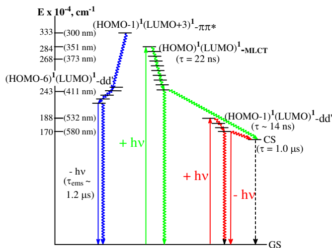
Scheme II. Simplified energy diagram showing the photophysical processes of [\text{Ni}(\text{tmdbzTAA-CO...})] when they are excited with 580, 532 and 351 nm light. A dashed arrow and wavy arrows represent respectively the back electron transfer decay of CS reforming the ground state and radiationless relaxations of excited states
