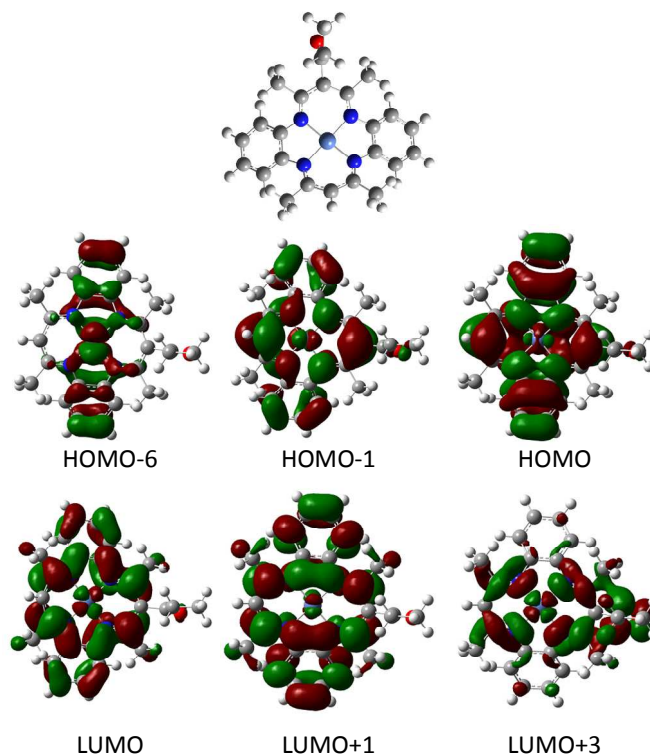
Figure 2. Molecular orbitals involved in the UV-Vis electronic transitions. The optimized structure of the model compound used in the TDDFT calculations is shown at the top of the figure.
