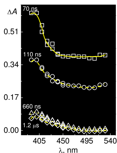
Figure 4. Transient spectra recorded when a deaerated solution of poly( \text{Ni}^{\text{II}}[\text{tmdbzTAA}]_2 ) buffered at pH = 8 and containing 0.1 M tEA was irradiated at 351 nm.
