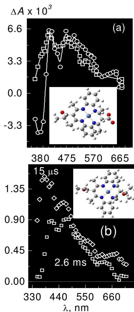
Figure 8. Spectra recorded in pulse radiolysis when poly(Ni II [tmdbzTAA]) 2 was reduced: (a), by CO 2 •- (○) and (CH 3 ) 2 C • OH (□) and (b), by the combined actions of e - aq and (CH 3 ) 2 C • OH. An Inset to (a) and (b) are respectively the optimized structures of the eq. 2 and eq. 3 products. Delays from the radiolytic pulse used recording the spectra are: (○) 500 μs, (□) 300 μs in (a) and (○) 15 μs, (□) 2.6 ms in (b). Other experimental details are given in the text.
