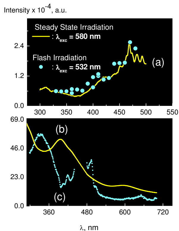
Figure 9. Luminescence of \text{poly}(\text{Ni}^{\text{II}}[\text{tmdbzTAA}]_2) in deaerated solutions buffered at pH 8. The emission spectrum, recorded in the steady state irradiation of the solution at \lambda_{\text{exc}} = 580 nm (a, solid line) has been superimposed with the emission spectrum (a, circles) recorded 5 \mu\text{s} after the flash irradiation of the solution at \lambda_{\text{exc}} = 532 nm. The excitation spectrum (b) was recorded monitoring the emission at 460 nm. It is superimposed with the absorption spectrum of the solution (c).
