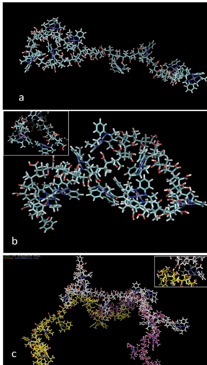
Figure 10. Structures obtained after short MD simulations of one strand (a, b) and 3 strands (c) for full protonation of the backbone, showing the interactions that help stabilizing a given morphology. The inset in b shows the H-bond interactions between the OH groups of the backbone and the annulene pendant. The inset in c. shows the H-bond interactions between carboxylate groups of different strands.
