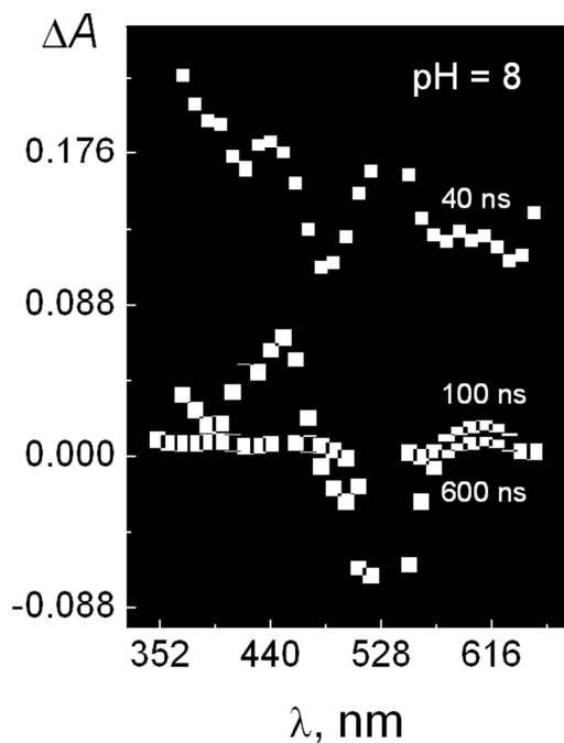
Figure 5. Transient spectra recorded when a deaerated aqueous solution of the polymer containing 2.2 \times 10^{-4} \text{ M} [\text{Ni}^{\text{II}}(\text{tmdbzTAA-CO- -})] pendants buffered at pH = 8 was flash irradiated at 532 nm. Delays from the laser flash used in these experiments are indicated in the figure.
