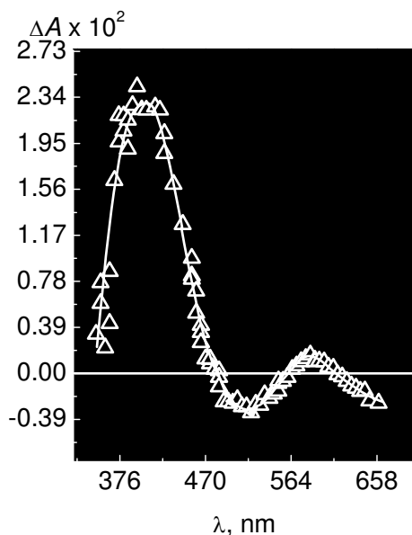
Figure 7. Transient spectrum recorded when a deaerated solution of poly(Ni II [tmdbzTAA]) 2 containing an electron acceptor was flash irradiated at 532 nm. The spectrum in the figure was recorded using 1.0 × 10 -2 M Co III (acac) 3 as the electron acceptor.
