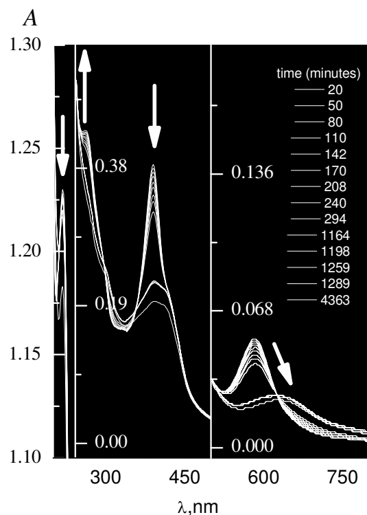
Figure 1. Changes of the poly(Ni II [tmdbzTAA]) 2 UV-Vis absorption spectrum with time due to the annulene ligand protonation. The inset show delays (in minutes) used when each spectrum was recorded and the arrows show the sense of the change in the spectrum.
