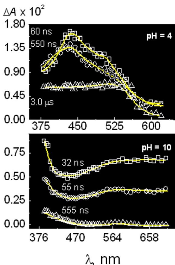
Figure 3. Transient spectra recorded when solutions of poly( \text{Ni}^{\text{II}}[\text{tmdbzTAA}]_2 ) that contained 1.0 \times 10^{-4} M [\text{Ni}^{\text{II}}(\text{tmdbzTAA-CO- -})] pendants buffered respectively at pH = 4 (top frame) and 10 (bottom frame) were flash irradiated at 351 nm. Delays from the laser flash used to record each spectrum and the pH of the solutions are indicated in the figure. In the solution buffered at pH = 10, a spectrum with a maximum at \lambda_{\text{max}} = 646 nm and another spectroscopic feature with \lambda_{\text{max}} \leq 385 nm is observed immediately after the laser flash. The position of the 646 nm maximum shifts with time to \sim 586 nm at the end of the spectroscopic change on the millisecond time domain. A significant change in the intensity of the bands takes place concurrent with the shift of the maximum. Inspection of the absorbance changes at 385 nm, \Delta A_{385} , and 547 nm, \Delta A_{547} , shows a ratio \Delta A_{385}/\Delta A_{547} \sim 1.3 at the end of the flash irradiation and \Delta A_{385}/\Delta A_{587} \geq 8.4 at the end of the spectroscopic change.
