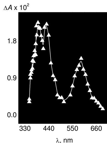
Figure 6. The 532 nm flash irradiation of a poly( \text{Ni}^{\text{II}}[\text{tmdbzTAA}]_2 ) solution containing 0.1 M phenol produced the spectrum shown with an absorption band at \lambda_{\text{max}} = 430 \text{ nm} assigned to the phenoxide radical.
