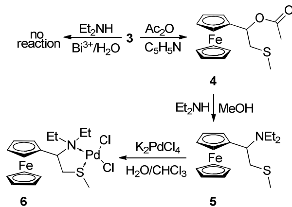
Scheme 2 Synthesis of complex 6 .
