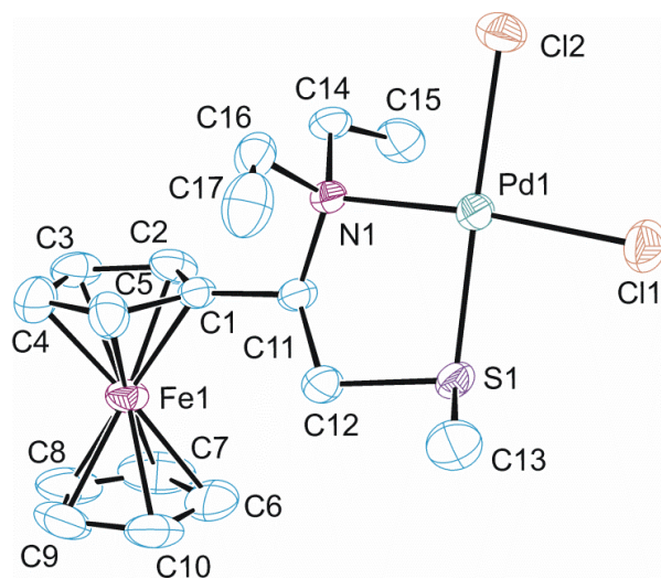
Fig. 1. The molecular structure of 6 with atom numbering scheme (hydrogen atoms and ethanol solvent molecule are omitted for clarity). Displacement ellipsoids are drawn at the 30% probability level. Other projections of the molecule are given in Fig. S1 (see Supporting Information). Selected bond lengths (Å) and angles (°): Pd1–N1 = 2.107(3), Pd1–S1 = 2.2350(10), Pd1–Cl1 = 2.3016(11), Pd1–Cl2 = 2.3387(11), N1–C16 = 1.496(5), N1–C14 = 1.504(5), N1–C11 = 1.543(5); N1–Pd1–S1 = 87.92(8), N1–Pd1–Cl1 = 174.67(9), S1–Pd1–Cl1 = 86.77(4), N1–Pd1–Cl2 = 93.73(8), S1–Pd1–Cl2 = 178.34(4), Cl1–Pd1–Cl2 = 91.58(5).
