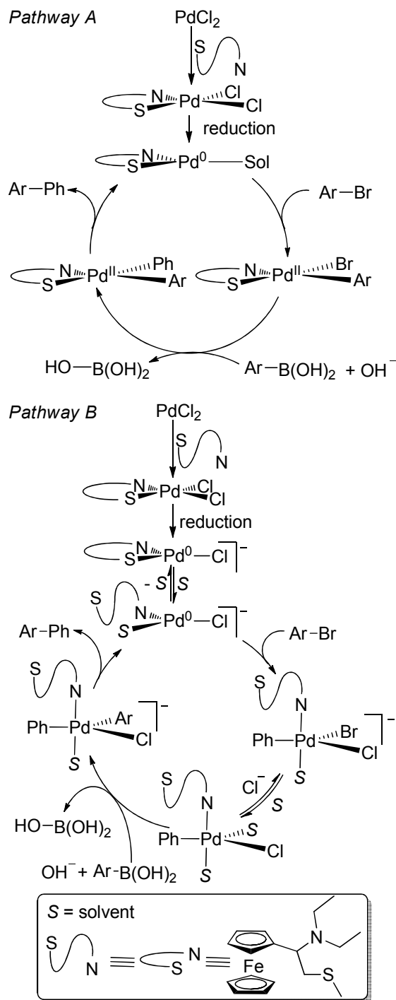
Scheme 6 The Suzuki-Miyaura couplings of phenylboronic acid with organic halides catalyzed by complex 6 .
