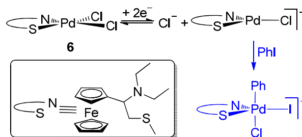
Scheme 4 Reduction of 6 at the working electrode and trapping of the obtained Pd 0 species.
