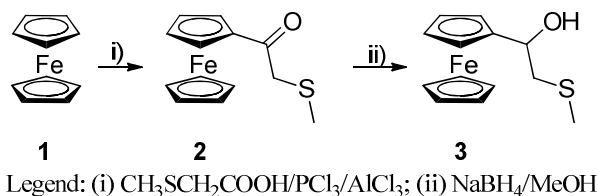
Scheme 1 Synthesis of alcohol 3 .
