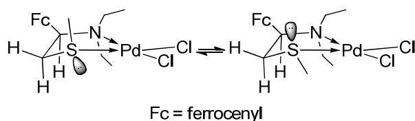
Scheme 3 Equilibrium between diastereoisomers of 6 in solution.
