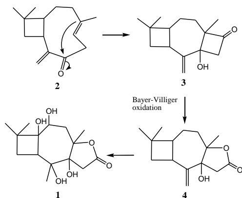
Fig. 3. A possible biogenetic pathway for 1 .
