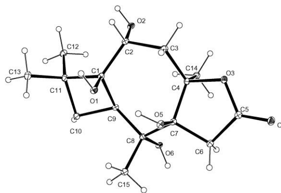
Fig. 2. Molecular projection of 1 .
