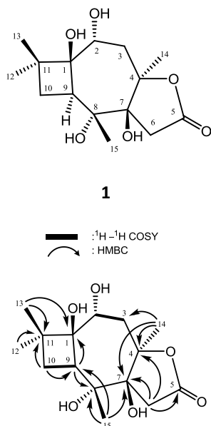
Fig. 1. The structure and its 1 H- 1 H COSY and selective HMBC of 1 .
