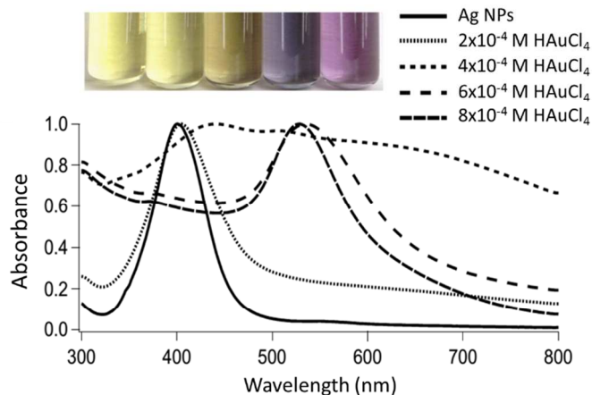
Figure 3. Representative optical images and UV-vis absorption spectra of Ag-Au BNPs with increasing Au fractional composition as determined by EDX. All spectra are normalized to their localized surface plasmon peak maxima. The nanoparticles were prepared by heating 1 mL of \approx 1 nM ( OD \approx 12 ) 22 nm Ag nanoparticles to \sim 100 °C and adding \text{HAuCl}_4 (1 to 8 \mu\text{L} ; 0.1 M) to the hot solution. The inset is a digital photograph of Ag and Ag-Au (made with 2 \times 10^{-4} M, 4 \times 10^{-4} M, 6 \times 10^{-4} M, and 8 \times 10^{-4} M of \text{HAuCl}_4 ) nanoparticles. For the UV-vis absorption spectra, the black solid line at 400 nm represents Ag nanoparticles and the dotted lines correspond to Ag-Au nanoparticles made with 2 \times 10^{-4} M, 4 \times 10^{-4} M, 6 \times 10^{-4} M, and 8 \times 10^{-4} M of \text{HAuCl}_4 , respectively.
