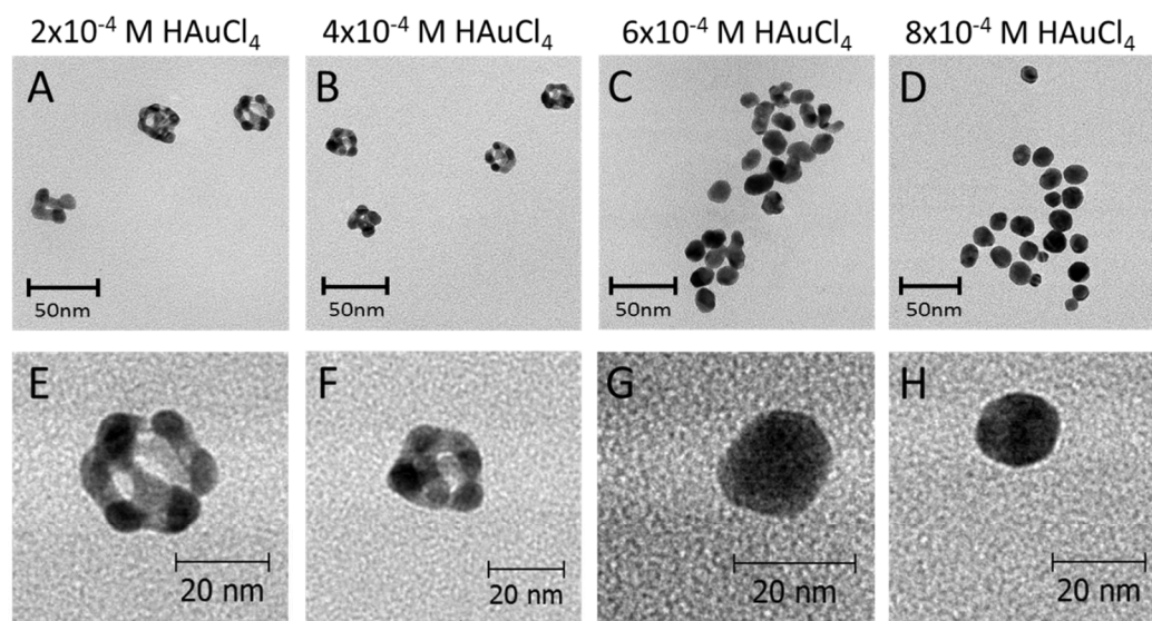
Figure 1. TEM images of Ag-Au nanoparticles. The nanoparticles were prepared by adding \text{H AuCl}_4 (1 to 8 \mu\text{L} ; 0.1 M) to 1 mL of \approx 1 \text{ nM} ( \text{OD} \approx 12 , \approx (22 \pm 3) \text{ nm} ) Ag nanoparticles. Top panel: representative TEM images of Ag-Au NPs prepared at 100^\circ\text{C} with (A) 2 \times 10^{-4} \text{ M} ( \approx 20\% \text{ Au} ), (B) 4 \times 10^{-4} \text{ M} ( \approx 50\% \text{ Au} ), (C) 6 \times 10^{-4} \text{ M} ( \approx 90\% \text{ Au} ), and (D) 8 \times 10^{-4} \text{ M} ( \approx 93\% \text{ Au} ) of \text{H AuCl}_4 . Bottom panel: high magnification TEM images of Ag-Au NPs prepared at 100^\circ\text{C} with (E) 2 \times 10^{-4} \text{ M} ( \approx 20\% \text{ Au} ), (F) 4 \times 10^{-4} \text{ M} ( \approx 50\% \text{ Au} ), (G) 6 \times 10^{-4} \text{ M} ( \approx 90\% \text{ Au} ), and (H) 8 \times 10^{-4} \text{ M} ( \approx 93\% \text{ Au} ) of \text{H AuCl}_4 .
