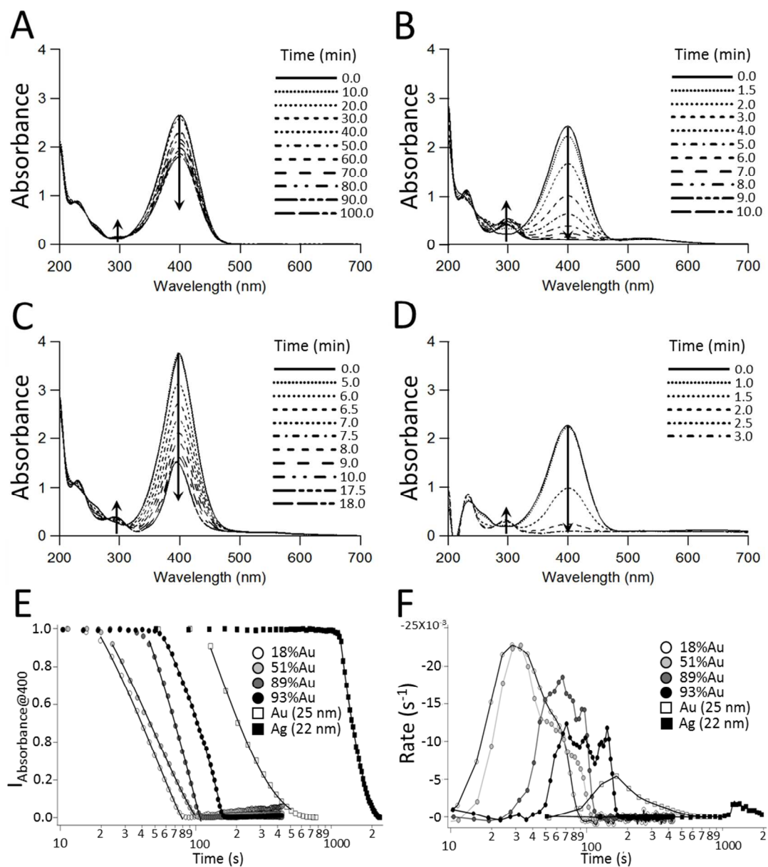
Figure 4. The reduction of 4-nitrophenol. The time evolution for the reduction of 1.5 \times 10^{-4} M (1.7 mL; 0.15 mM) 4-nitrophenol by 5 \times 10^{-3} M (1.0 mL; 0.015 M) NaBH 4 determined from UV-vis spectroscopy at 4 s (399 – 401 nm) or 30 s (200 – 700 nm) intervals. (A) Borohydride only, (B) Au NPs (300 \mu L) ( \approx 25 nm), (C) Ag NPs (300 \mu L) ( \approx 22 nm), and (D) Ag-Au NPs (300 \mu L) roughly 50% Au and \approx 22 nm. (E) The absorbance spectra at 400 nm for the reduction of 1.5 \times 10^{-4} M 4-NP by \sim 5 \times 10^{-3} M NaBH 4 in the presence of Ag-Au NPs ( \approx 18, 51, 89, and 93% Au) Au NPs ( \approx 25 nm), and Ag NPs ( \approx 22 nm). (F) The time evolution in the TOF for Ag-Au NPs ( \approx 18, 51, 89, and 93% Au) Au NPs ( \approx 25 nm), and Ag NPs ( \approx 22 nm). All reactions were run at 25 ^{\circ} C.
