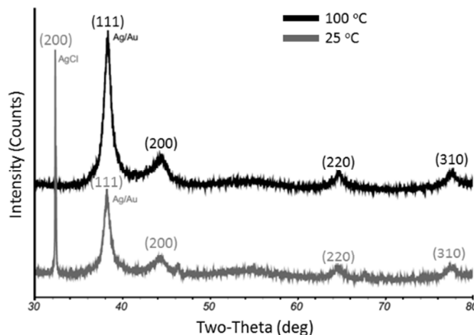
Figure 2. Representative XRD patterns of the Ag-Au nanoparticles. The nanoparticles were prepared by adding 1 \times 10^{-4} M \text{HAuCl}_4 (1 \mu\text{L} ; 0.1 M) to 1 mL of \approx 1 nM (OD \approx 12 ) 25 nm Ag NP seeds at 25 or 100 ^\circ\text{C} . Samples were centrifuged at 1500 \times g for 5 minutes to remove any AgCl precipitate prior XRD characterization. The 25 ^\circ\text{C} preparation has a (200) Bragg peak from AgCl.
