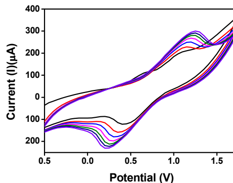
Fig. 2. CV of electropolymerization of P(TPFc-co-TPA) in DCM containing 0.1 mol L -1 TBAP 6 at 250 mV/s scan rate.
