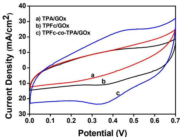
Fig. 4. CVs of a) TPA/GOx, b) TPFC/GOx and c) P(TPFC-co-TPA)/GOx (pH 4.5 Na-Acetate buffer, 50 mM at 250 mV/s scan rate.).
