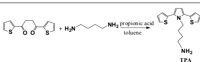
Scheme 2. The synthetic route for TPA
