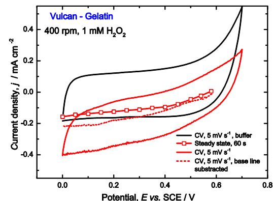
Fig. 2 Comparison of the electrode performance obtained using cyclic voltammetry and steady state methods. a) Vulcan-PVDF and b) Vulcan-Gelatin electrodes. Conditions: scan rate 5 \text{ mV s}^{-1} pH 6.00, \text{N}_2 atmosphere, enzyme loading: Vulcan-PVDF - 1 \text{ mg cm}^{-2} and Vulcan-Gelatin - 1.75 \text{ mg cm}^{-2}
