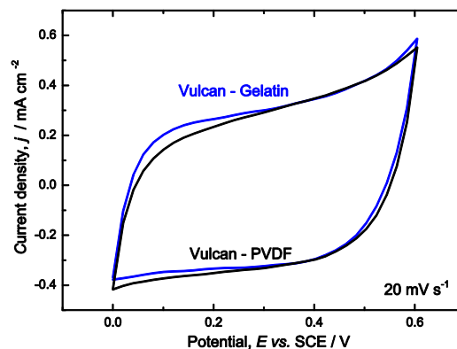
Fig. 5 Cyclic voltammograms of Vulcan HRP - electrodes in 0.1 M phosphate buffer. Conditions: scan rate 20 mV s -1 , 400 rpm, N 2 atmosphere, pH 6.00.
