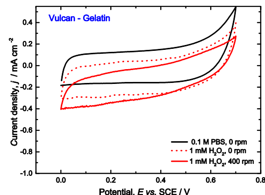
Fig. 1 Cyclic voltammograms of porous enzymatic electrodes in phosphate buffer and in 1 mM hydrogen peroxide, without rotation and at 400 rpm. a) Vulcan-PVDF and b) Vulcan-Gelatin. Conditions: scan rate 5 mV s -1 , pH 6.00, room temperature, N 2 atmosphere, enzyme loadings (1 mg cm -2 for Vulcan-PVDF and 1.75 mg cm -2 for Vulcan-Gelatin electrodes).
