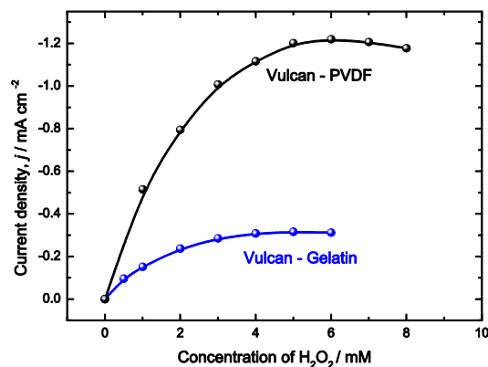
Fig. 4 Influence of the hydrogen peroxide concentration on the activity of Vulcan HRP - electrodes at optimized enzyme loadings. Conditions: enzyme loadings 1.75 mg cm -2 for Vulcan-Gelatin and 1.1 mg cm -2 for Vulcan-PVDF, electrode potential: 0.0 V vs. SCE, 400 rpm, N 2 atmosphere, pH 6.00.
