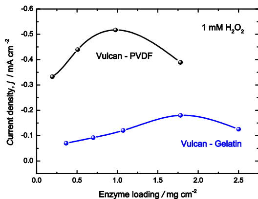
Fig. 3 Influence of enzyme loading on the activity of Vulcan HRP - electrodes, Conditions: 1 mM hydrogen peroxide, electrode potential: 0.0 V vs. SCE, 400 rpm, N 2 atmosphere, pH 6.00.
