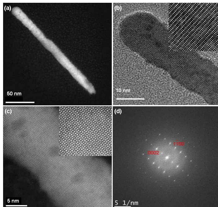
Fig. 4 (a) STEM images of ZnO ultra-thin NW with a diameter of less than 15nm. (b) HRTEM image of the nanowire and (c) HAADF-STEM image showing the atoms in the NW. Insets in (b) and (c) show the lattice planes and the atoms, respectively. (d) FFT pattern obtained from the HRTEM image 4b indicates that the growth axis of the nanowire is \langle 0001 \rangle .
