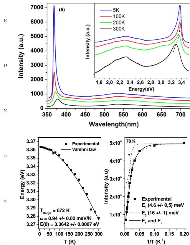
Fig. 5 Photoluminescence properties of the ultra narrow ZnO NWs grown on PS beads (lowest concentration). a) Typical PL spectra for 4 different temperatures as indicated. Inset shows the same spectra but in logarithmic scale and as a function of the energy. b) Varshni plot for the Near Band Edge emission and corresponding ZnO fitting parameters except for the Debye temperature which as explained in the text was taken from the literature. c) UV peak emission intensity as a function of the inverse of temperature. The solid line represents the best fit to the data by the use of two activation energies E_1 and E_2 . The dashed and dotted lines indicate the fits with a single activation energy E_1 or E_2 , respectively.
