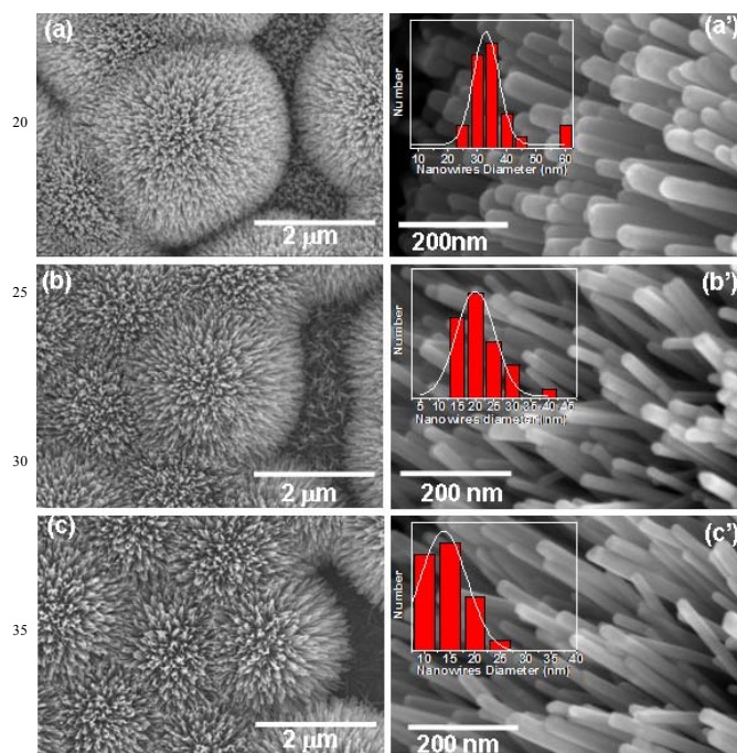
Fig. 6 SEM images of ZnO NWs grown as a function of varying solution concentration. Concentration of the solution used was (a, a') 0.029M, (b, b') 0.02M and (c, c') 0.018M respectively. (a, b, c) are low magnification SEM images while (a', b', c') are magnified SEM images of the NWs showing the diameter dispersion of the NW size. The insets on the upper left hand corner in (a', b', c') show the diameter distribution of the NWs while the white line on the histograms represents the corresponding fitted Gaussian distributions.
