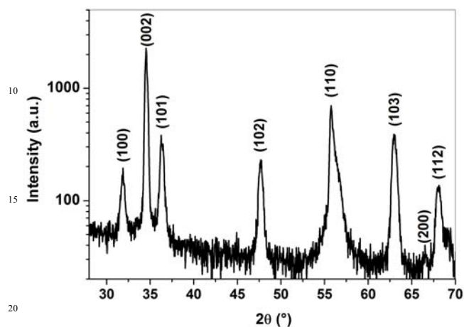
Fig. 3 A representative XRD pattern of ultra-thin crystalline ZnO NWs grown at a low concentration of 0.018M.
