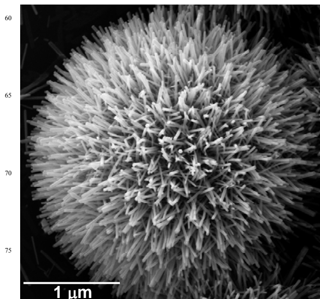
Fig. 1 SEM image of urchin-like ultra-thin ZnO NWs synthesized on PS beads as templates.
