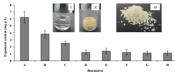
Fig. 1 Content of ergosterol (mg ergosterol g -1 of sample) in resting cells of A. flavus (A) and in the PAAFs: (B) Af-Pol EM-B; (C) Af-Pol EM-D; (D) Af-Pol BA; (E) Af-Pol DCPA; (F) Af-Pol AA; (G) Af-Pol EA; and (H) Af-Pol IL-HFP.
