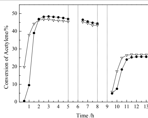
Fig. 8 Control experiments over Au/AC (●) and 1Au/5SiO 2 /AC (▽) catalysts: C 2 H 2 /HCl (5 h)→HCl (1 h)→C 2 H 2 /HCl (2 h)→C 2 H 2 (1 h)→C 2 H 2 /HCl (4 h).
