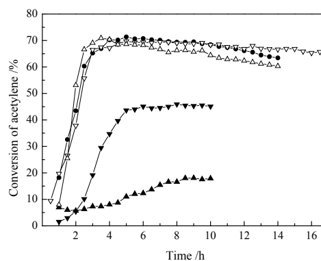
Fig. 1 Conversion of acetylene over 1Au/AC (●), 1Au/5SiO 2 /AC (▽), 5SiO 2 /1Au/AC (▼), 1Au/5SiO 2 (ammonia)/AC (Δ) and 5SiO 2 (ammonia)/1Au/AC (▲). C 2 H 2 flow rate was 12.5 mL/min, HCl/C 2 H 2 =1.13, GHSV=530/h.
