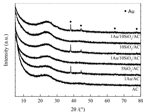
Fig. 5 XRD patterns of different samples
