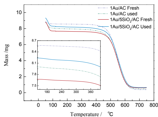
Fig. 3 TGA and DTGA profiles of AC, 1Au/AC, 5SiO 2 /AC and 1Au/5SiO 2 /AC
