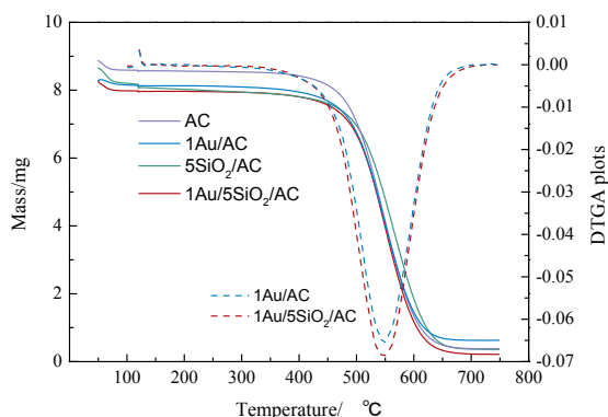
Fig. 9 TGA profiles of fresh and used 1Au/AC and 1Au/5SiO 2 /AC catalysts.
