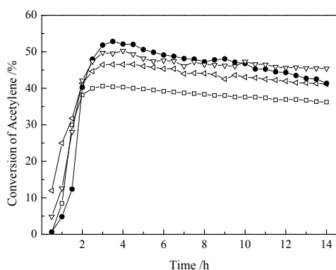
Fig. 2 Acetylene Conversion over 1Au/AC (●), 1Au/1SiO 2 /AC (□), 1Au/5SiO 2 /AC (▽), 1Au/10SiO 2 /AC (◁), C 2 H 2 flow rate was 25mL/min, HCl/C 2 H 2 =1.13, GHSV=1060/h.
