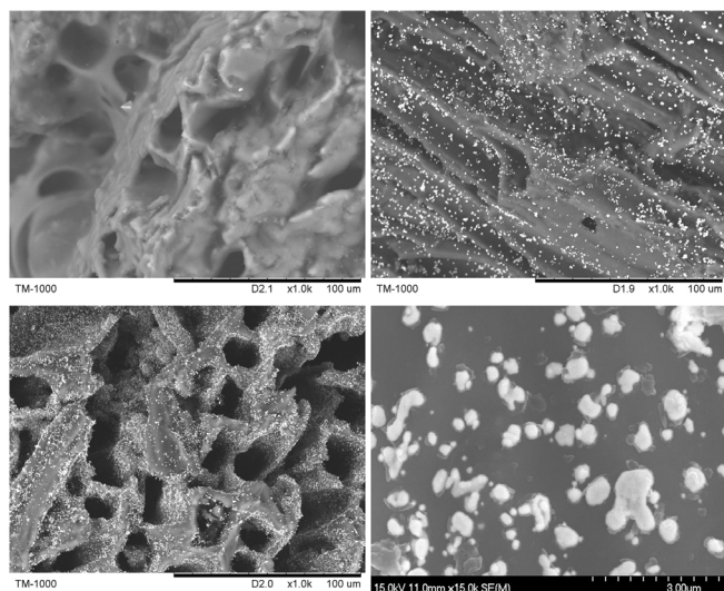
Fig. 4 SEM images of AC (a), 5SiO 2 /AC (b) and 1Au/5SiO 2 /AC (c, d)
