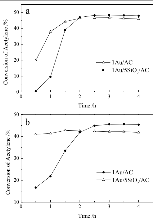
Fig. 7 Catalytic activity of 1Au/AC and 1Au/5SiO 2 /AC: (a) fresh, (b) after 32 h thermal treatment. C 2 H 2 flow rate was 25 mL/min, HCl/C 2 H 2 =1.13, GHSV=1060/h.
