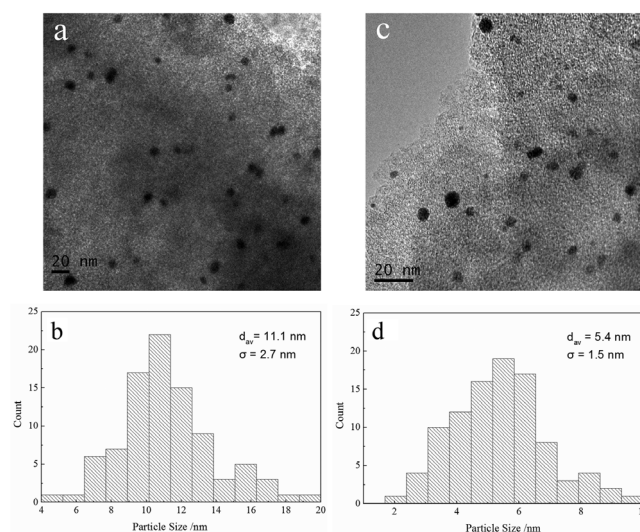
Fig. 6 TEM images and particle size distributions of fresh 1Au/AC (a, b) and 1Au/5SiO 2 /AC (c, d).
