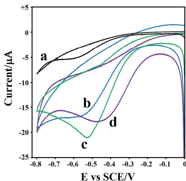
Figure 9. CV values of various electrodes in 0.2 M PBS (pH 6.5) in presence of 1.0 mM \text{H}_2\text{O}_2 : (a) bare GCE and AgNPs-rGO/GCE prepared by using different ultrasonication times of (b) 5 min, (c) 15 min and (d) 30 min.
