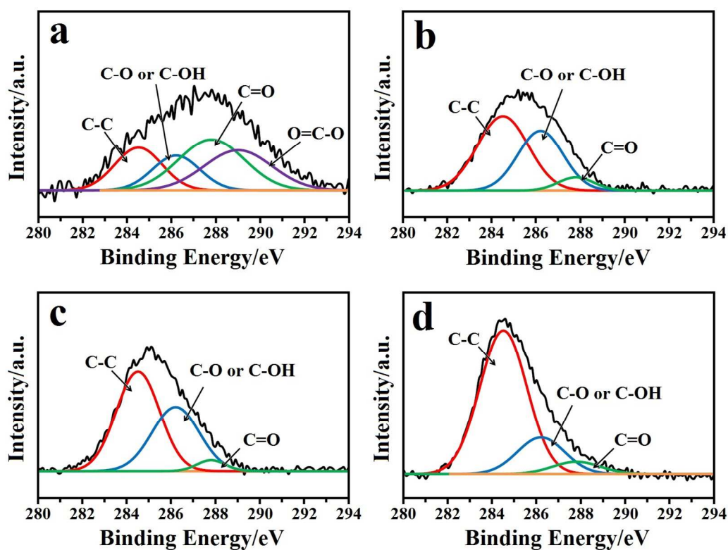
Figure 4. XPS spectra of pristine GO (a) and AgNPs-rGO prepared at different ultrasonic irradiation times: 5 min (b), 15 min (c) and 30 min (d).
