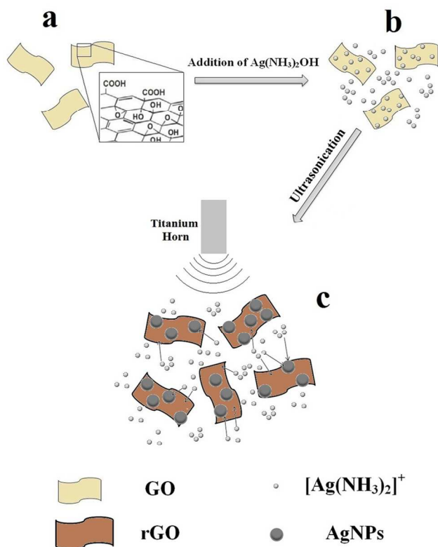
Figure 8. Schematic illustration of formation mechanism for AgNPs-rGO composite via ultrasonic irradiation.
