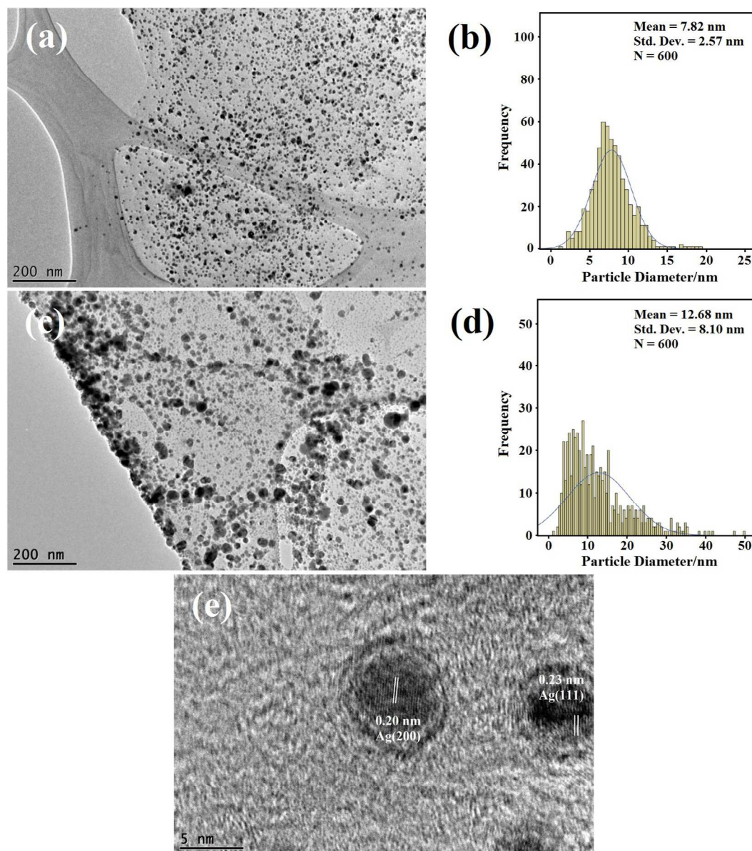
Figure 7. TEM images and size distribution diagrams of AgNPs-rGO prepared by using solution with GO (1.0 mg/mL) to \text{Ag}(\text{NH}_3)_2\text{OH} (0.04 M) volume ratio of 4 at different ultrasonic irradiation times of 15 min (a and b) and 30 min (c and d), and HRTEM image of AgNPs anchored on surface of graphene sheet (e).
