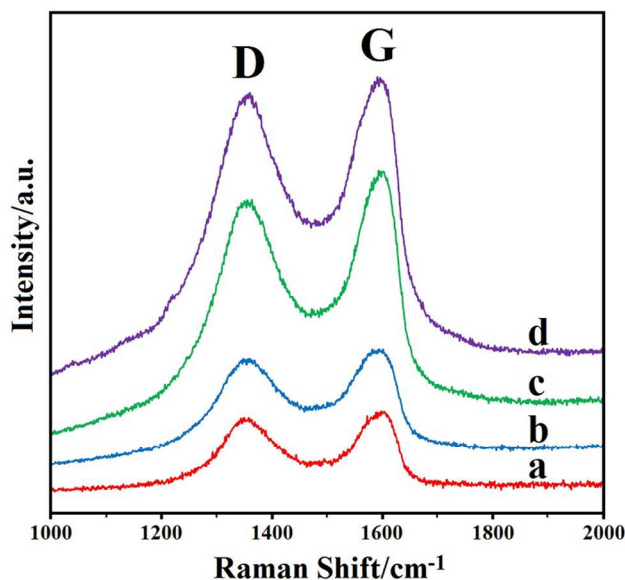
Figure 5. Raman spectra of pristine GO (a) and AgNPs-rGO prepared at different ultrasonic irradiation times: 5 min (b), 15 min (c) and 30 min (d).
