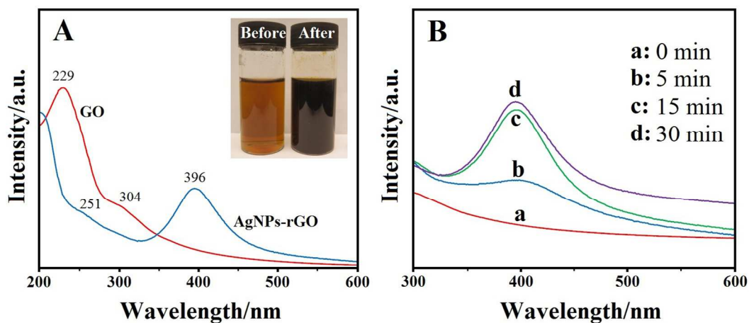
Figure 2. (A) UV–Vis absorption spectra of GO and AgNPs-rGO (inset shows photograph of solution of GO and \text{Ag}(\text{NH}_3)_2\text{OH} before and after ultrasonic irradiation) and (B) time evolution of UV–Vis absorption spectra of AgNPs-rGO.
