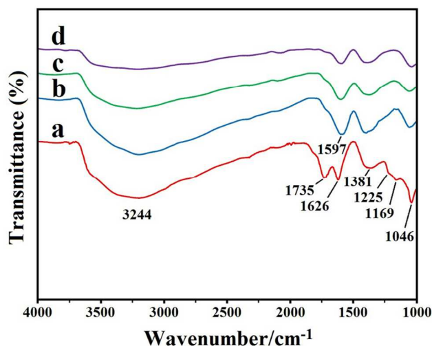
Figure 3. FTIR spectra of pristine GO (a) and AgNPs-rGO prepared at different ultrasonic irradiation times: 5 min (b), 15 min (c) and 30 min (d).
