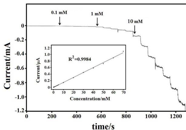
Figure 10. Steady-state response of AgNPs-rGO-4/GCE to successive injections of H_2O_2 into stirred 0.2 M PBS (pH 6.5) with applied potential of -0.4 V. The inset is the corresponding calibration curve.
