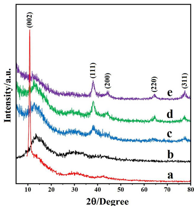
Figure 1. XRD patterns of pristine GO (a), sample holder (b) and AgNPs-rGO prepared at different ultrasonic irradiation times: 5 min (c), 15 min (d) and 30 min (e).
