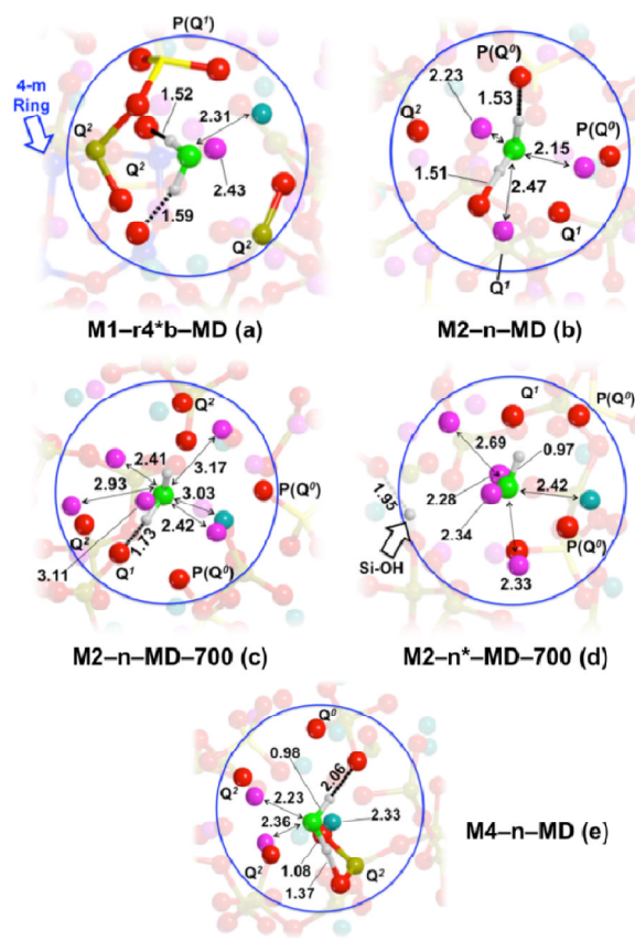
Fig. 7 Final configurations generated by optimizing structures sampled during CPMD trajectories. Symbols and notation as in Fig. 3.
