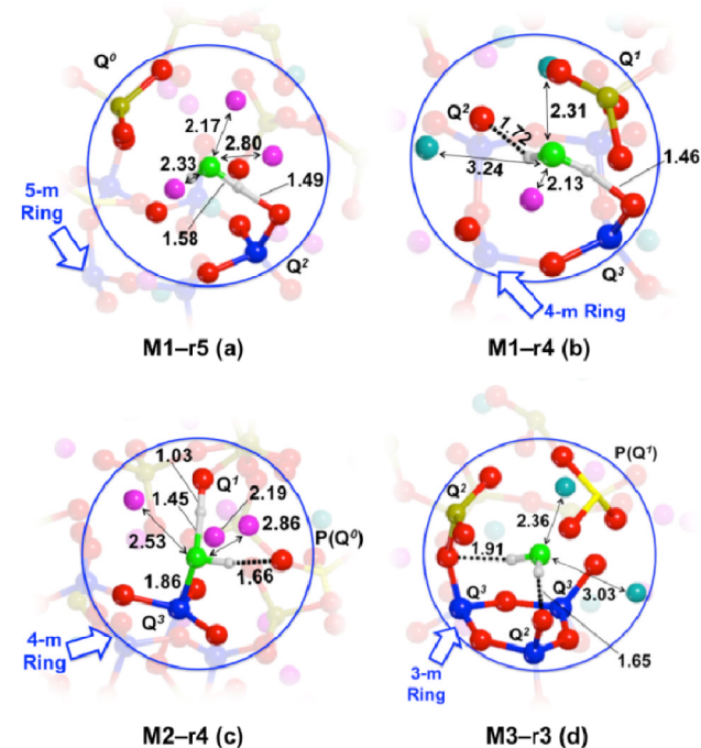
Fig. 3 Optimized water/BG45 configurations with water initially inserted in the proximity of a ring: (a) M1-r5, (b) M1-r4, (c) M2-r4 and (d) M3-r3. Colour codes are red (O), ochre (Si), yellow (P), magenta (Na), cyan (Ca). Si atoms forming the ring are blue and the water oxygen is green. Atoms contained inside the water coordination sphere (the sphere of radius 3.3 \text{ \AA}^{23} centred on the water oxygen) are highlighted in the foreground, whereas the other atoms are shadowed. Hydrogen bonds are shown as bold-dashed dark lines. Relevant interatomic distances are shown. The arrows highlight the position of the relevant ring.
