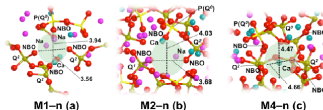
Fig. 2 BG45 cages studied in this work: (a) M1-n, (b) M2-n, and (c) M4-n.
