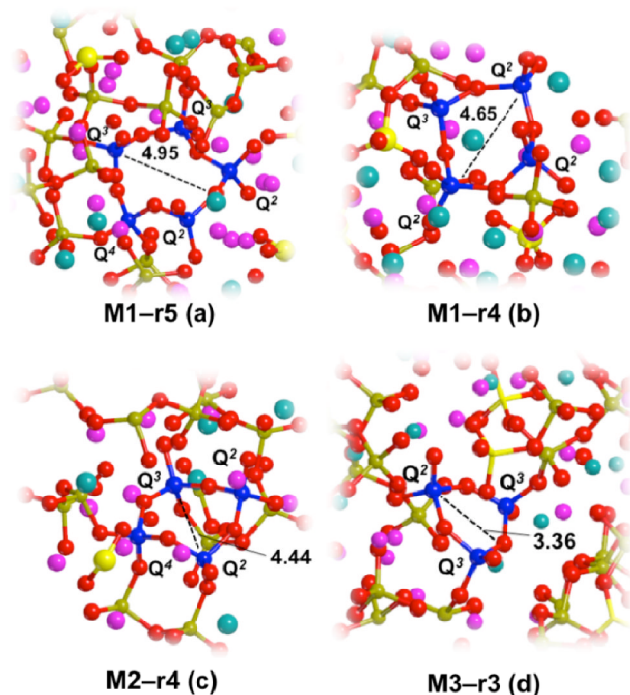
Fig. 1 BG45 rings probed in this work: (a) 5-m and (b) 4-m ring from model 1, (c) 4-m ring from model 2 and (d) 3-m ring from model 3.
