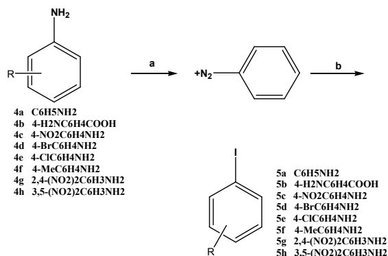
Scheme 2: Synthesis of the aryl iodide 5a-f by using Fe 3 O 4 @SILnP as catalyst. Reagents and conditions (a) NaNO 2 , Fe 3 O 4 @SILnP, drops of H 2 O, 0°C (b) NaI, 0°C to RT
