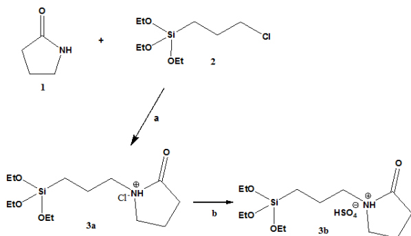
Scheme 1: Synthesis of N-(propyl triethoxysilane)-2-pyrrolidone. Reagents and condition (a) dry toluene, reflux, 24 h (b) \text{H}_2\text{SO}_4 , DCM, 0^\circ\text{C} to 60^\circ\text{C} , 12h.
