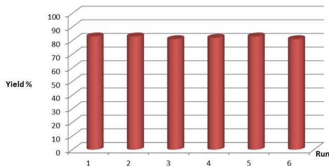
Figure 6: Reuse of Fe 3 O 4 @SILnP in the diazotization-iodination of 4-NO 2 C 6 H 4 NH 2
