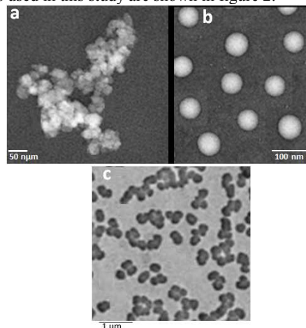
Figure 2 The micro-pictures of (A) naked \text{Fe}_3\text{O}_4 particles (TEM); (B) magnetic silica nanoparticles (TEM); (C) magnetic silica nanoparticles modified with ionic liquids.
