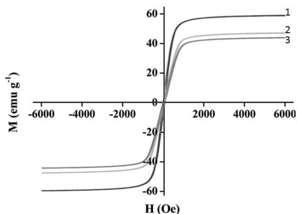
Figure 3: Magnetization curve of (1) magnetite nanoparticles (2) silica coated \text{Fe}_3\text{O}_4 and (3) magnetic silica nanoparticles modified with ionic liquids.
