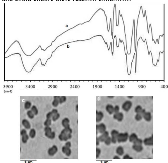
Figure 7: FT-IR spectra and the Transmission electron microscope (TEM) images of the fresh catalyst (a, c), and the used catalyst after 6 cycles (b, d).
