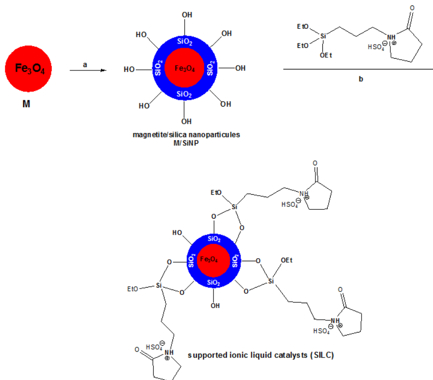
Figure 1: general structure of the supported ionic liquid catalysts ( \text{Fe}_3\text{O}_4@\text{SILNP} ) based on N-propyl-2-pyrrolidonium hydrogen sulfate ([NPP] \text{HSO}_4^- ) bonded to nano-sized silica-coated magnetite. (a) \text{H}_2\text{O} / EtOH / \text{NH}_3 aq, sonication, TEOS, 12 h (b) toluene, reflux, 24 h.
