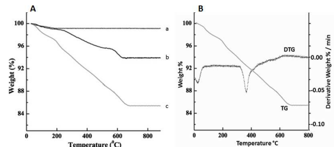
Figure 4: (A) Thermogravimetric (TG) curves for (a) magnetite (b) silica coated magnetite and (c) magnetic silica nanoparticles modified with ionic liquids (SILnP) and (B) TG-DTG curves for \text{Fe}_3\text{O}_4@\text{SILnP}
