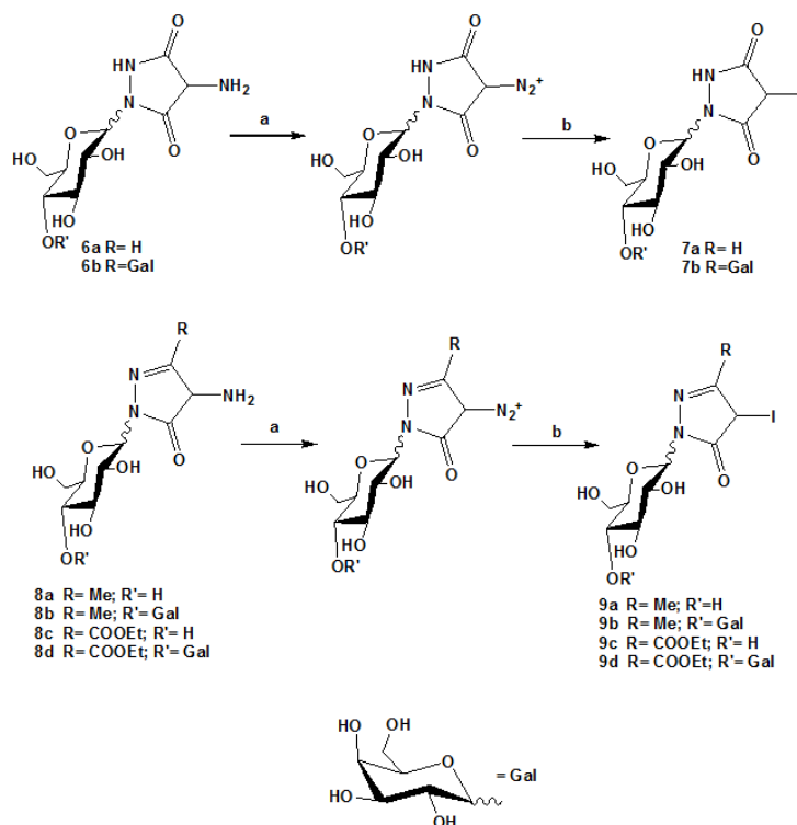
Scheme 3: Synthesis of the pyrazolidine-3,5-dione iodides 7a-b , and pyrazolin-5-one iodides 9a-d by using \text{Fe}_3\text{O}_4@\text{SiLNp} as catalyst. Reagents and conditions (a) \text{NaNO}_2 , \text{Fe}_3\text{O}_4@\text{SiLNp} , drops of \text{H}_2\text{O} , 0^\circ\text{C} (b) \text{NaI} , 0^\circ\text{C} to RT
