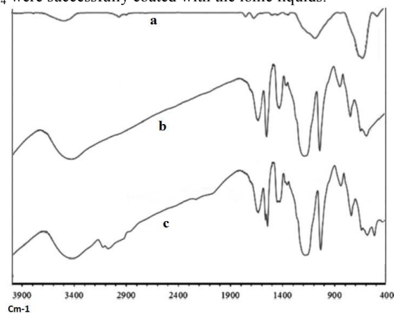
Figure 5: FT-IR Spectrum (a) silica coated \text{Fe}_3\text{O}_4 , (b) [H-NPP] \text{HSO}_4 ionic liquid and (c) magnetic silica nanoparticles modified with ionic liquids
