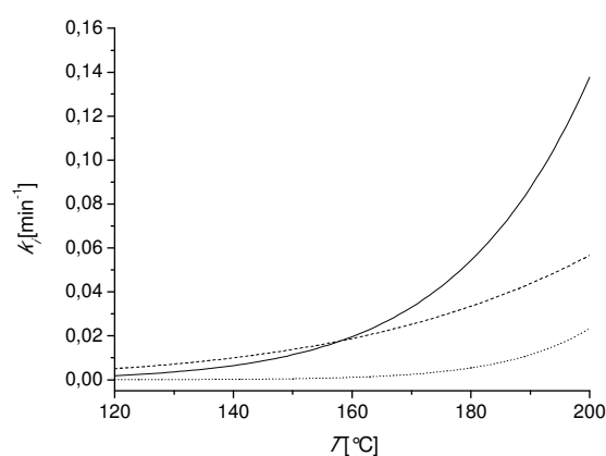
Fig. 5: Kinetic rate constants k_3 (solid line), k_4 (dashed line) and k_5 (dotted line) in dependency of the temperature and a constant catalyst concentration of c = 0.01 M. The rate constants are calculated using (eq. 7) and the parameters of Tab. 3.
