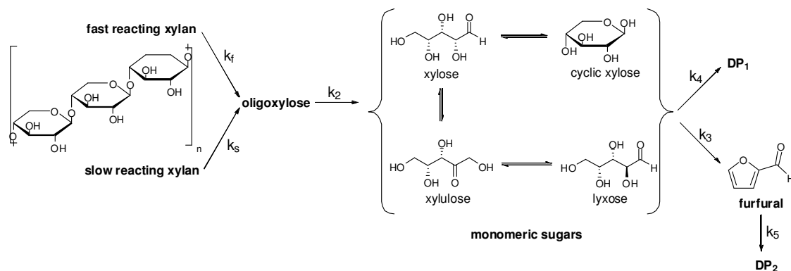
Fig. 1: Reaction model used to determine the kinetic rate constants of the xylan hydrolysis. MS \equiv monomeric sugars; DP \equiv degradation products, in the following text also often described as byproducts.
