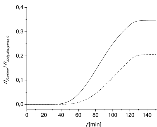
Fig. 7: Calculated furfural concentration profile in the larger scale experiment using (eq. 7). Dashed line: Sample 1; Solid line: Sample 2.
