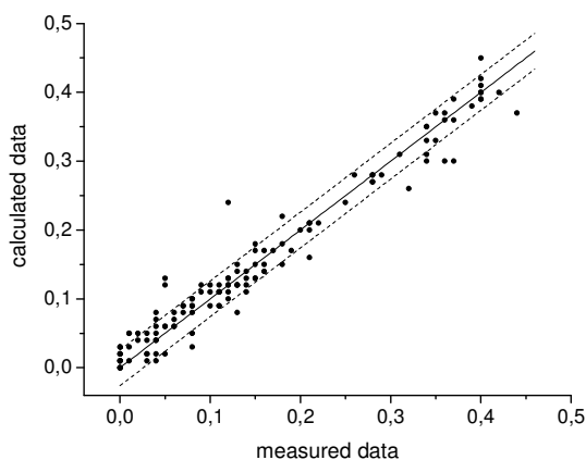
Fig. 3: Comparison of the measured and with the Matlab calculated amounts of xylan, monomeric sugars and furfural. The solid line has an intercept of zero and a slope of one. The dashed lines are the upper and the lower boundaries of the mean error.
