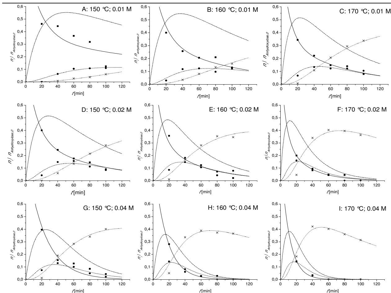
Fig. 2: Kinetic plots of the xylan hydrolysis during Methanosolv pulping of beech wood. ■ xylan; ● monomeric carbohydrates; X furfural; solid line: fitted xylan; dashed line: fitted monomeric carbohydrates; dotted line: fitted furfural; dashed/dotted line: calculated oligoxylose; Reaction conditions: A: 150°C, 0.01 M AICl 3 ; B: 160°C, 0.01 M AICl 3 ; C: 170°C, 0.01 M AICl 3 ; D: 150°C, 0.02 M AICl 3 ; E: 160°C, 0.02 M AICl 3 ; F: 170°C, 0.02 M AICl 3 ; G: 150°C, 0.04 M AICl 3 ; H: 160°C, 0.04 M AICl 3 ; I: 170°C, 0.04 M AICl 3 . The reaction temperature and the catalyst concentration are additionally shown on top right of each graph.
