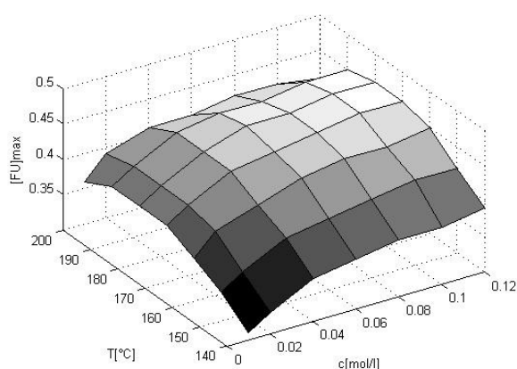
Fig. 4: 3-D-plot of the maximum furfural yields in dependency of the catalyst concentration and the temperature. The yields are calculated with Matlab using (eq. 7) and the values from Tab. 3.
