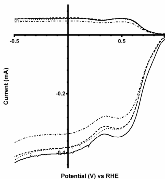
Fig. 5 RRDE LSVs of \text{Ca}_2\text{Ru}_{1.75}\text{Bi}_{0.25}\text{O}_{6.75} in \text{O}_2 -saturated aqueous KOH ( 1 \text{ mol dm}^{-3} ) and varying concentrations of \text{K}_2\text{CO}_3 at 600 rpm: solid line = \text{K}_2\text{CO}_3 -free, dashed = 0.01 \text{ mol dm}^{-3} , dotted = 0.05 \text{ mol dm}^{-3} , and dash-dot = 0.1 \text{ mol dm}^{-3} .
