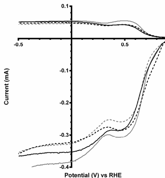
Fig. 6 RRDE LSVs of \text{Ca}_2\text{Ru}_{2.25}\text{Bi}_{0.75}\text{O}_{7.75} ( x = 0 in black and x = 0.25 in grey) in \text{O}_2 -saturated aqueous KOH ( 1 \text{ mol dm}^{-3} ) containing the following concentrations of \text{K}_2\text{CO}_3 : solid line = 0 \text{ mol dm}^{-3} ( \text{CO}_3^{2-} -free baseline) and dashed = 0.1 \text{ mol dm}^{-3} . Rotation rate = 600 rpm.
