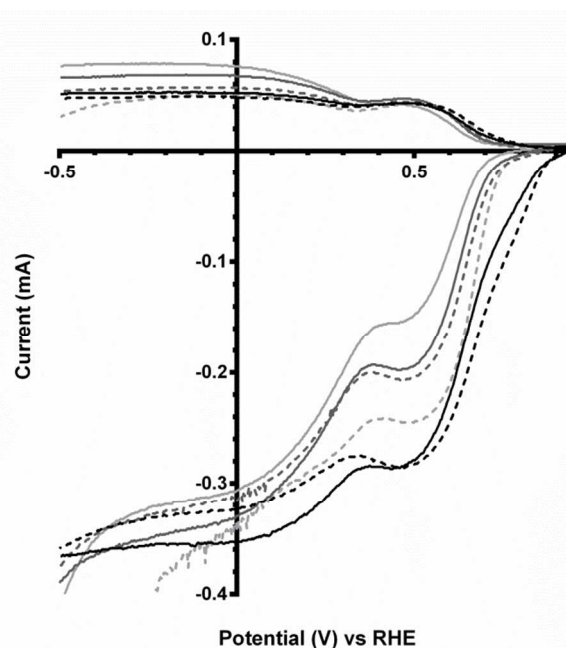
Fig. 9 RRDE LSVs of \text{Ca}_2\text{Ru}_{2-x}\text{Bi}_x\text{O}_{7-y} ( x = 0 in black, x = 0.5 in dark grey, and x = 0.75 in light grey) in \text{O}_2 -saturated aqueous KOH ( 1 \text{ mol dm}^{-3} ) containing the following concentrations of \text{K}_2\text{CO}_3 : solid line = 0 \text{ mol dm}^{-3} ( \text{CO}_3^{2-} -free baseline) and dashed = 0.1 \text{ mol dm}^{-3} . Rotation rate = 600 rpm.
