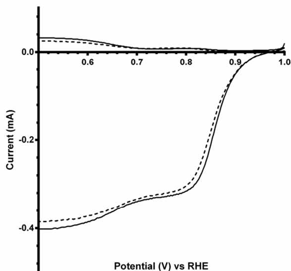
Fig. 17 RRDE LSVs of Pt black catalyst in in O 2 -saturated aqueous KOH (1 mol dm -3 ) containing the following concentrations of K 2 CO 3 : solid line = 0 mol dm -3 (CO 3 2- -free baseline) and dashed = 0.1 mol dm -3 . Rotation rate = 600 rpm.
