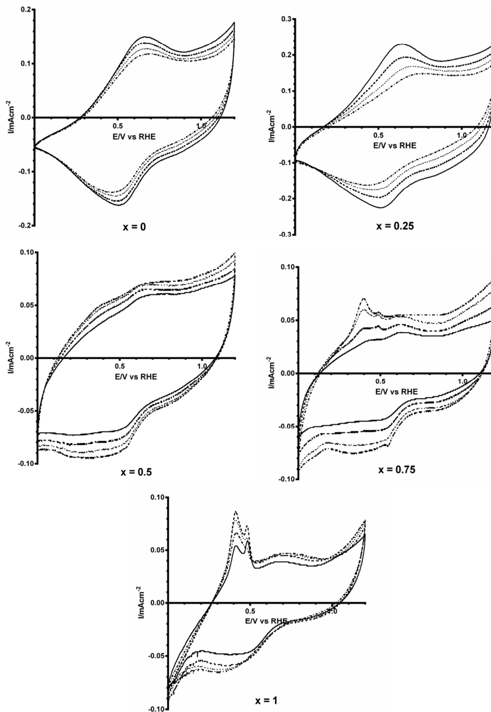
Fig. 3 Cyclic voltammograms of \text{Ca}_2\text{Ru}_{2-x}\text{Bi}_x\text{O}_{7-y} ( x = 0, 0.25, 0.5, 0.75 and 1 ) catalysts in \text{N}_2 -saturated \text{KOH} showing the increasing double layer capacitance on addition of increasing concentrations of \text{CO}_3^{2-} into the electrolyte: solid = no \text{K}_2\text{CO}_3 [ \text{KOH} -only blank experiment], dashed = 0.01 \text{ mol dm}^{-3} , dotted = 0.05 \text{ mol dm}^{-3} , and dash-dot = 0.1 \text{ mol dm}^{-3} .
