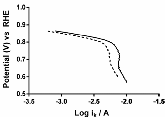
Fig. 18 Tafel plots of Pt black in in O 2 -saturated aqueous KOH (1 mol dm -3 ) with varying concentrations of K 2 CO 3 : solid = K 2 CO 3 -free and dashed = 0.1 mol dm -3 .
