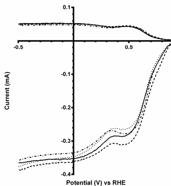
Fig. 4 RRDE Linear sweep voltammograms (LSV) of \text{Ca}_2\text{Ru}_2\text{O}_7 in \text{O}_2 -saturated aqueous KOH (1 mol \text{dm}^{-3} ) at different scan rates (top) and \text{O}_2 -saturated aqueous KOH (1 mol \text{dm}^{-3} ) with varying concentrations of \text{K}_2\text{CO}_3 at 600 rpm (bottom): solid line = \text{K}_2\text{CO}_3 -free, dashed = 0.01 mol \text{dm}^{-3} , dotted = 0.05 mol \text{dm}^{-3} , and dash-dot = 0.1 mol \text{dm}^{-3} .
