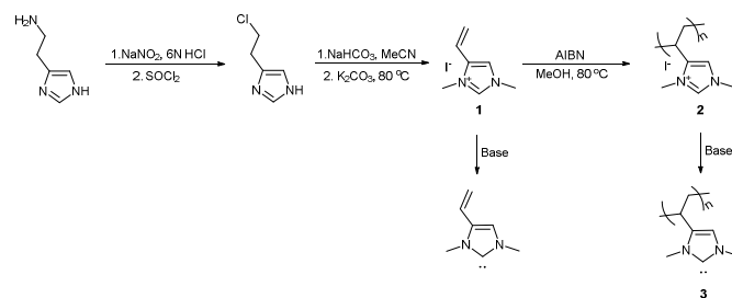
Scheme 1. Synthesis of 1 and 2 from Histamine
