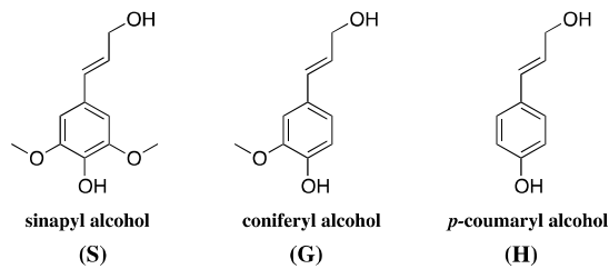
Figure 3: The three main monomer building blocks of lignin.
