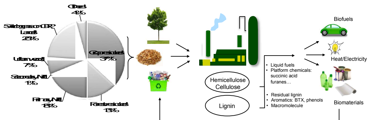
Figure 2: Cartoon showing the role of the future biorefinery as part of a fully integrated agro-biofuel-biomaterial-biopower cycle. The pie chart shows the distribution of vegetal biomass by volume. (CRP=Conservation Reserve Program)
