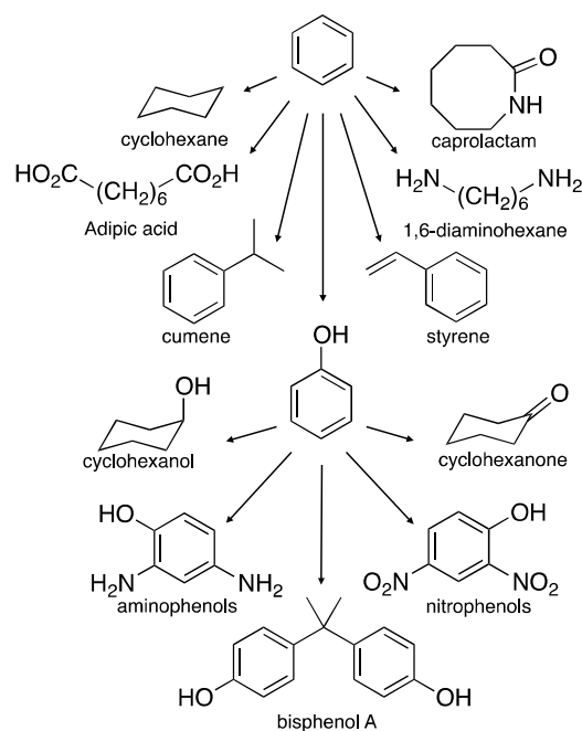
Figure 5: Current petrochemical products starting from benzene and phenol.
