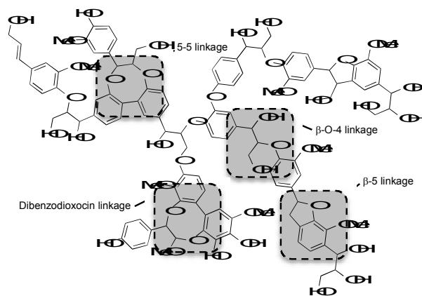
Figure 4: Schematic representation of lignin chemical bonds.
