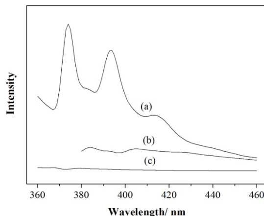
Figure 6. Fluorescence spectra of NPM solution (300 mg L -1 ) in acetonitrile: (a) after addition of MIP-SH (10 mg L -1 , excitation wavelength 343 nm), (b) before addition of MIP-SH (excitation wavelength at 360 nm), (c) before addition of MIP-SH (excitation wavelength 343 nm).
