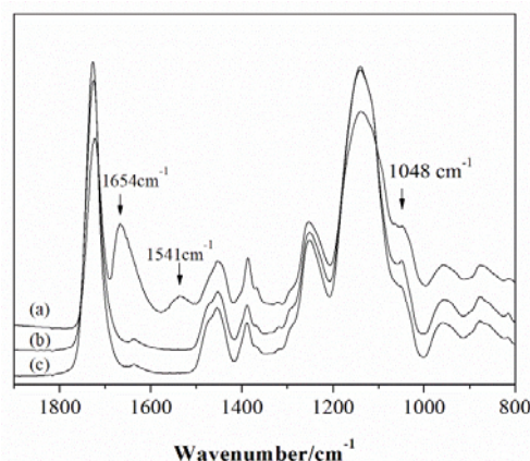
Figure 5. FTIR spectra of (a) MIP-polyNIPAm, (b) MIP, and (c) MIP-SH.
