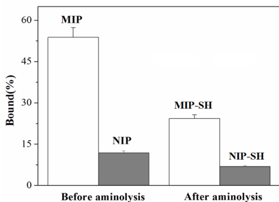
Figure 7. Uptake of nicotine ( 0.155 \text{ mM} ) in acetonitrile by the imprinted and non-imprinted polymer microspheres ( 5 \text{ mg mL}^{-1} ) before and after the aminolysis treatment.
