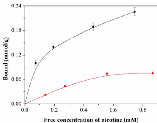
Figure 2. Equilibrium binding of nicotine to the MIP (■) and the NIP (●) microspheres. The particle concentration was 5 mg/mL in acetonitrile.
