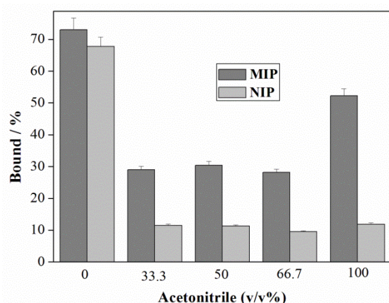
Figure 4. Uptake of nicotine (0.155 mM) by 5 mg of polymer microspheres in water containing different amount of acetonitrile.
