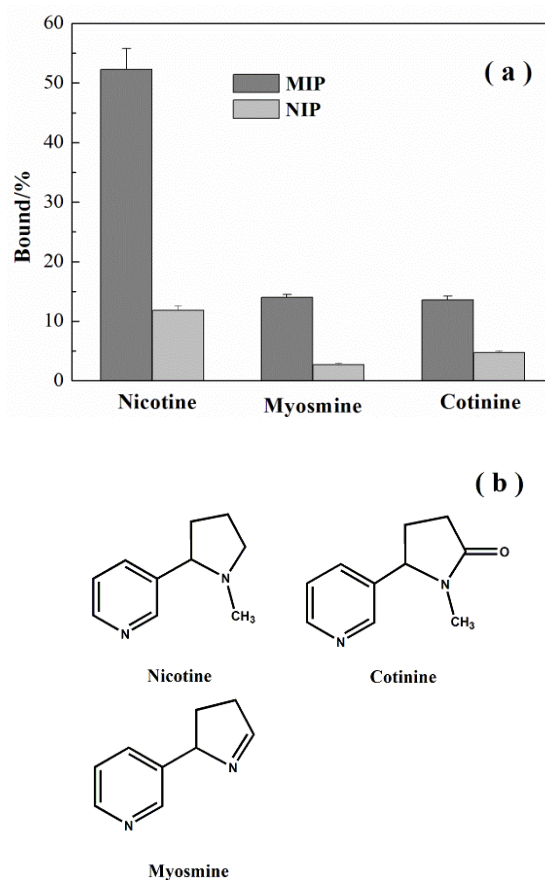
Figure 3. (a) Uptake of nicotine and its structural analogues (0.155 mM) by MIP and NIP microspheres (5 mg) in 1 mL of acetonitrile. (b) Chemical structures of the tested analytes.
