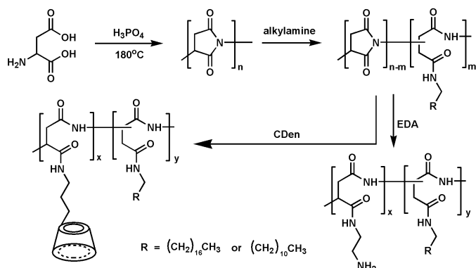
Scheme 1 Synthesis of PSI (A), PASP-DDA/ODA-CDen (B) and PASP-DDA/ODA-EDA (C)
