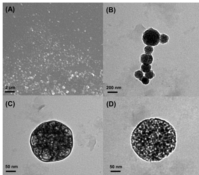
Figure 4 SEM image (A), TEM image (B) of PASP-ODA-DDA-CDen and enlarged TEM of PASP(45K)-DDA-CDen (C) and PASP(45K)-DDA-EDA (D) in octanol solution at 25 °C.
