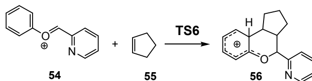
Scheme 15. [4^++2] I-DA reaction between oxonium cation 54 and cyclopentene 55 .
