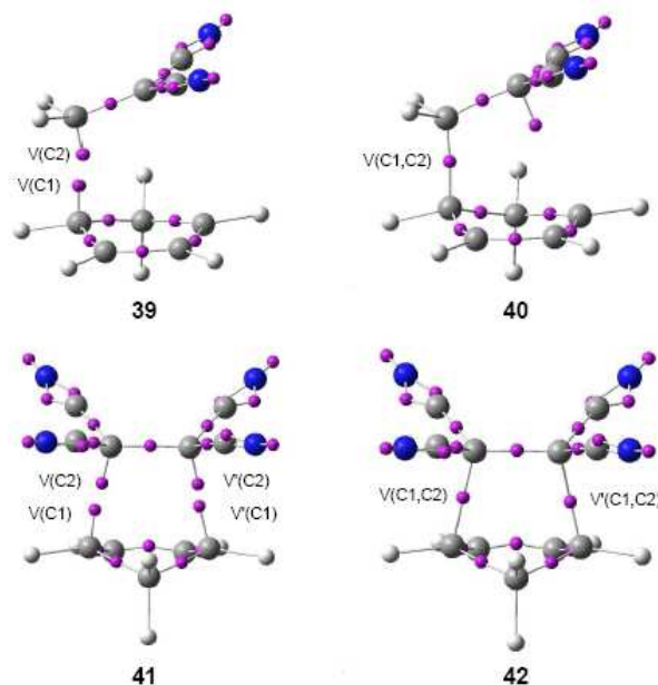
Figure 9. ELF attractors at selected points of the IRC of the P-DA reactions between Cp 4 and DCE 6 , 39 and 40 , and TCE 14d , 41 and 42 .
