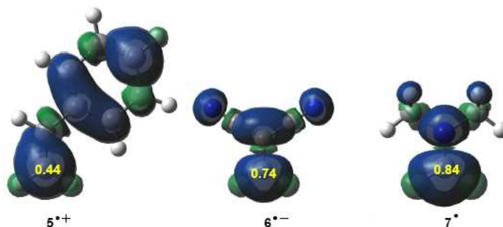
Figure 10. Nucleophilic P_k^- function of styrene 5 , electrophilic P_k^+ Parr function of DCE 6 , and radical P_k^o Parr functions of iminium cation 7 .
