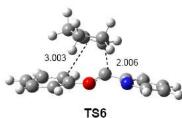
Figure 13. TS6 associated with the [4^++2] I-DA reaction between the oxonium cation 54 and cyclopentene 55 .
