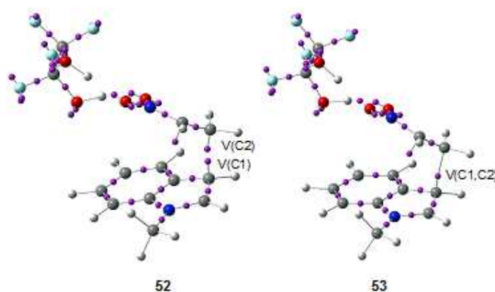
Figure 12. Selected structures 52 and 53 involved the formation of the C–C single bond formation in the Friedel-Crafts reaction shown in Scheme 13.
