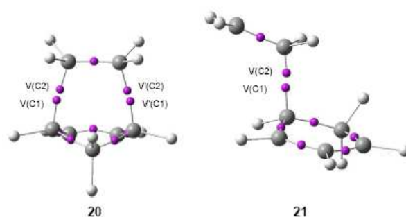
Figure 7. Semblance between the pseudodiradical structure 20 involved in the one-step mechanism, and the diradical structure 21 involved in the stepwise mechanism of the N-DA reaction between Cp 4 and ethylene 2 .
