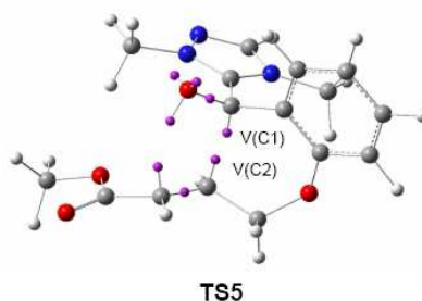
Figure 11. TS5 associated with the C–C bond formation in Breslow intermediate 43 .
