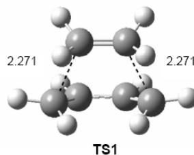
Figure 1. B3LYP/6-31G* transition structure TS1 associated with the DA reaction between butadiene 1 and ethylene 2 . Distances are given in Angstroms.
