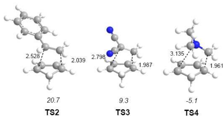
Figure 2. TSs involved in the DA reactions of Cp 4 with styrene 5 , TS2 , with dicyanoethylene 6 , TS3 , and with iminium cation 7 , TS4 . Relative energies are given in kcal/mol, while distances are given in Angstroms.
