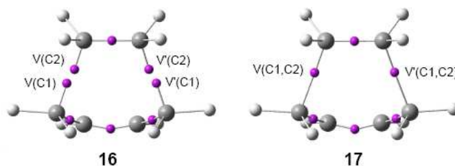
Figure 5. Most relevant ELF attractors in the structures of phase V, structure 16 , and phase VI, structure 17 , involved in the synchronous C–C single bond formation in the N-DA reaction between butadiene 1 and ethylene 2 . The pseudoradical centers involved in the C–C bond formation are characterised by the four V(C) monosynaptic basins present in structure 16 .
