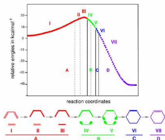
Figure 6. Reaction path calculated by means of the IRC method for the DA reaction between butadiene 1 and ethylene 2 . \Delta E are in kcal/mol. A bonding between atoms in all phases is demonstrated by the standard Lewis representation; however, in the case of
