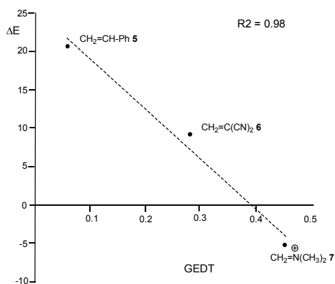
Figure 4. Plot of the activation energies \Delta E , in kcal/mol, vs GEDT, in e, for the DA reactions given in Scheme 3.
