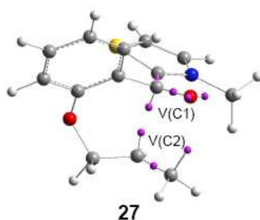
Figure 8. Pseudodiradical structure 27 generated along the C–C bond formation step in the N-heterocyclic carbene-catalysed hydroacylation of unactivated C–C double bonds.
