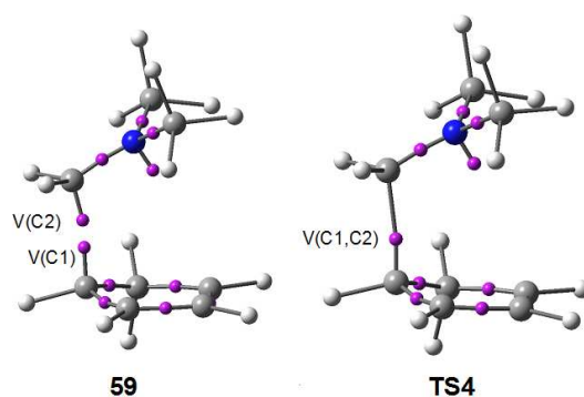
Figure 15. The most relevant ELF attractors in structure 59 and TS4 involved in the C–C single bond formation in the I-DA reaction between Cp 4 and iminium cation 7 .
