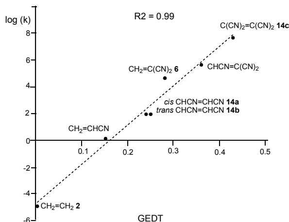
Figure 3. Plot of the logarithm of the experimental rate constant k vs GEDT, in e, R^2 = 0.99 , for the DA reactions of Cp 4 with ethylene 2 , and the cyanoethylene series.
