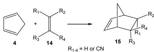
Scheme 5. DA reactions between Cp 4 and cyanoethylene series 14 .
