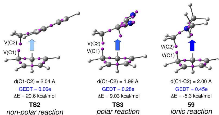
Figure 16. Most relevant data of pseudodiradical structures involved in the C–C bond formation in the N-DA reaction of Cp 4 with styrene 5 , in the P-DA reaction of Cp 4 with DCE 6 , and in the I-DA reaction of Cp 4 with iminium cation 7 . The blue arrow indicates the direction of GEDT.
