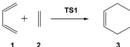
Scheme 1. DA reaction between butadiene 1 and ethylene 2 .
