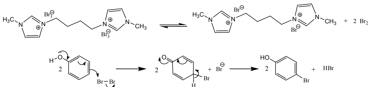
Scheme 4. Plausible mechanism.
