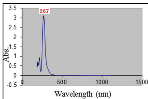
Figure 2. The UV absorption of [bMImB].(Br 3 ) 2 .
