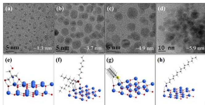
Fig. 9 (a-d) TEM images of varied-sized ZnO NPs prepared from zinc acetate and sodium hydroxide in ethanol in the presence of different ligands: (a) THMA, (b) TOPO, (c) DDT, and (d) HDA. (e-h) are the corresponding optimised surface structures of ZnO NPs capped with ligands used in (a-b), respectively (adapted with permission from ref. 72, copyright 2012, Springer).
