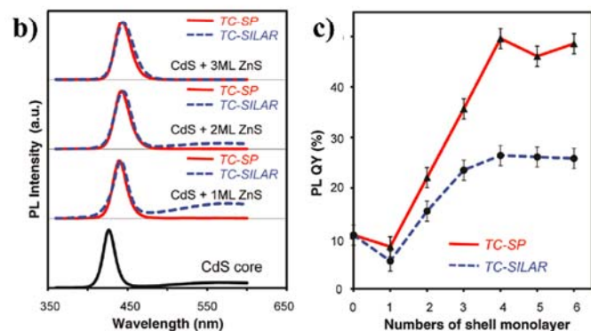
Fig. 11 (a) The reaction scheme for the synthesis of CdS/ZnS core/shell NCs via the TC-SP method. (b) PL properties of the CdS/ZnS core/shell NCs in comparison to the initial CdS core NCs. (c) The comparison of the PL-QY of CdS/ZnS NCs grown by both TC-SP and thermal-cycling coupled SILAR (TC-SILAR) methods (reproduced with permission from ref. 96, copyright 2010, American Chemical Society).
