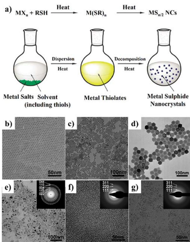
Fig. 5 (a) Schematic illustration of the “non-injection” method for the synthesis of metal sulphide NCs. (b–j) Representative TEM images of NCs obtained by the “non-injection” method: (b) \text{Ag}_2\text{S} ; (c) \text{Cu}_2\text{S} ; (d) \text{PbS} ; (e) \text{Ni}_3\text{S}_4 ; (f) \text{CdS} ; and (g) \text{ZnS} . The insets in (e–g) are the corresponding selected area electron diffraction (SAED) patterns (adapted with permission from ref. 26, copyright 2011, Royal Society of Chemistry).
