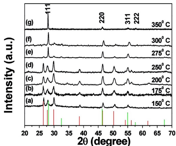
Fig. 26 XRD patterns of \text{CuInS}_2 NCs synthesised at different temperatures for TOPO:DDT = 50:50. The red and green lines at the bottom refer to the peak positions of wurtzite and zinc-blende phases, respectively (reproduced with permission from ref. 166, copyright 2009, American Chemical Society).
