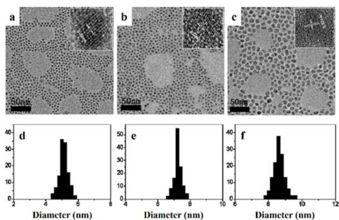
Fig. 7 TEM and high-resolution transmission electron microscopy (HRTEM) images of the as-prepared ZnSe NCs synthesised at 300 °C with different amount of OA as the capping ligands. The average particle size is (a) 5.0 nm, (b) 7.2 nm, and (c) 8.4 nm. (d-f) are the corresponding size-distribution histograms obtained from (a-c), respectively (reproduced with permission from ref. 84, copyright 2010, Royal Society of Chemistry).
