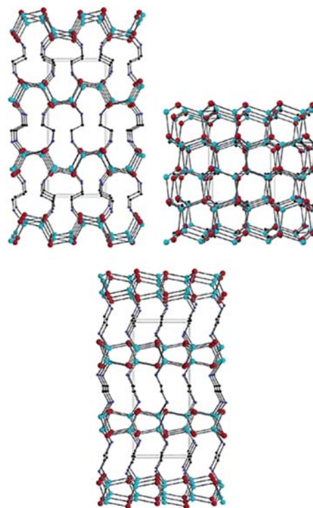
Fig. 21 Structural view of \text{CdSe-0.5en} down the b (top, left), c (top, right) and a (bottom) axes of the orthorhombic cell. Red, cyan, blue, and black balls stand for Cd, Se, N, and C atoms, respectively. H atoms are omitted for clarity (reproduced with permission from ref. 153, copyright 2003, American Chemical Society).
