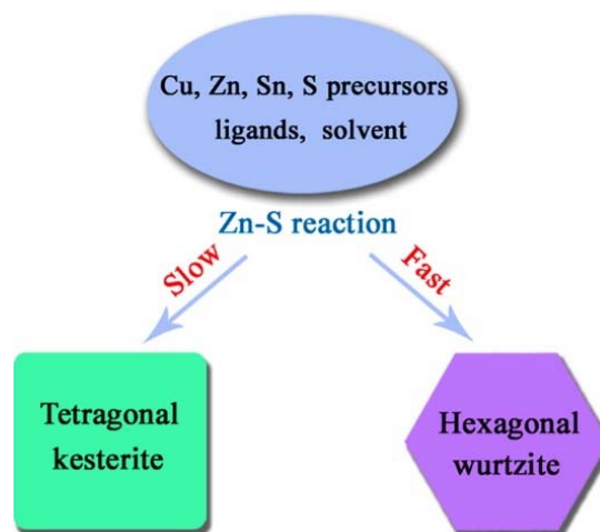
Fig. 28 Schematic diagram of the proposed mechanism of phase-controlled synthesis of \text{Cu}_2\text{ZnSnS}_4 NCs. The crystalline phase was determined by the reactivity between Zn and S, where a preference for Zn-S reaction over Sn-S reaction favours the formation of a metastable hexagonal wurtzite structure (reproduced with permission from ref. 171, copyright 2013, American Chemical Society).
