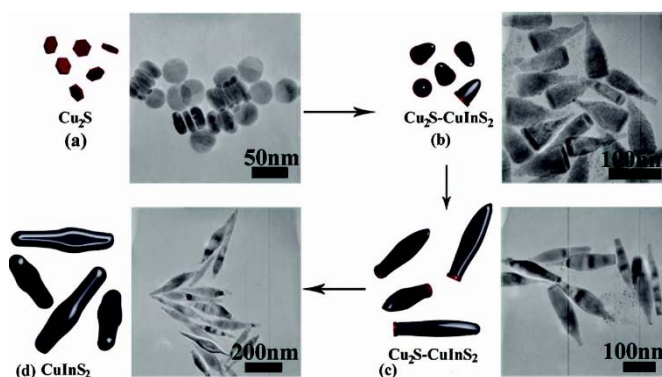
Fig. 25 Schematic of the proposed growth mechanism with corresponding TEM images: (a) formation of \text{Cu}_2\text{S} nanodisks at the initial stage, (b) epitaxial growth of \text{CuInS}_2 on \text{Cu}_2\text{S} nanodisks leads to biphasic NRs, (c) continued growth of \text{CuInS}_2 with the conversion of \text{Cu}_2\text{S} into \text{CuInS}_2 , and (d) monophasic \text{CuInS}_2 NCs (reproduced with permission from ref. 163, copyright 2009, American Chemical Society).
