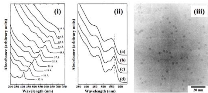
Fig. 3 (i) The optical absorption spectra of CdSe NCs dispersed in hexane with the size ranging from ~ 12 to 115 Å. (ii) The optical absorption spectra of CdSe NCs: (a) before size-selective precipitation; (b) after one cycle size-selective precipitation from the growth solution with methanol; (c) after dispersion in 1-butanol and second size-selective precipitation with methanol; (d) after a final size-selective precipitation from 1-butanol/methanol. (iii) The transmission electron microscope (TEM) image of CdSe NCs with size around 35.0 Å ± 5% (reproduced with permission from ref. 31, copyright 1993, American Chemical Society).
