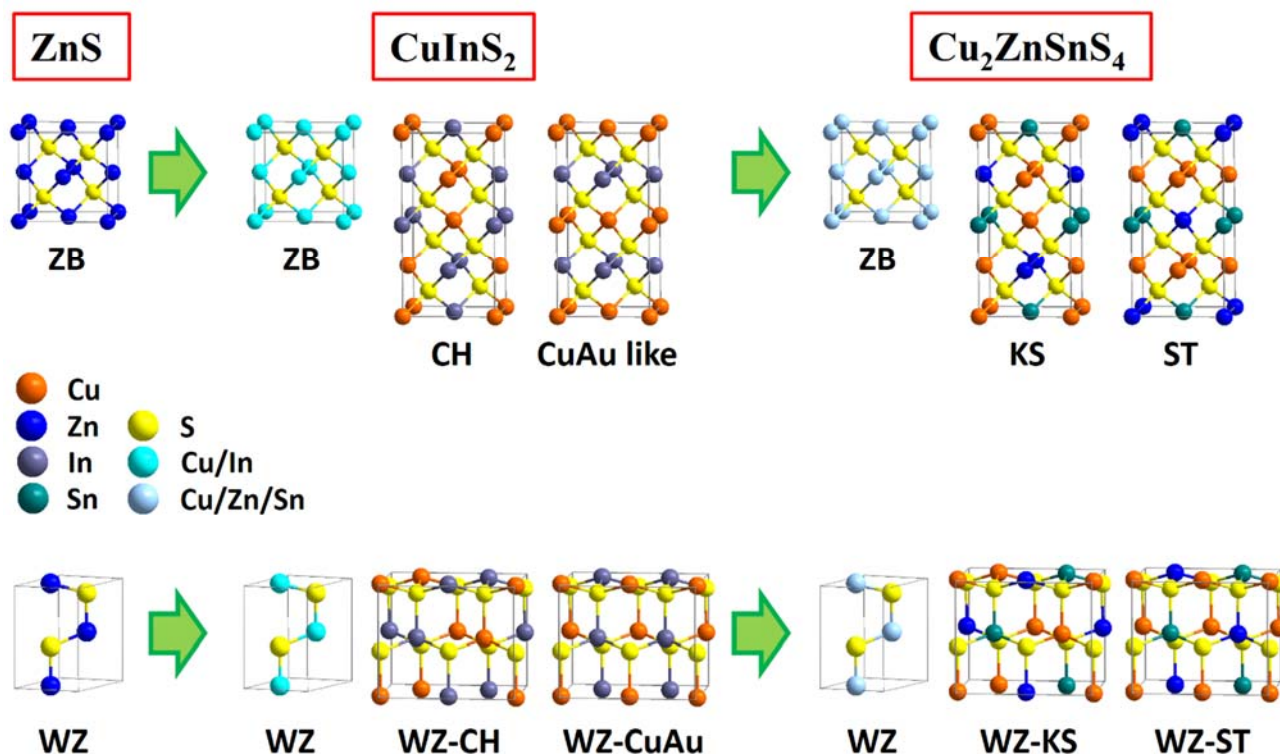
Fig. 23 Schematic diagram of the structural derivation of ternary CuInS 2 and quaternary Cu 2 ZnSnS 4 NCs from binary ZnS, which possesses the zinc-blende (ZB) and wurtzite (WZ) phases. CuInS 2 and Cu 2 ZnSnS 4 compounds also possess the basic ZB and WZ phases, while have more derived structures, such as chalcopyrite (CH), wurtzite-chalcopyrite (WZ-CH), CuAu-like, and WZ-CuAu-like for CuInS 2 ; kesterite (KS), wurtzite-kesterite (WZ-KS), stannite, and wurtzite-stannite (WZ-ST) for Cu 2 ZnSnS 4 .
