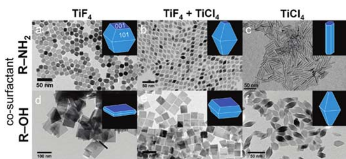
Fig. 20 TEM images of \text{TiO}_2 NCs synthesised using the precursor \text{TiF}_4 (a,d), a mixed precursor of \text{TiF}_4 and \text{TiCl}_4 (b,e), and \text{TiCl}_4 (c,f). The depicted in a-c and d-f are synthesised in the presence of OLA and 1-octadecanol (ODOL), respectively (reproduced with permission from ref. 149, copyright 2012, American Chemical Society).
