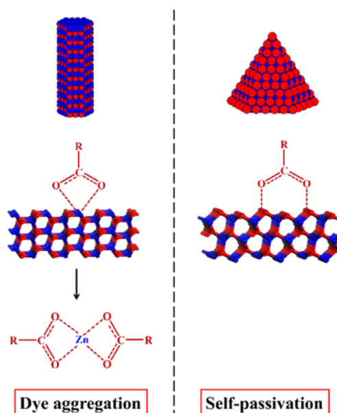
Fig. 19 Comparison of the effect of ZnO surface termination on the dye adsorption for DSSCs. Left: the \{10-10\} surface of ZnO nanorods exposed with Zn/O (50%/50%) atoms is likely to be etched by acidic dye molecules, resulting in dye aggregation. Right: the \{10-11\} surface of ZnO nanocones is terminated with 100% O atoms, leading to a durable performance in DSSCs (reproduced with permission from ref. 144, copyright 2013, American Chemical Society).
