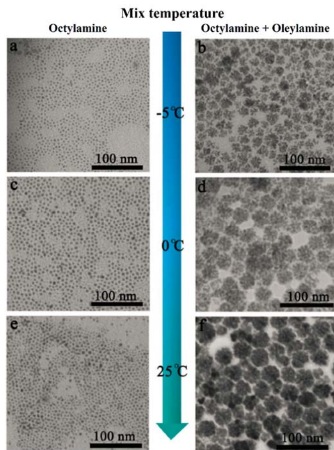
Fig. 8 TEM images of PbS NCs synthesised by non-injection method using an individual amine (left column) and mixed amines (right column) as the capping ligands at different reaction temperatures: (a,b) -5 °C; (c,d) 0 °C; and (e,f) 25 °C (reproduced with permission from ref. 82, copyright 2013, Royal Society of Chemistry).
