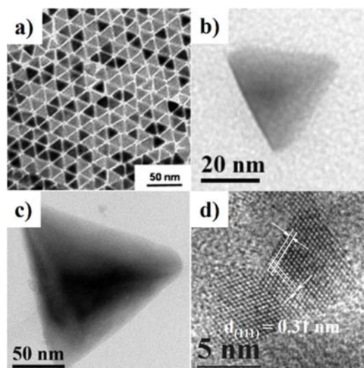
Fig. 16 TEM images of tetrahedral nanocrystals: (a) chalcopyrite CuInSe 2 NCs, (b) zinc-blende CuInS 2 NCs, (c) zinc-blende Cu 2 SnS 3 NCs, and (d) zinc-blende Cu 2 ZnSnS 4 NCs (reproduced with permission from ref. 116, copyright 2009, American Chemical Society; and ref. 140, copyright 2013, Royal Society of Chemistry).
