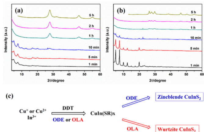
Fig. 22 (a,b) XRD patterns of CuInS 2 NCs prepared with different reaction times in ODE and OLA solvent, respectively. (c) Schematic diagram for the formation mechanism of CuInS 2 NCs using different capping ligands (reproduced with permission from ref. 140, copyright 2013, Royal Society of Chemistry).
