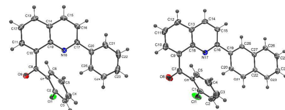
Figure 3 ORTEP diagrams (50% probability) of 4a and 4b .
