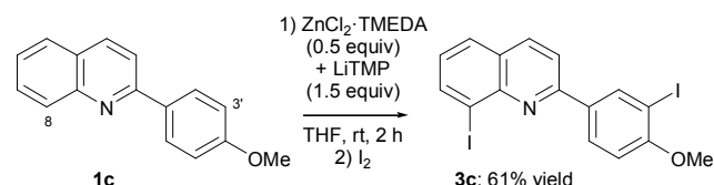
Scheme 3 Deprotonation of 1c followed by iodination.
