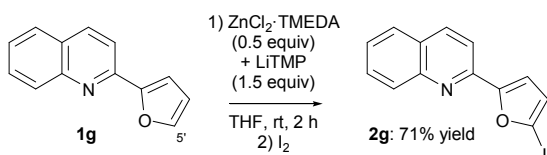
Scheme 6 Deproto-metallation of 1g followed by iodination.
