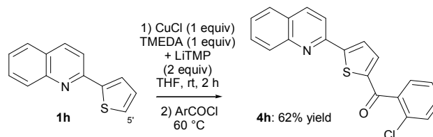
Scheme 9 Deproto-metallation of 1h followed by aroylation.
