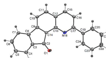
Figure 4 ORTEP diagrams (50% probability) of 5a .
