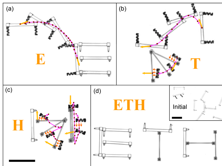
Figure 4. Several different contact and non-contact manipulation strategies were combined in a single experimental demonstration. (a)-(d) ‘ETH’ logo assembled using cooperation of multiple microcarriers. The purple lines show the trajectory and orange arrows show the direction of motion. The scale bar is 100\ \mu\text{m} .
