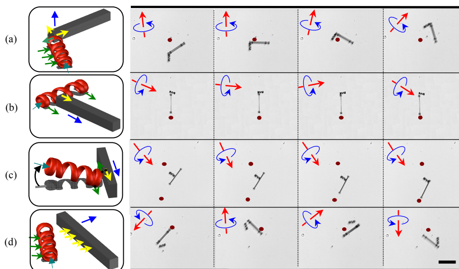
Figure 2. Schematic description and experimental demonstration of four basic ways to push a bar on the surface of the substrate (a) A microcarrier pushes one end of the bar to rotate 90 degrees using its head directly with another end of the bar as center. (b) The slight drift generates the pushing force acting on the bar. (c) The bar is conveyed by a microcarrier that was tilted 15 degrees up from the surface. (d) The bar is pushed and rotated by lateral fluid flow. The dots are reference points and the scale bar is 100 \mu\text{m} .
