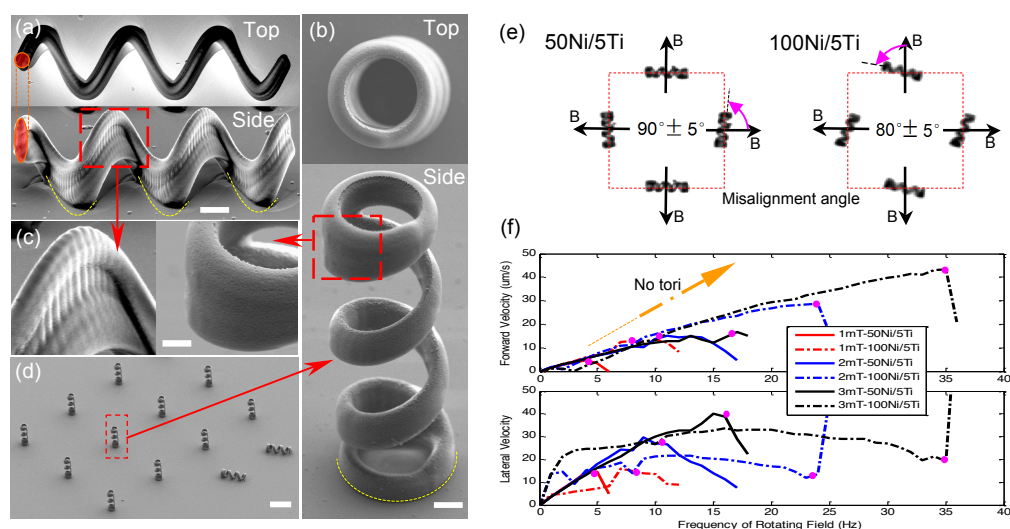
Figure 1. Fabrication of microcarriers and characterization of their swimming properties. (a) SEM images of a bare helical structure that was written horizontally using IP-L photoresist. (b) The vertically written helical microcarrier from SU-8. The scale bars are 2 \mu\text{m} . (c) Comparison of texture features of designs shown in (a) and (b). The scale bar is 1 \mu\text{m} . (d) A horizontal array of helical microcarriers. The scale bar is 20 \mu\text{m} . The alignment of magnetization angle (e) and swimming performance (f) of same-sized carriers coated with different thicknesses of magnetic material.
