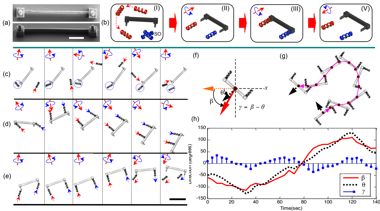
Figure 3. Cooperative manipulation using multiple microcarriers. (a) SEM image of a microbar fabricated with handles. (b) Schematic description of the cooperative manipulation strategy. (c) Snapshots from the recorded videos showing the positioning of multiple carriers around the microbar. The carrier in blue circle cannot move as the rotating frequency of the magnetic field is higher than its step out (SO) frequency. (d) Moving the microbar with two carriers without firm attachment. (e) Loading and unloading of microcarriers. (f) Steering direction of the microcarrier. The horizontal dashed line is a reference line with 0 degree. (g) The trajectory of the microcarrier transported with loaded microcarriers. The angular error between the expected and recorded orientation of the microbar remains lower than \pm 50 degrees throughout the experiment. The scale bars are 20 and 100 \mu\text{m} .
