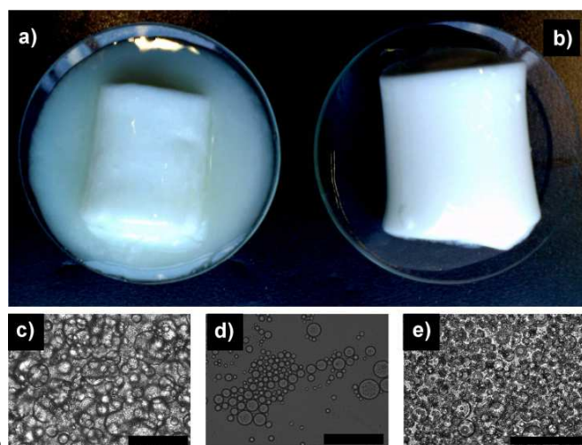
Fig. 2. a & b) Photographs of emulsion gels prepared at internal phase volumes ( \phi_{\text{water}} ) of 0.5 and 0.75 respectively; c & d) Optical microscopy image (scale bars = 25 \mu\text{m} ) of separated gel and fluid phases respectively of emulsion prepared at \phi_{\text{water}} = 0.5 . Notice the microstructure difference of the two phase; e) Optical microscopy image (scale bar = 25 \mu\text{m} ) of HIPE gel prepared at \phi_{\text{water}} = 0.75 .
