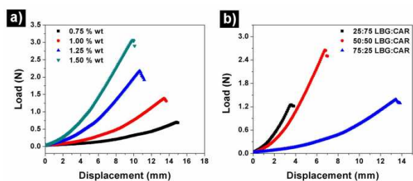
Fig. 4. Load-displacement curves for HIPE gels made with LBG:CAR at a) different total polymer concentrations while keeping the LBG:CAR proportion at 75:25 and b) different ratios of LBG:CAR at a total polymer concentration of 1 %wt. PGPR was used as an emulsifier in this emulsions at concentration of 0.4 %wt.
