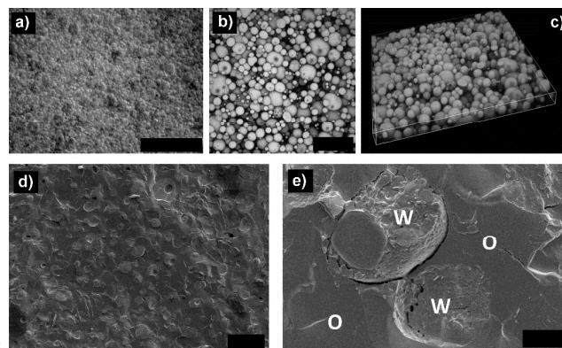
Fig. 3. a & b) Optical and confocal microscopy images of HIPE gel prepared at \phi_{\text{water}} = 0.75 (scale bars = 100 & 20 \mu\text{m} respectively); c) 3D volume view created using stacked images obtained from confocal microscopy (sample depth = 15 \mu\text{m} ); d) Cryo-SEM image of freeze fractured HIPE gel showing gelled droplets in an oil continuous phase (scale bar = 10 \mu\text{m} ); e) The fractured gelled water droplet (scale bar = 2 \mu\text{m} ), water (W) and oil (O) phase are marked for better clarity. The HIPE gel was prepared using 0.4%wt of emulsifier (PGPR) and a total polymer concentration of 1 %wt (containing LBG:CAR in 75:25 ratio).
