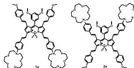
Scheme 2. Computational models.
