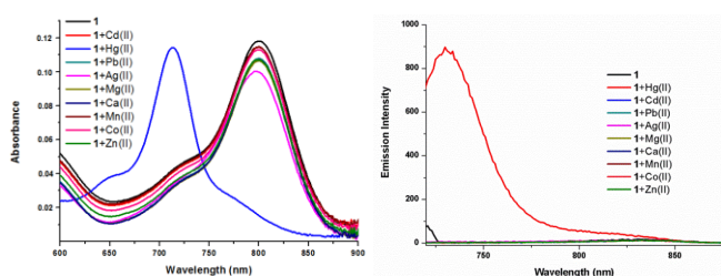
Fig. 1. Electronic absorption and emission spectra of 1 (0.5 \mu\text{M} ) in THF in absence and presence of various metal ions. Added metal ion concentrations were 5 \mu\text{M} . Excitation wavelength was 710 nm.
