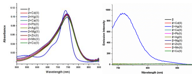
Fig. 2. Electronic absorption and emission spectra of 2 (1.0 \mu\text{M} ) in THF in absence and presence of various metal ions. Added metal ion concentrations were 10 \mu\text{M} . Excitation wavelength is 725 nm.
