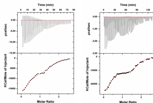
Fig. 3. Calorimetric binding isotherm for the compound 3 (right, 0.4 mM 3 titrated with 5 mM \text{Hg}(\text{ClO}_4)_2 ) and 4 (left, 0.14 mM 4 titrated with 2 mM \text{Hg}(\text{ClO}_4)_2 ) in acetonitrile.
