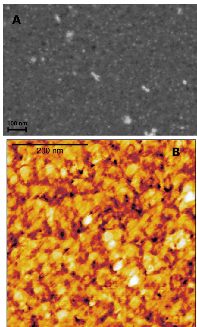
Fig. 6 A) Backscattered (BS) SEM micrograph the graphite-Pt-nanocomposite film (the bright spots denote chemical (z-number) contrast of the Pt-NPs); B) is the AFM-phase image showing the distribution of Pt-NPs (black spots).
