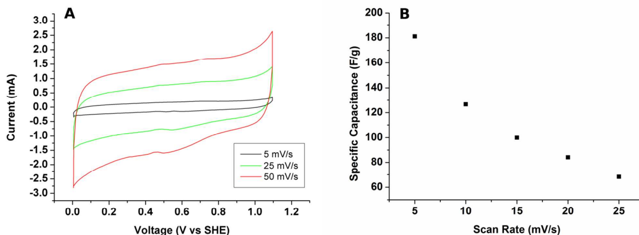
Fig. 7 A) Current vs voltage (CV) curves of the graphite films in a 0.5M H 2 SO 4 electrolyte for 3 different voltage scans; B) Plot of the specific capacitance as a function of the scan rate.
