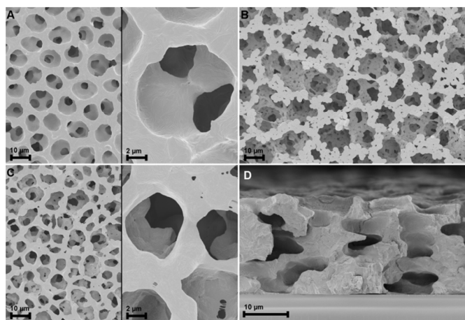
Fig. 1 Secondary electron (SE) micrographs of porous PVDF-films. (A) dual magnification SE micrographs of a PVDF-TrFE copolymer film showing ordered, hierarchical porosity; notice that the pore walls are rather smooth. (B) A PVDF film that was processed using a high oxidant concentration and displaying larger pores. (C) A PVDF film that was processed with a smaller oxidant concentration than above; the pores become smaller and ordering increases. (D) Is a cross section SE micrograph of a PVDF-TrFE film to demonstrate pore connectivity.
