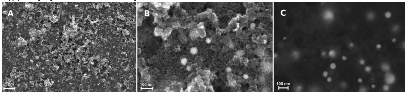
Fig. 5 SEM micrographs of the graphite-Ag-nanocomposite film: A) at low magnification showing overall film morphology (the bright spots are Ag-NPs); B) at higher magnification; C) is a BS SEM micrograph of B) displaying the morphology of the Ag-NPs (some of them are beneath the surface, hence the diffuse contrast). This journal is © The Royal Society of Chemistry 2012
