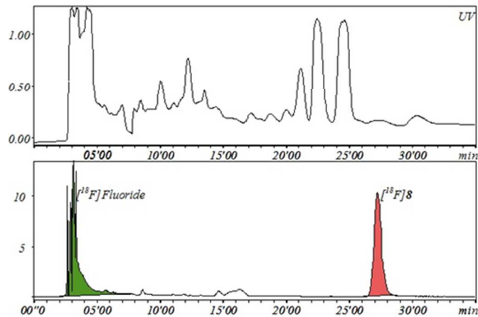
Figure 3: Radiochromatogram of the separation of [^{18}\text{F}]\mathbf{8} by semi-preparative HPLC. (60:40 acetonitrile/buffer: 1 % aqueous TEA/ \text{H}_3\text{PO}_4 , pH 8.0-8.5; Luna PFP(2); 4 ml/min).
