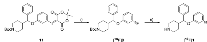
Scheme 4: Radiosynthesis of 3- ^{18}\text{F} FPPMP ( ^{18}\text{F} 1 ). i) n.c.a. ^{18}\text{F} fluoride, Kryptofix ® 2.2.2., \text{K}_2\text{CO}_3 , acetonitrile, 120 ^\circ\text{C} ; ii) \text{CF}_3\text{CO}_2\text{H} , DCM.
