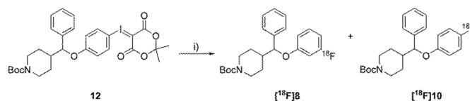
Scheme 5: Formation of regioisomers in the synthesis of 4- [^{18}\text{F}]\mathbf{10} . i) n.c.a. [^{18}\text{F}]\text{fluoride} , Kryptofix ® 2.2.2., \text{K}_2\text{CO}_3 , acetonitrile, 130 °C
