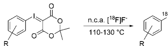
Scheme 1: Nucleophilic n.c.a. ^{18}\text{F} -fluorination of arenes using iodonium ylides.
