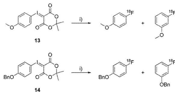
Scheme 6: Formation of regioisomers in the reaction of ylides \mathbf{13} and \mathbf{14} with n.c.a. [^{18}\text{F}]\text{fluoride} . i) n.c.a. [^{18}\text{F}]\text{fluoride} , Kryptofix ® 2.2.2., \text{K}_2\text{CO}_3 , acetonitrile, 130 °C
