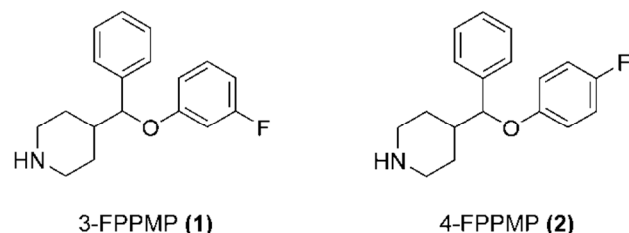
Figure 2: Molecular structures of 3-FPPMP (1) and 4-FPPMP (2), ligands for the NE- and SE-reuptake transporters, respectively.
