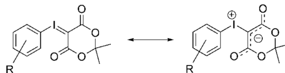
Figure 1: Resonance structures of aryl-iodonium ylides.
