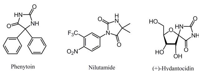
Figure 2: Biologically-active hydantoin compounds
