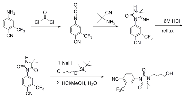
Figure 4: Traditional Synthesis of RU58841
