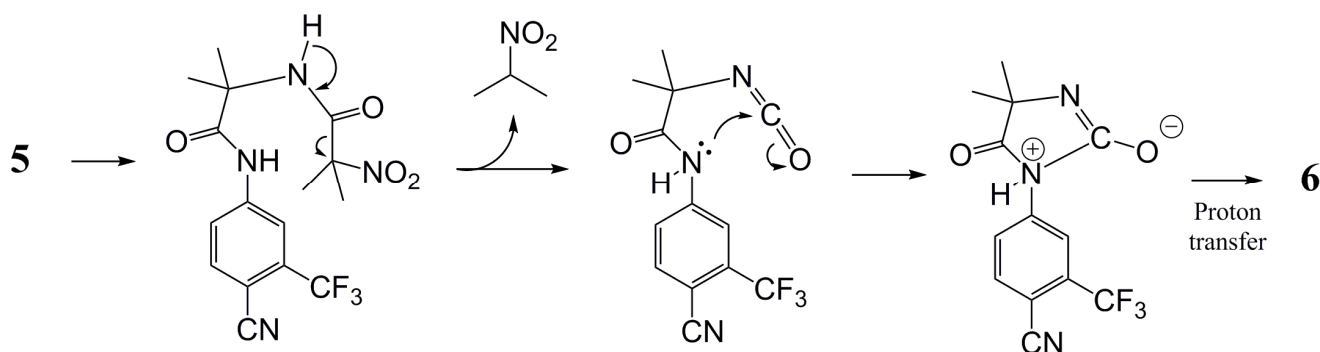
Figure 6: Probable mechanism for hydantoin formation
