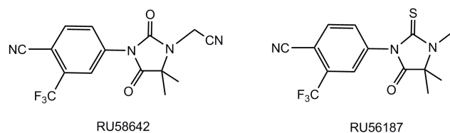
Figure 3: RU58642 and RU56187
