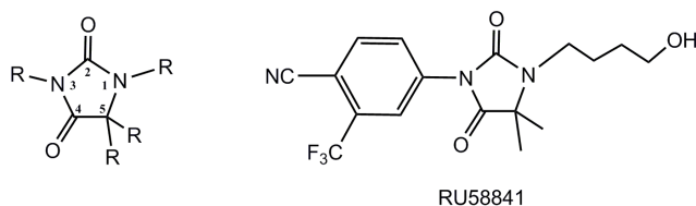
Figure 1: Hydantoin group and RU58841 anti-baldness compound
