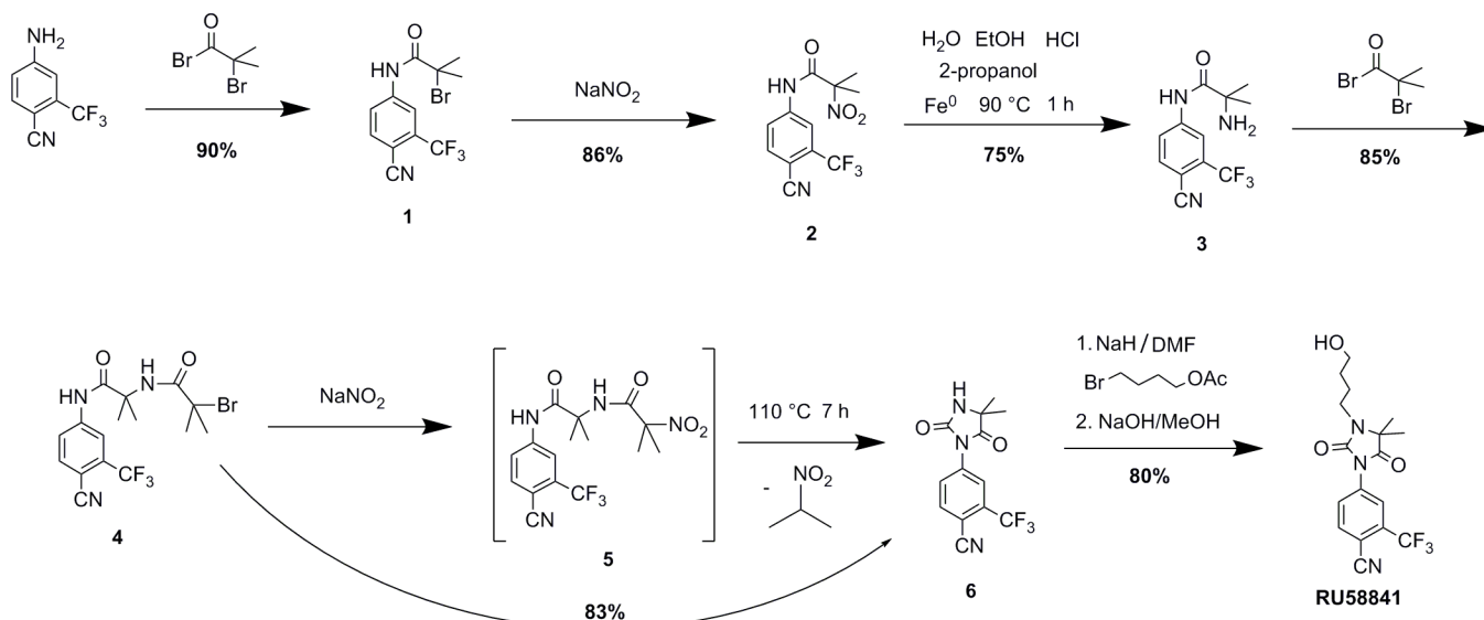
Figure 5: Alternative synthesis of RU58841
