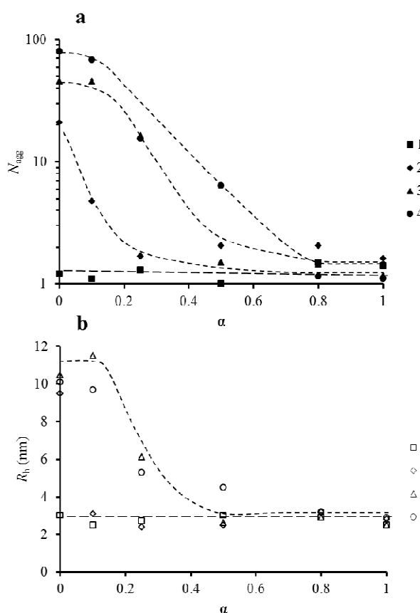
Fig. 3 a) Evolutions of N_{agg} with \alpha for polymers 1 , 2 , 3 and 4 . b) Evolutions of R_h with \alpha for polymers 1 , 2 , 3 and 4 . Values of N_{agg} and R_h given are then obtained extrapolation to zero concentration. Lines are included as a guide for the reader.
