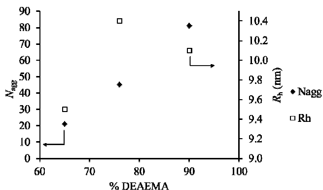
Fig. 5 Effect of the DEAEMA loading on the N_{\text{agg}} and R_h for polymers 2, 3 and 4 at \alpha = 0 . Values of N_{\text{agg}} and R_h given are then obtained extrapolation to zero concentration.
