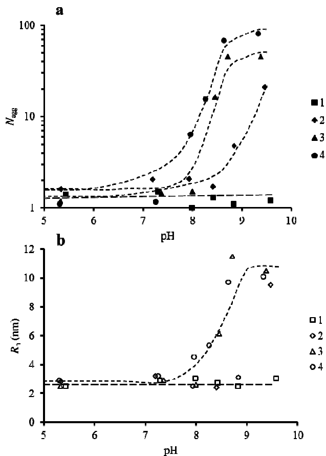
Fig. 4 a) Evolutions of N_{agg} with pH for polymers 1 , 2 , 3 and 4 . b) Evolutions of R_h with pH for polymers 1 , 2 , 3 and 4 . Values of N_{agg} and R_h given are then obtained extrapolation to zero concentration. Lines are included as a guide for the reader.
