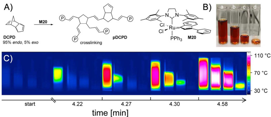
Fig 2 ROMP of dicyclopentadiene initiated with M20 (A), photograph of reaction vessels ((a) 3.7, (b) 2.6, (c) 1.2 and (d) 0.5 mL) containing the formulation for ROMP (B) and thermal images showing the heat evolution during polymerisation depending on the volume (C)
