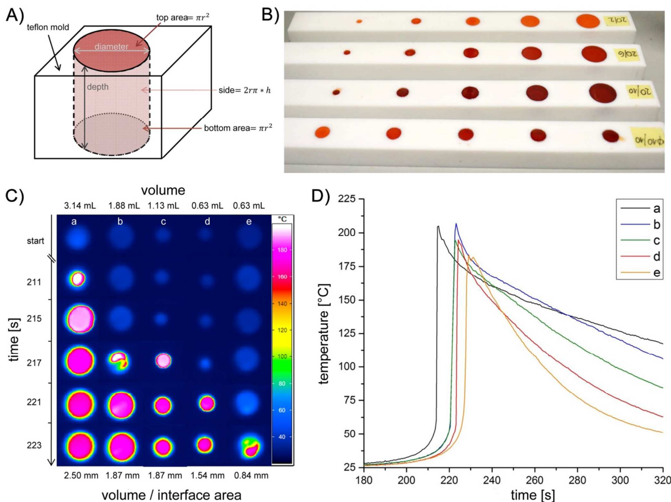
Fig 3 General shape of the reaction chambers (A), photograph of the reaction chambers made in Teflon (B), thermal image showing the heat evolution during ROMP in dependence of the dimensions of the reaction chambers (cf. Table 1) (C) and time/temperature profiles of the reaction chambers a-e (D).
