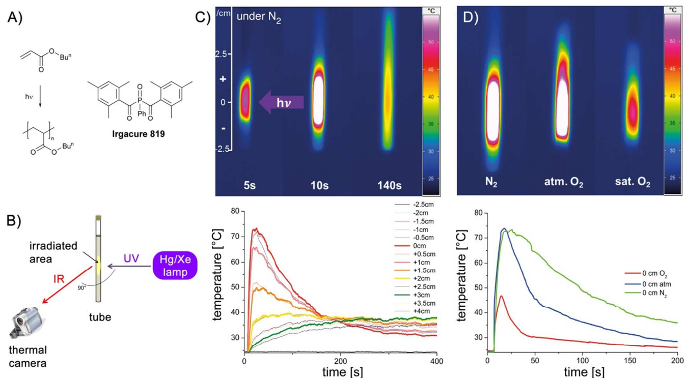
Fig.1 Polymerisation under investigation (A), experimental setup for the recording of thermal images (B), thermal images of formulations irradiated for 10 s at 5, 10, and 140 s after irradiation was stopped (under N_2 ) (C, above) and time/temperature profiles for the same experiment at selected distances from the position of irradiation (C, below) as well as thermal images of samples at different oxygen concentrations recorded 10 s after irradiation was stopped (D, above) and time/temperature profiles at the centre of irradiation of these samples (D, below).
