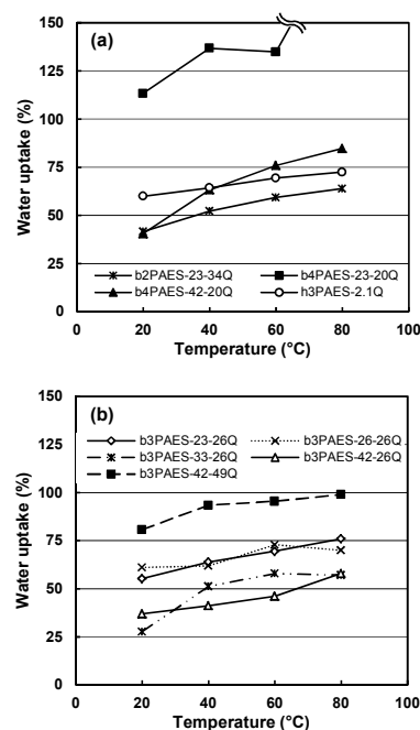
Figure 6. Water uptake data of the b2PAES- n -mQ, b4PAES- n -mQ (a), and the b3PAES- n -mQ (b) AEMs in the Br - form as a function of temperature under fully hydrated (immersed) conditions. The data is provided in two plots for clarity.
