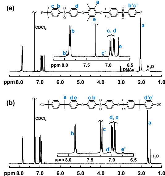
Figure 1. Representative ^1H NMR spectra of the PAES precursor blocks: fluorine terminated ol-26-F3 (a), and phenolate terminated ol-23-OH (b).
