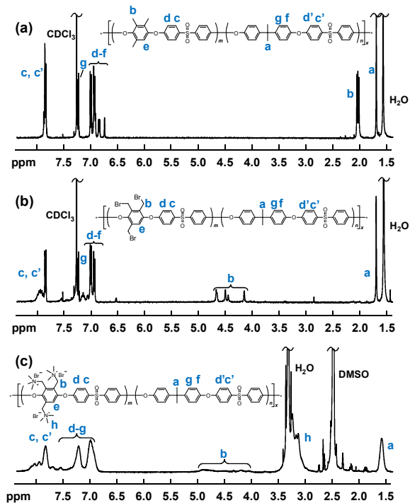
Figure 2. Representative 1 H NMR spectra of multiblock copolymers before modification, (a) b3PAES-26-26, after benzylic bromination, (b) b3PAES-26-26Br, and after quaternization, (c) b3PAES-26-26Q.
