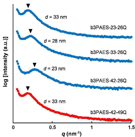
Figure 3 SAXS data of nominally dry multiblock copolymer membranes. The data have been shifted vertically for clarity and the arrowheads indicate q_{\max} .
