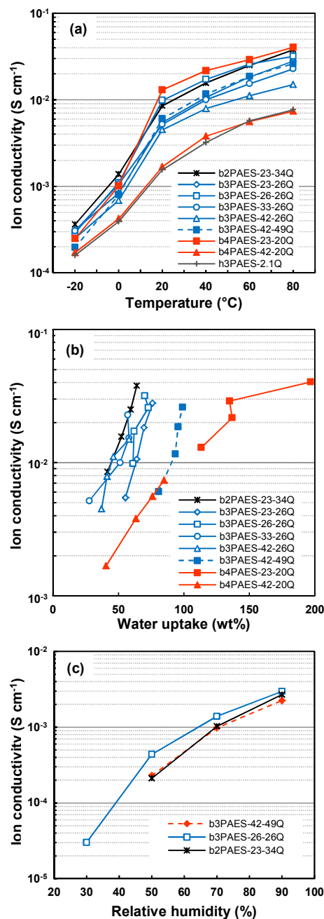
Figure 7. Br - conductivity of the AEMs in the fully hydrated (immersed) state as a function of temperature (a), as a function of water uptake in the temperature range 20–80 °C (b), and as a function of relative humidity at 80 °C (c).
