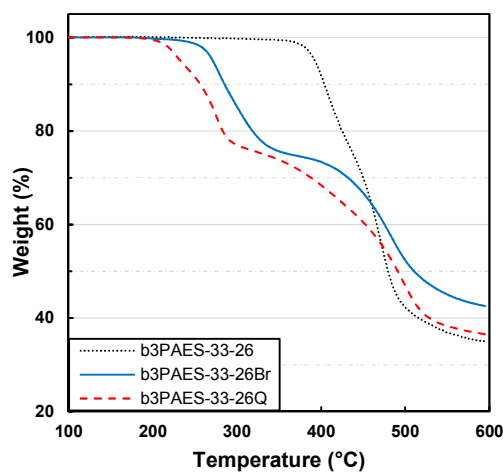
Figure 5 TGA traces of b3PAES-33-26 in the unmodified, benzylbrominated and quaternized form.
