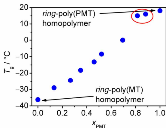
Figure 3 Glass transition temperature T_g versus the molar amount X_{PMT} of PMT in ring-poly (PMT- block -MT) polymer. The regime of sufficient mechanical stability of the (AB) n -multiblock-copolymer at room temperature showing absence of rigid fracture is marked by a red circle.
