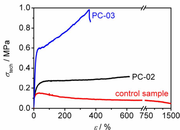
Figure 7 Stress-strain curves of polycyclic samples PC-02 and PC-03 and non-functionalized ring polymer \zeta . For reasons of clarity only one curve per material is plotted.
