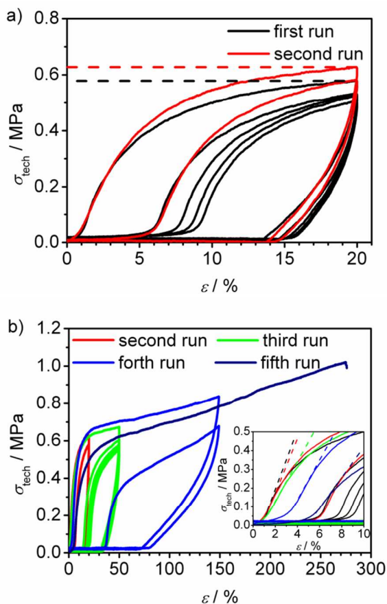
Figure 9 Cyclic stress-strain curves of a) polycyclic sample PC-03 before (black curve) and after (red curve) first thermal regeneration (first and second run) and b) second to fifth run. Note that between each run the specimen was thermally regenerated. The dashed lines in a) indicate the stress applied at 20 % elongation in the first run ( \sigma_{20\%}^0 ) and in the second run ( \sigma_{20\%} ). The small inset diagram in b) is a zoomed view of the initial stress-strain-region and shows the shift of the curves after each regeneration.
