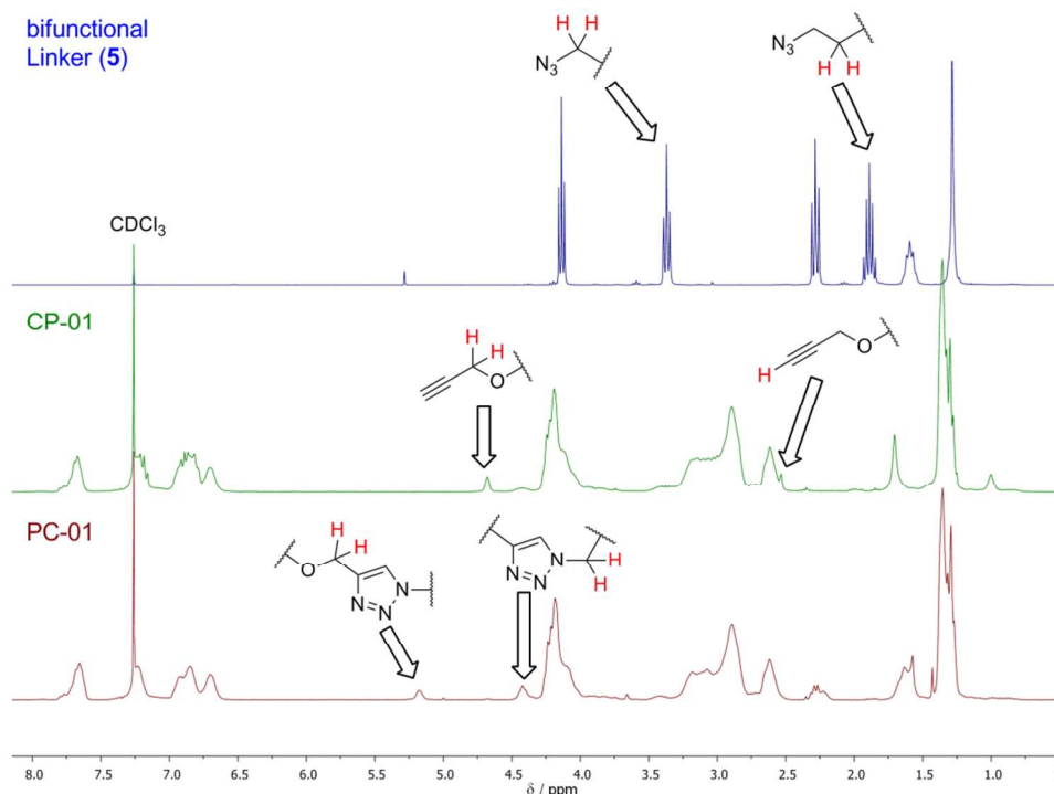
Figure 5 ^1\text{H-NMR} -spectra of the bifunctional linker (dark blue), precursor polymer CP-01 (green) and the polyaddition product of both, PC-01 (maroon). The prominent protons indicating the presence of alkyne- (4.68 and 2.53 ppm) and azide groups (3.37 and 1.89 ppm) marked in the reactants disappear or shift to 5.18 and 4.45 ppm, respectively, in the resulting polyadduct PC-01, clearly indicating the formation of a triazole ring.
