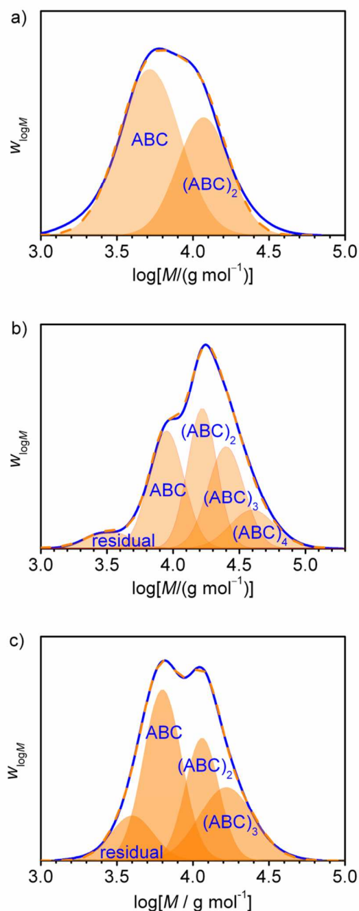
Figure 4 Molar mass distributions (SEC distributions) of samples (a) CP-01, (b) CP-02, and (c) CP-03, which were fitted by several Gaussian functions (orange filled curves) that estimated the individual multiples (ABC)_n of the ring merging reaction and residual polymer from the previous polymerization step. Original data: blue curves, sum of Gaussian fits: orange dashed curves.
