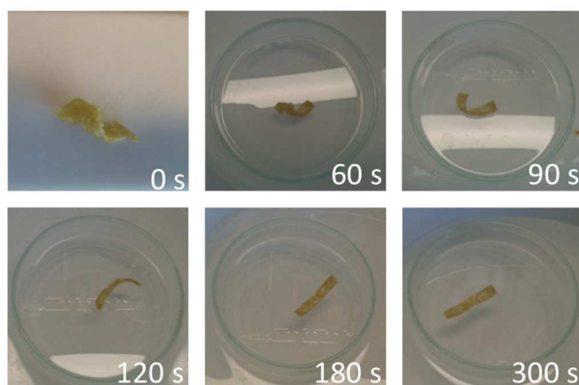
Figure 10 Series of pictures showing the shape regeneration of a twisted specimen of sample PC-03. The sample was put in a petri-dish and heated to 40 °C in a water bath.
