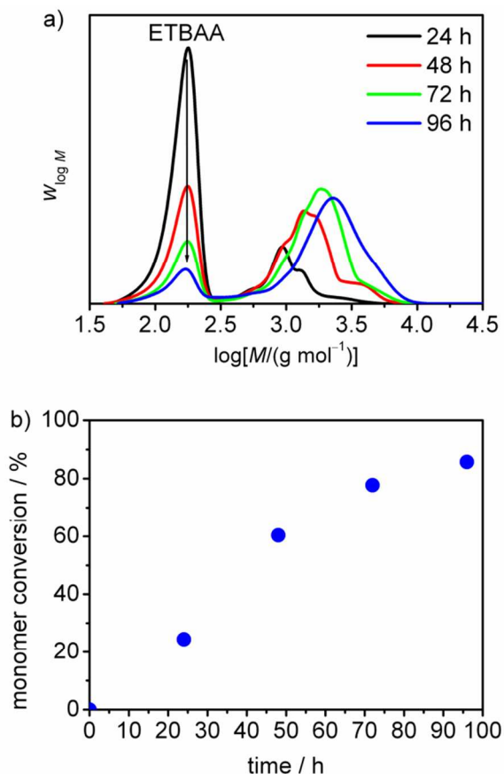
Figure 2 a) Molar mass distribution (SEC-distribution) after various times and b) monomer conversion vs. time in the ring expansion polymerization of ETBAA with PTZDA as the initiator in solution of NMP at 70 °C. Conditions: ETBAA/PTZDA=5:1, c_{\text{ETBAA}}=0.5 \text{ mol L}^{-1} , c_{\text{TBAAC}}=10 \text{ mol}\% .
