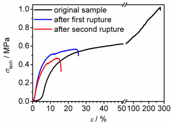
Figure 12 Stress-strain curves of PC-03 before rupture (black curve, 5th run of cyclic tensile testing described above) and after 1 st and 2 nd rupture including subsequent healing (blue and red curves).
