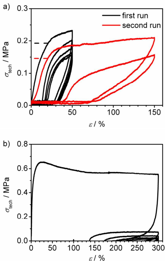
Figure 8 Cyclic stress-strain curves of a) polycyclic sample PC-02 before (black curve) and after (red curve) thermal regeneration and b) precursor polymer CP-02. 1 min pause between runs. The dashed lines in a) display the amount of stress applied at 20 % strain in the first run ( \sigma_{20\%}^0 ) and in the second run ( \sigma_{20\%} ).
