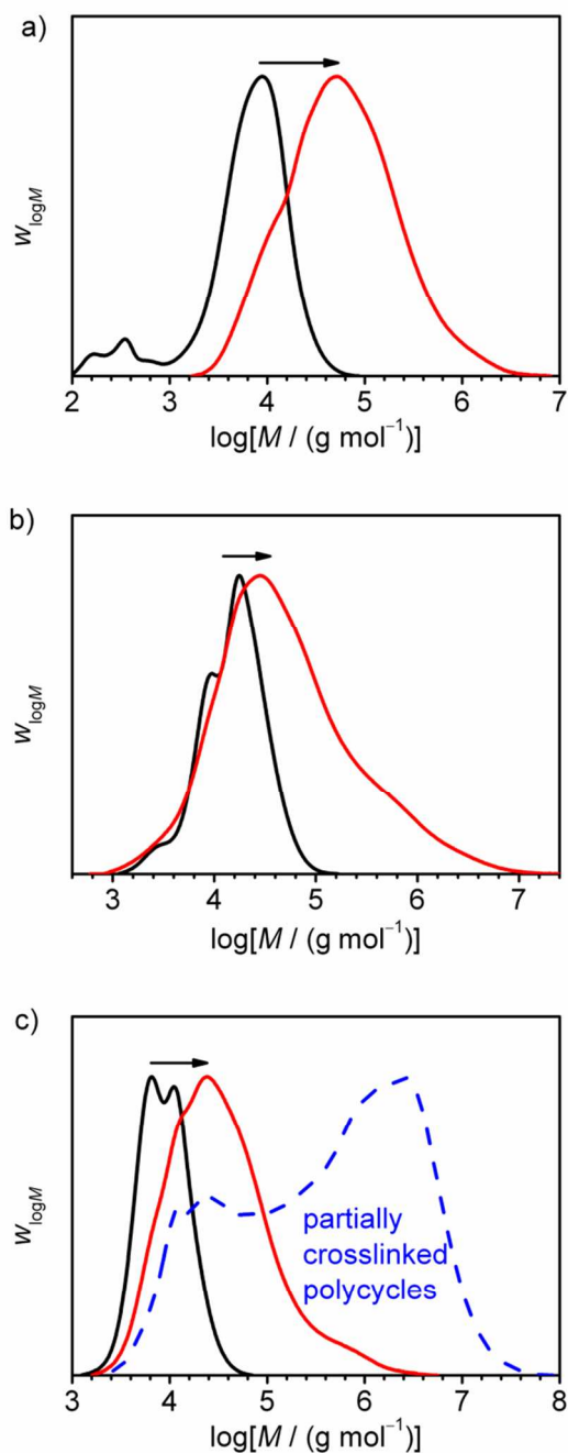
Figure 6 Evolution of molar mass distributions (SEC traces) during the polyaddition reactions of a) CP-01, b) CP-02, and c) CP-03 (black curves) with the bifunctional linker. The polyaddition products a) PC-01 and b) PC-02 are shown after precipitation from diethyl ether and drying (red curves). The molar mass distribution of c) PC-03 was recorded after dissolution of the precipitated material in THF before the drying process (red curve) and after ultrasonic treatment of the re-dissolved material which became insoluble after drying (blue dashed curve), see text for further information.
