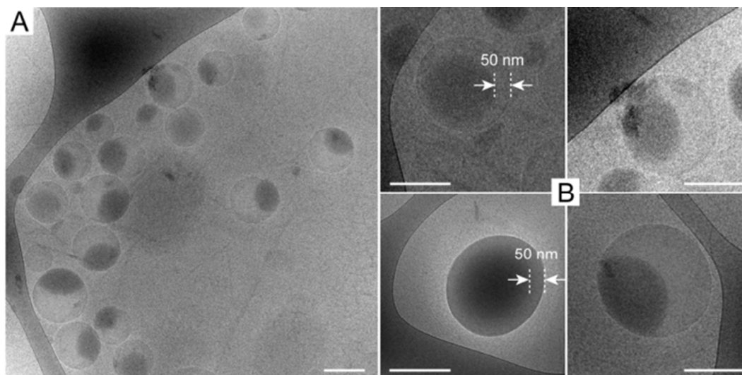
Figure 2. Cryo-TEM images of cross-linked polymeric vesicles without staining. The scale bar represents 200 nm.
