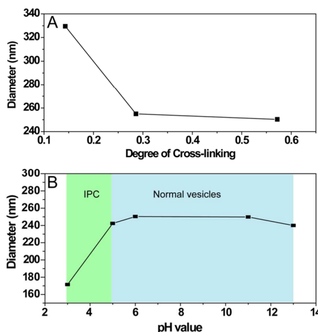
Figure 3. Hydrodynamic diameters measured by DLS as a function of (A) degree of cross-linking (DOC) and (B) pH values.
