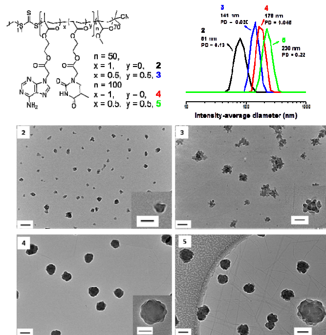
Fig. 2 Representative TEM images of self-assemblies prepared by RAFT dispersion polymerization in \text{CHCl}_3 , their corresponding polymer structures and DLS particle size distributions of 2 , 3 , 4 and 5 . Scale bar 100 nm (inset 50 nm).
