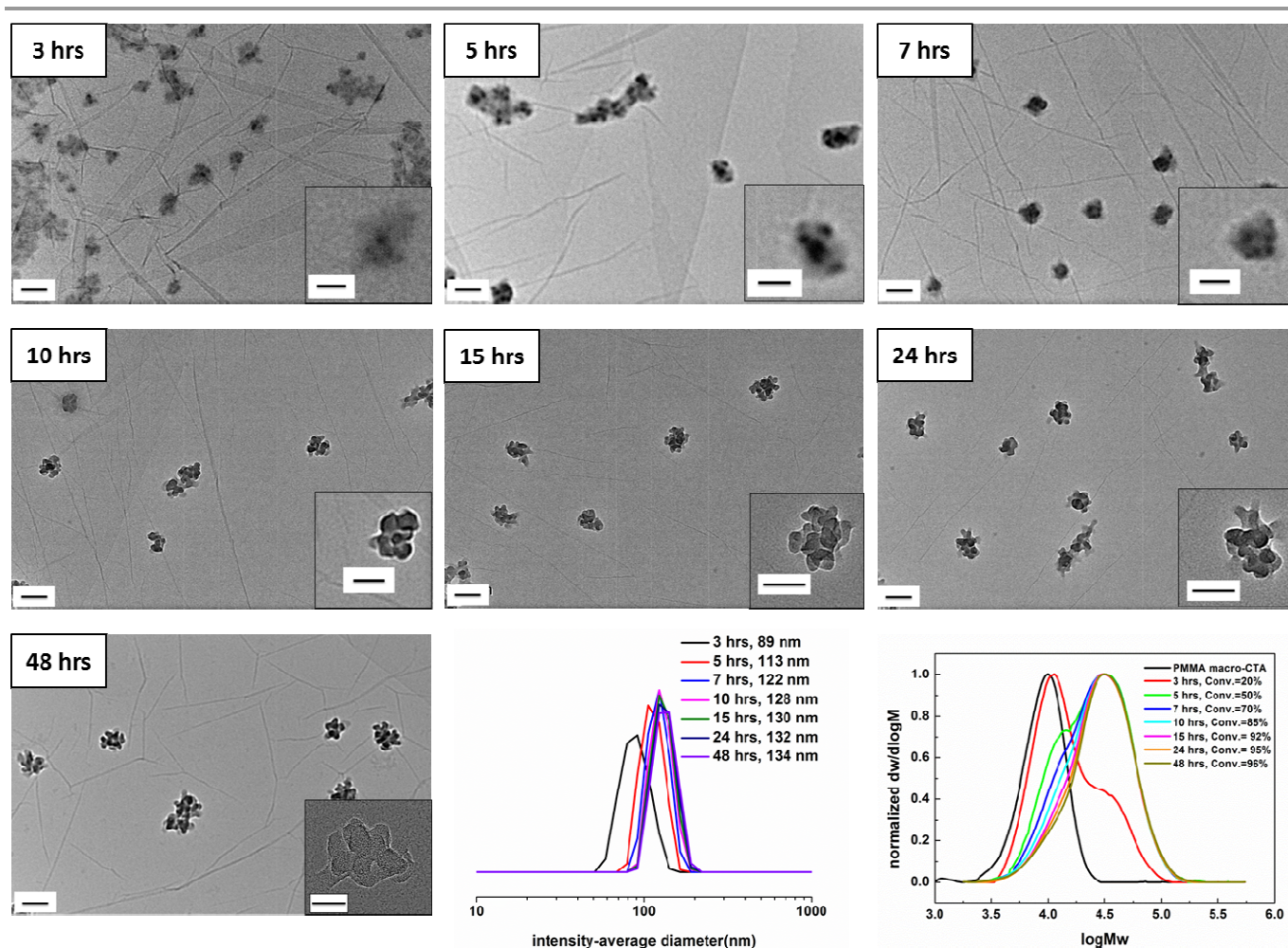
Fig. 1 Evolution of the self-assembly by unstained TEM analysis, intensity-average diameter as determined by DLS and SEC traces (DMF as eluent, PMMA standard) with monomer conversion using a PMMA 70 macro-CTA for the RAFT dispersion polymerization of a mixture of AMA and TMA in \text{CHCl}_3 at 60 °C. The target diblock composition was PMMA 70 - b -(PAMA 0.5 - co -PTMA 0.5 ) 50 , 3 . Scale bar: 100 nm (inset: 50 nm). The inset image of 48 hours was taken by TEM at a higher magnification (150 k).
