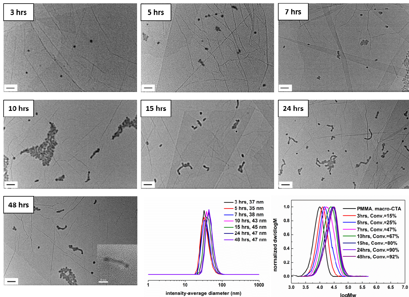
Fig. 3 Evolution of the self-assembly by unstained TEM analysis, intensity-average diameter as determined by DLS and SEC traces (DMF as eluent, PMMA standard) with monomer conversion using a PMMA 70 macro-CTA for the RAFT dispersion polymerization of a mixture of AMA and TMA in 1,4-dioxane at 60 °C. The target diblock composition was polymer 7 , PMMA 70 - b -(PAMA- co -PTMA) 50 . Scale bar: 100 nm. The inset image of 48 hours was taken by TEM at a higher magnification (60x).
