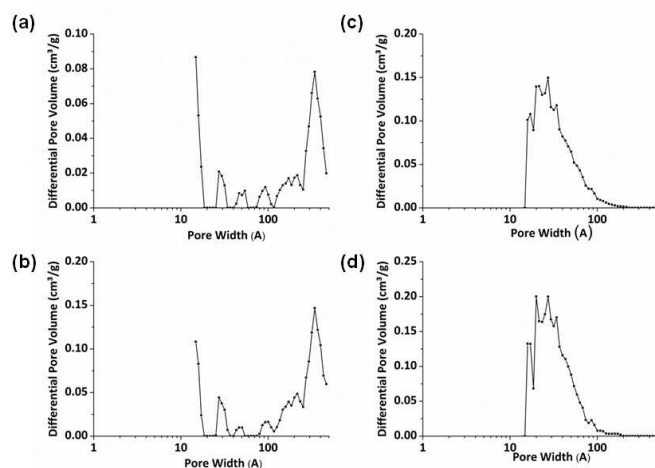
Fig. 5 NL-DFT pore size distributions of CMP-1 intermediates synthesised at varying reaction times: a) 60 min, b) 120 min, c) 300 min, d) 1080 min. The NL-DFT model for slit pores was used in the calculations.
