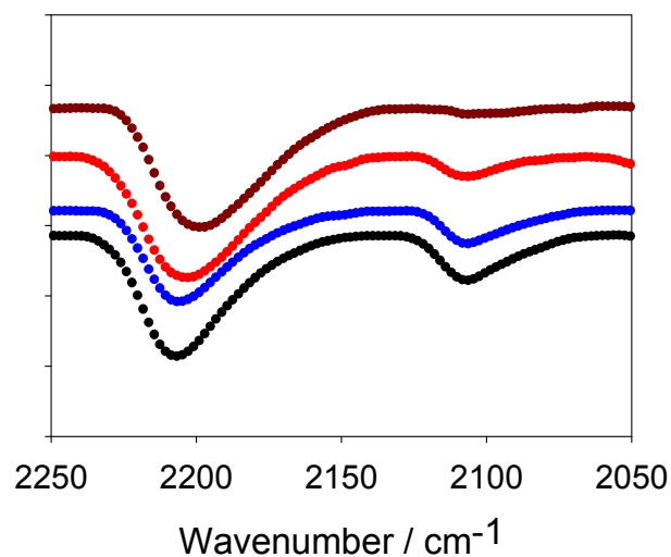
Fig. 1. FTIR spectra of CMP-1 at different reaction times (black data = 40 mins; blue = 60 mins, red = 120 mins and brown = 1080 mins) showing consumption of terminal alkyne groups (peak at 2100 cm -1 ). Data are offset on the y-axis for clarity.
