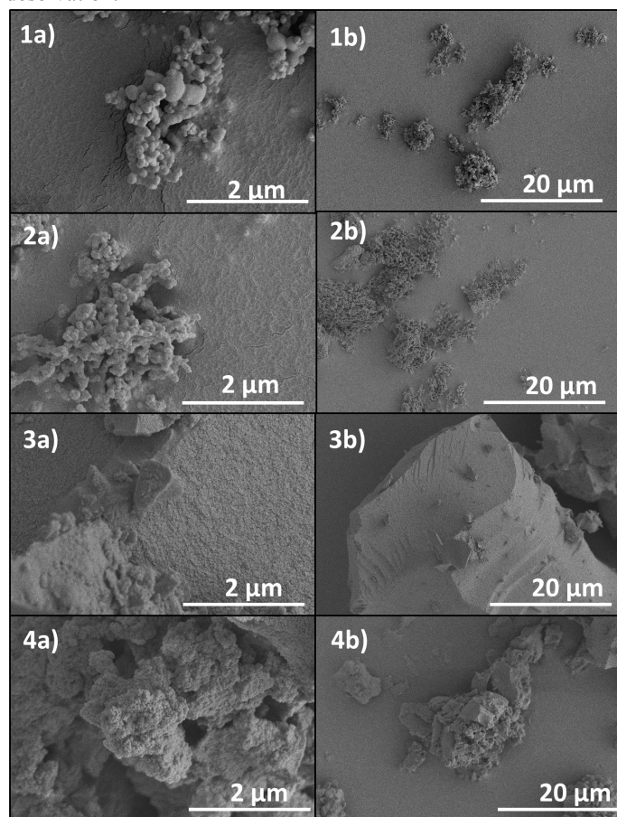
Fig. 6 SEM images of CMP-1 materials collected at reaction times of: 1) 60 min, 2) 120 min, 3) 300 min, 4) 1080 min. Scale bars are 2 \mu\text{m} (left images) and 20 \mu\text{m} (right images).
