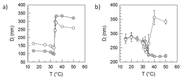
Figure 6. Correlation between D_h and temperature for a) P1-N, P2-N and b) for triblock copolymers with styrene; graph a) the grey and white symbols are P1-N and P2-N, respectively; graph b) the grey and white symbols are P1-N-S and P2-N-S, respectively.
