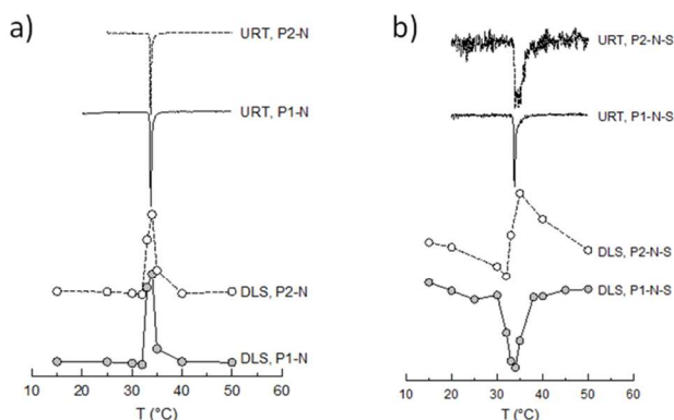
Figure 7. Correlation between the change in the temperature gradient of hydrodynamic diameter (from DLS, dD_h/dT , the two lower curves) and of the speed of sound (from URT heating, d\Delta U/dT , the two upper curves) with temperature for P1-N, P2-N diblock copolymer particles (graph a)) and P1-N-S, P2-N-S triblock copolymer particles (graph b)).
