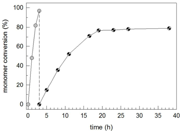
Figure 1. Monomer conversion - time curve for the synthesis of P1-N-S triblock copolymer dispersions; the grey and patterned symbols describe the NIPAM and styrene conversion, respectively.
