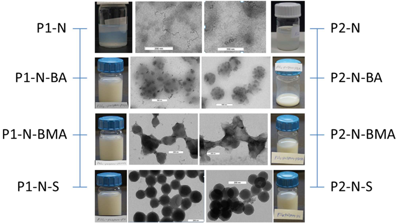
Figure 3. TEM micrographs of the diblock copolymer dispersions and the starting PIL dispersions showing the typical structures observed when the dispersions were dried on carbon-coated copper grids; the photographic snapshots arranged on the sides of the figure illustrate the dispersions as obtained after dialysis. The bar indicates 200 and 500 nm for samples P1, P2, P1-S, P2-S and P1-BA, P2-BA, P1-BMA, P2-BMA, respectively.
