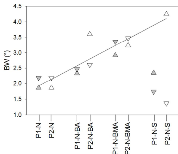
Figure 8. Width of the base of the d\Delta U/dT peaks (BW) for the various PNIPAM-containing block copolymer particles; grey and white symbols are samples prepared with crosslinked (P1) and non-crosslinked (P2) PIL, respectively, triangles up and down indicate heating and cooling cycle, respectively; the line is the linear regression of the corresponding data points (all data except for P1-N-S and cooling for P2-N-S).
