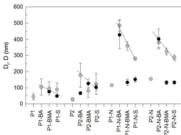
Figure 5. Comparison of hydrodynamic diameters from DLS ( D_i , grey spheres) and average diameters from TEM images ( D , black spheres) of PILs and their corresponding block copolymers latexes at room temperature; DLS measurements and preparation of TEM grids at room temperature; lines are just for guiding the eye.
