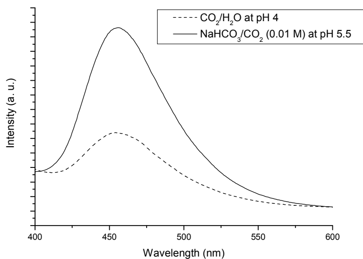
Figure 2S. Emission intensity of 7-HC measured at 455 nm obtained upon illumination (15 min) of deaerated suspensions of \text{TiO}_2 -P25 containing coumarin ( 1 \times 10^{-4} M). Compare with data of Figure 3 in the text.
