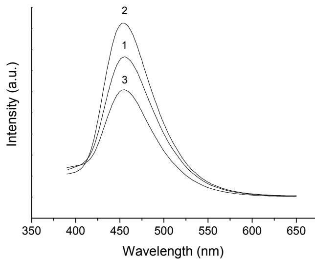
Figure 3S. Emission intensity of 7-HC measured at 455 nm obtained upon illumination (15 min) of deaerated suspensions of TiO 2 -P25 containing coumarin ( 1 \times 10^{-4} M), at pH 7.2 in the absence of NaHCO 3 (1); at pH 10 in the absence of NaHCO 3 (2); at pH 10 in the presence of NaHCO 3 /Na 2 CO 3 (3).
