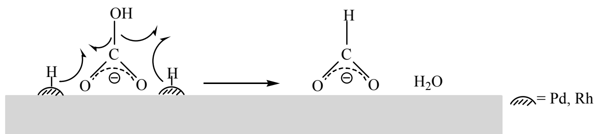
Scheme 2. Reduction of bicarbonate by hydrogen atoms formed in the discharge of \text{H}_2\text{O}/\text{H}^+ .
