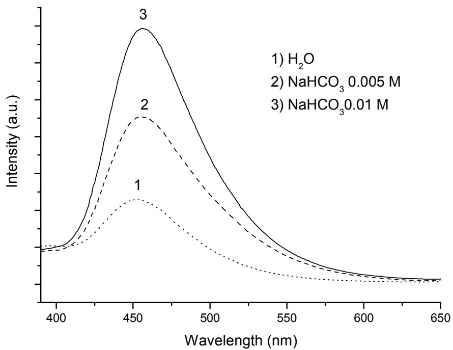
Figure 4. Emission intensity of 7-HC measured at 455 nm obtained on illumination (15 min) of deaerated aqueous suspensions of TiO 2 -P25 containing coumarin (1 × 10 -4 M).
