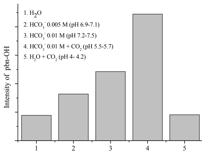
Figure 3. Comparison of the intensities of [pbn-OH]· adduct obtained upon irradiation of TiO 2 -P25 deaerated aqueous suspensions containing pbn (0.1M) with different concentrations of NaHCO 3 . Columns 4 and 5 are relative to samples deaerated with CO 2 .
