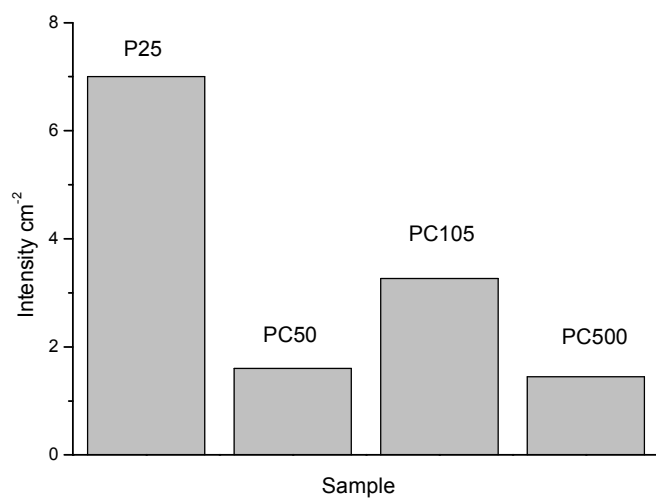
Figure 6. Intensity of the [\text{pbn-CO}_2]^\cdot adduct normalized by the area of the sample obtained on illumination (3 min) of different commercial \text{TiO}_2 powders dispersed in deaerated aqueous solutions containing \text{NaHCO}_3 (0.01M) and pbn (0.1 M), pH 7.2 \div 7.5.
