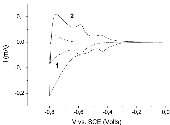
Figure 1S- Cyclic voltammetry curves for a \text{TiO}_2 (P25) in: (1) 0.01 M \text{NaHCO}_3 at pH 7.2 ; (2) 0.01 M \text{NaHCO}_3 bubbled with \text{CO}_2 until pH 5.5. Scan rate: 50 mV/s
