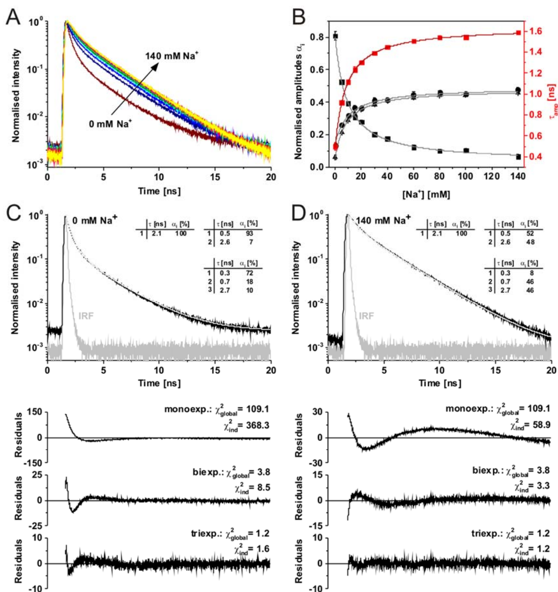
Fig. 3: In vitro calibration of ANG-2 in different Na + -buffer solutions. A Fluorescence decay curves of ANG-2 for different [Na + ]: 0, 5, 10, 15, 20, 30, 40, 60, 80, 100 and 140 mM (buffer solutions, pH 7.4; normalised at peak maximum). B Trend of normalised amplitudes ( \alpha_i ) and amplitude-weighted average fluorescence decay time ( \tau_{amp} ) for the global triexponential analysis of 55 decay curves from A ( N = 5 independent preparations) with the Na + -dependent decay time components \tau_1 = 0.3 ns (black squares), \tau_2 = 0.7 ns (black circles) and \tau_3 = 2.7 ns (black triangles), \tau_{amp} (red squares) and the K_D value of (8.3 \pm 0.4) mM calculated from the fit of \tau_{amp} using equation 3. C and D Normalised fluorescence decay curves (black) with associated triexponential fit curves (white) and generally used IRF (instrumental response function, grey) of Na + -free and Na + -saturated form of ANG-2. Mono-, bi and triexponential fit results of the global analyses were compared and shown with their corresponding amplitude components, residuals, \chi^2_{ind} and \chi^2_{global} values.
