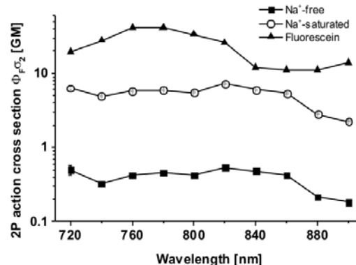
Fig. 2: 2P fluorescence excitation action cross-sections \Phi_F \sigma_2 of Na + -free and Na + -saturated ANG-2 buffer solutions ( N = 6 for each form). For the reference fluorescein (in NaOH, pH 11) literature data were used 18 ; 1 GM = 10^{-50} cm 4 s/photon; \Phi_F \sigma_2 is the product of 2P absorption cross-section \sigma_2 and fluorescence quantum yield \Phi_F .
