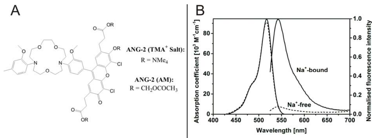
Fig. 1: A Chemical structure of ANG-2. 20 B Absorption and normalised fluorescence spectra of Na + -bound (solid lines) and Na + -free (dashed lines) form of ANG-2 with excitation wavelength \lambda_{\text{exc}} = 517 nm and c_{\text{dye}} = 1.3 \mu\text{M} .
