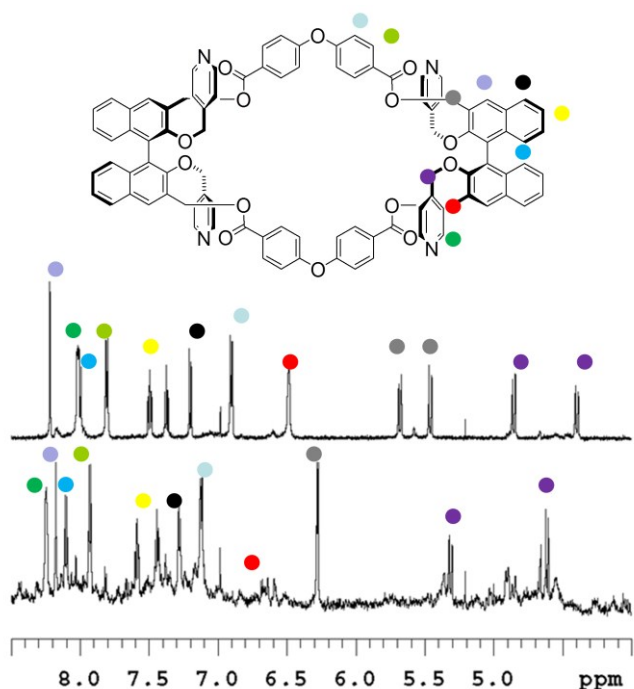
Fig. 3 ^1\text{H} NMR of in d_7 -MeCN at 25 °C top) macrocycle ( RR )-8 ( 2.8 \times 10^{-5} M, 500 MHz); bottom) same with 2 equiv. of \text{Pd}(\text{MeCN})_2\text{Cl}_2 added.
