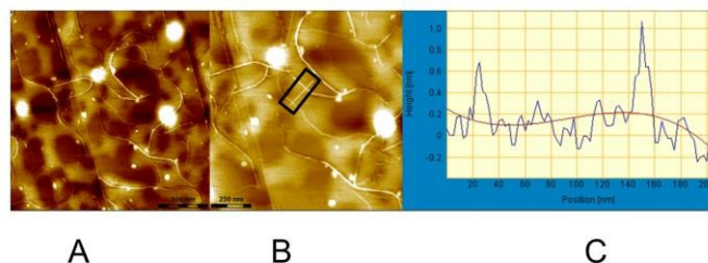
Fig. 5 AFM images of ( RR )- 8 , \text{C}_{60} and \text{PdCl}_2(\text{MeCN})_2 at the HOPG interface. (A and B) Example of fibres. (C) A height profile measured along the white line (highlighted in black box) in (B).
