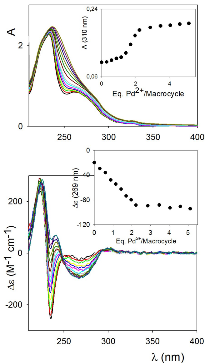
Fig. 3 ^1\text{H} NMR of in d_7 -MeCN at 25 °C top) macrocycle ( RR )-8 ( 2.8 \times 10^{-5} M, 500 MHz); bottom) same with 2 equiv. of \text{Pd}(\text{MeCN})_2\text{Cl}_2 added.
