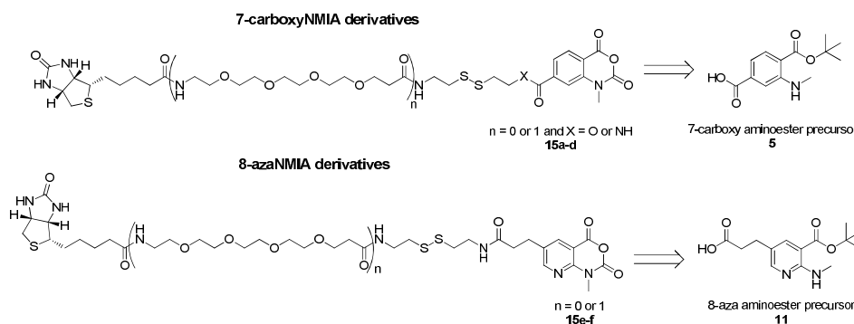
Fig. 3 7-carboxy and 8-azaisatoic anhydride derivatives 15a-f functionalized for RNA selective extraction.
