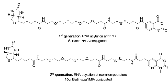
Fig. 1 Biotin-isatoic anhydride conjugated designed for RNA selective extraction.
